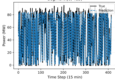
RF-WPF vs True (Wind farm site 6 (Nominal capacity-96MW)) Segment [0, 415)
