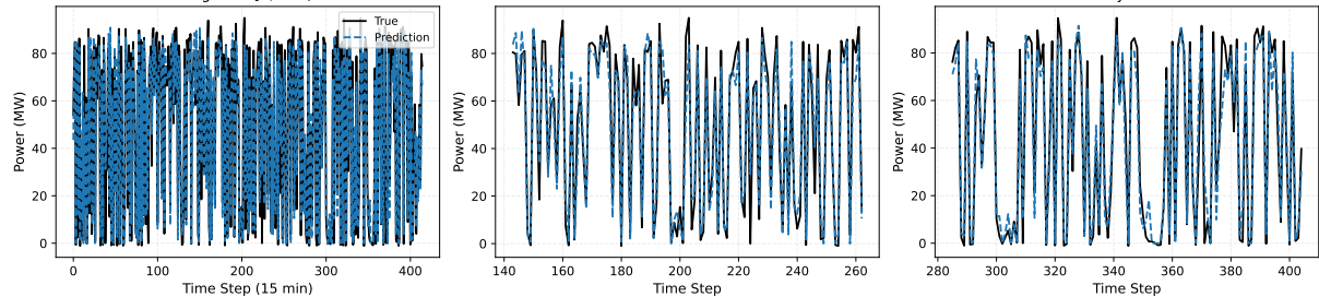
Fig. 3: Prediction-curve comparison on the Farm 6 extreme-weather test set (Part I). One row corresponds to one model, and each row contains the full segment plus peak/valley zoom views.
