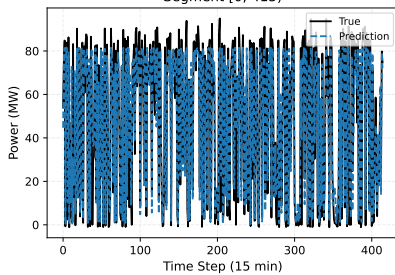
BRF-WPF vs True (Wind farm site 6 (Nominal capacity-96MW)) Segment [0, 415)
