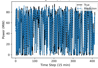
ARA-SVR vs True (Wind farm site 6 (Nominal capacity-96MW)) Segment [0, 415)
