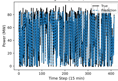
KMeans-GBT vs True (Wind farm site 6 (Nominal capacity-96MW)) Segment [0, 415)
