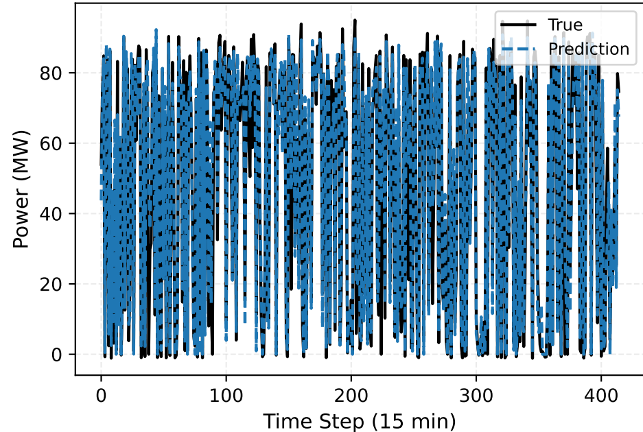
ARA-SVR vs True (Wind farm site 6 (Nominal capacity-96MW)) Segment [0, 415)
