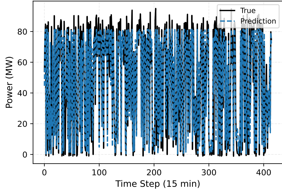
BRF-WPF vs True (Wind farm site 6 (Nominal capacity-96MW)) Segment [0, 415)
