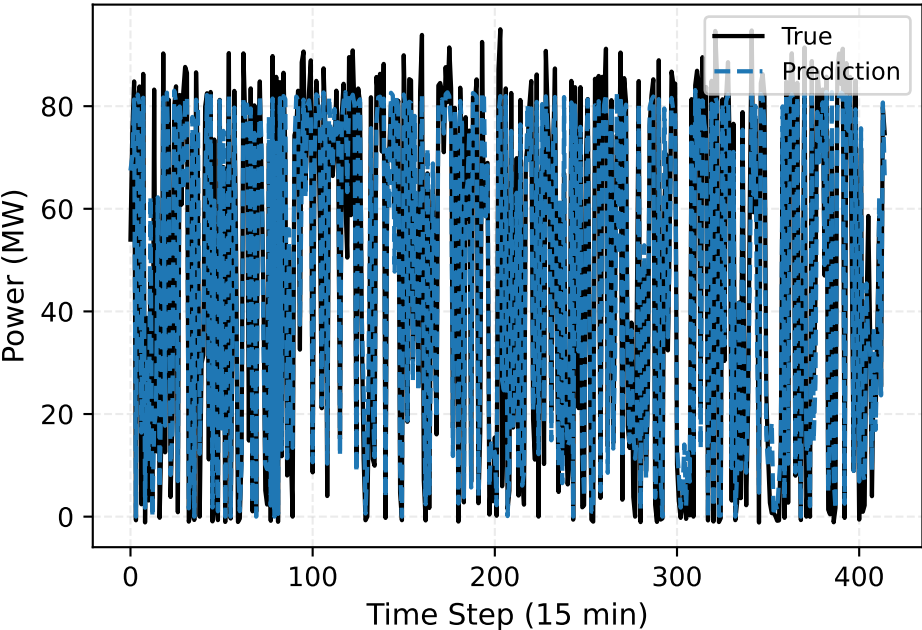
CNN-LSTM vs True (Wind farm site 6 (Nominal capacity-96MW)) Segment [0, 415)
