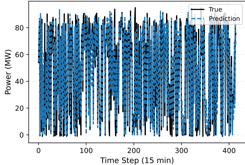
ELM vs True (Wind farm site 6 (Nominal capacity-96MW)) Segment [0, 415)
