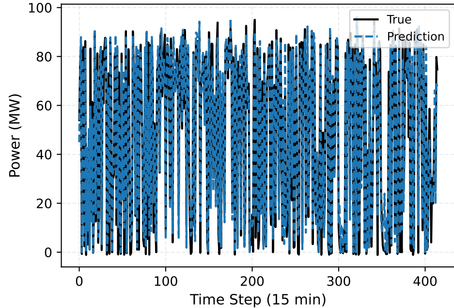
HHO-SVR vs True (Wind farm site 6 (Nominal capacity-96MW)) Segment [0, 415)
