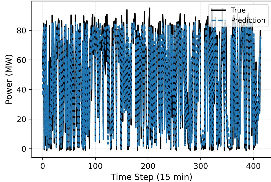
HistGBR vs True (Wind farm site 6 (Nominal capacity-96MW)) Segment [0, 415)
