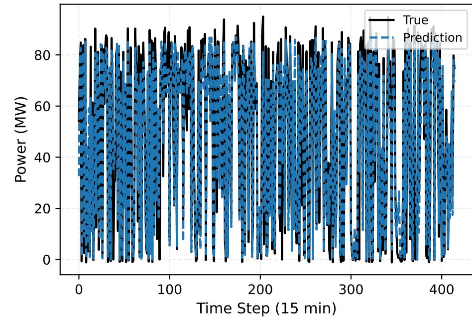
KMeans-GBT vs True (Wind farm site 6 (Nominal capacity-96MW)) Segment [0, 415)
