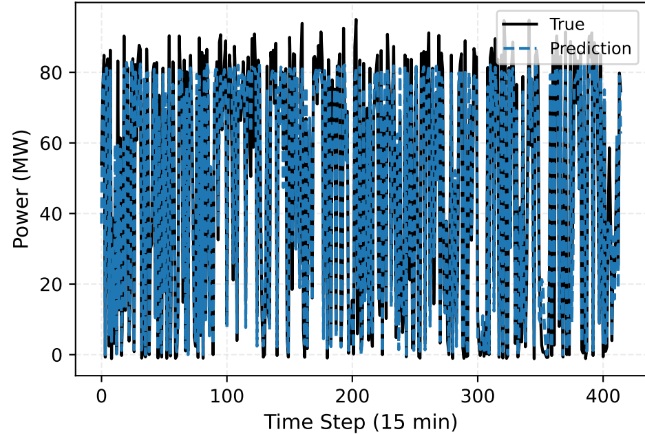
LSTM vs True (Wind farm site 6 (Nominal capacity-96MW)) Segment [0, 415)
