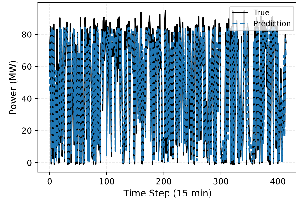
RandomForest vs True (Wind farm site 6 (Nominal capacity-96MW)) Segment [0, 415)
