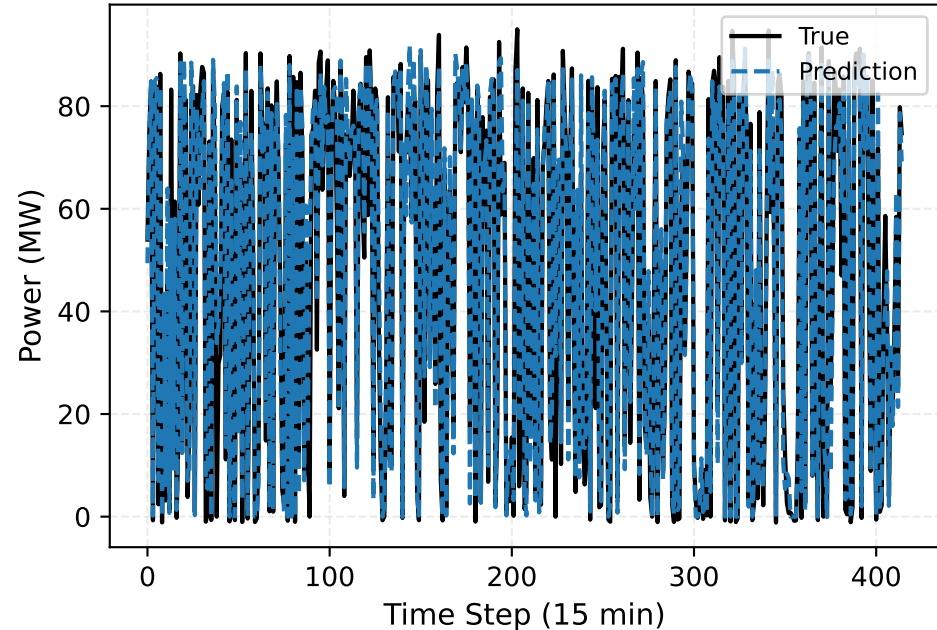
SVR vs True (Wind farm site 6 (Nominal capacity-96MW)) Segment [0, 415)
