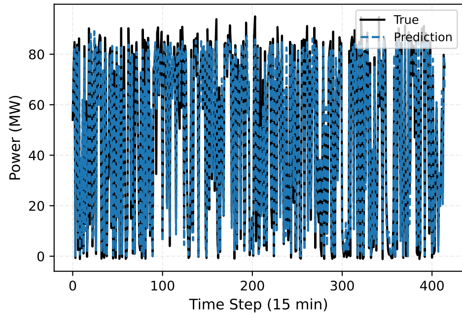
TL-LSTM vs True (Wind farm site 6 (Nominal capacity-96MW)) Segment [0, 415)
