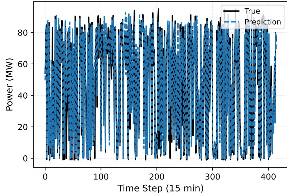
TL-SVR vs True (Wind farm site 6 (Nominal capacity-96MW)) Segment [0, 415)
