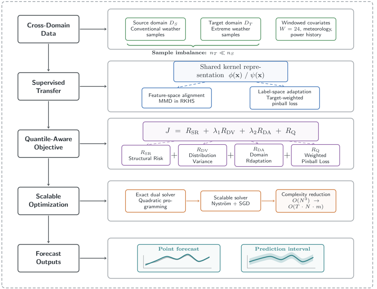
Fig. 1: Overall architecture of the proposed TL-QLDMR model. The left column shows the five-stage pipeline: cross-domain data preparation, supervised transfer learning, quantile-aware objective construction, scalable optimization, and forecast outputs. Each stage is elaborated in the corresponding right panel. In the supervised transfer stage, the shared kernel representation branches into feature-space alignment via MMD in RKHS and label-space adaptation via target-weighted pinball loss (indicated by dashed arrows). The quantile-aware objective decomposes into four additive terms: structural risk R_{SR} , distribution variance R_{DV} , domain adaptation R_{DA} , and weighted pinball loss R_Q . The optimization stage provides both an exact dual QP solver and a scalable Nyström + SGD solver with complexity reduction from O(N^3) to O(T \cdot N \cdot m) . The final outputs include deterministic point forecasts and probabilistic prediction intervals.
