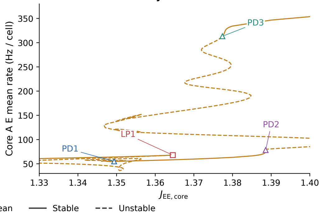
b Reference slice: cycle nodes
