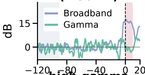
high-gamma (80-150 Hz)
