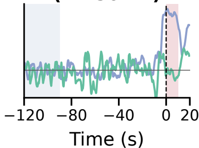
broadband (1-150 Hz)
