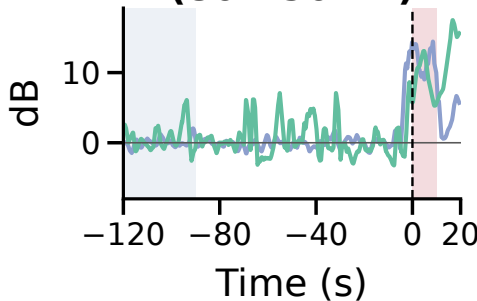
high-gamma (80-150 Hz)
