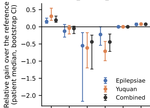
converged_teacher_forced vs current_teacher_forced_reference
