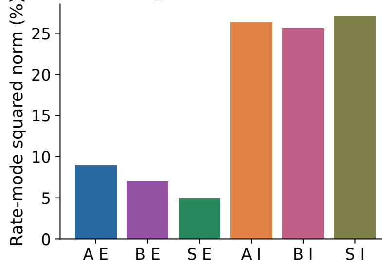
Right critical mode
