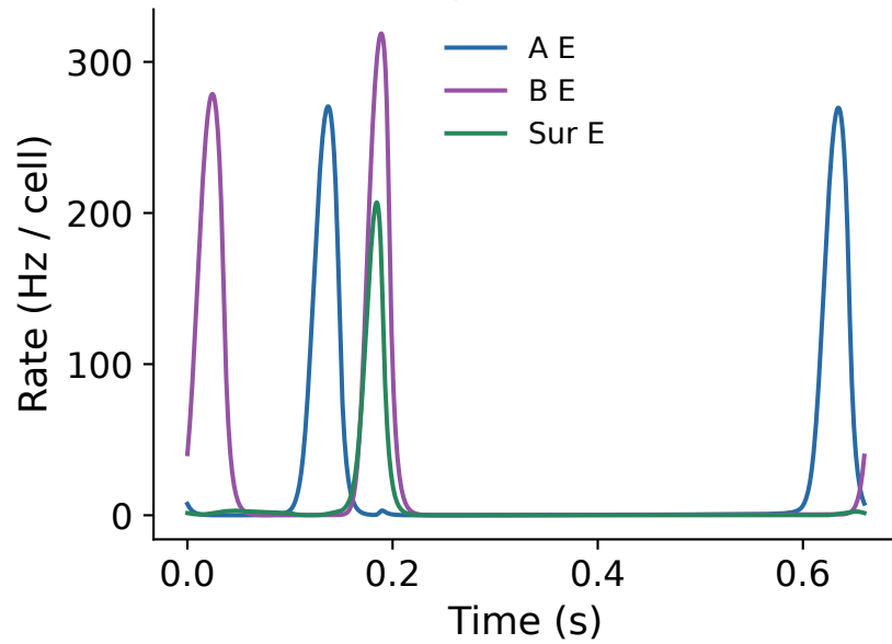
Cycle fold: J_{EE,core}=1.1762730100
