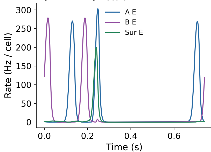
Cycle fold: J_{EE,core}=1.1762479453
