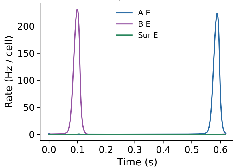
Cycle fold: J_{EE,core}=1.1218172204
