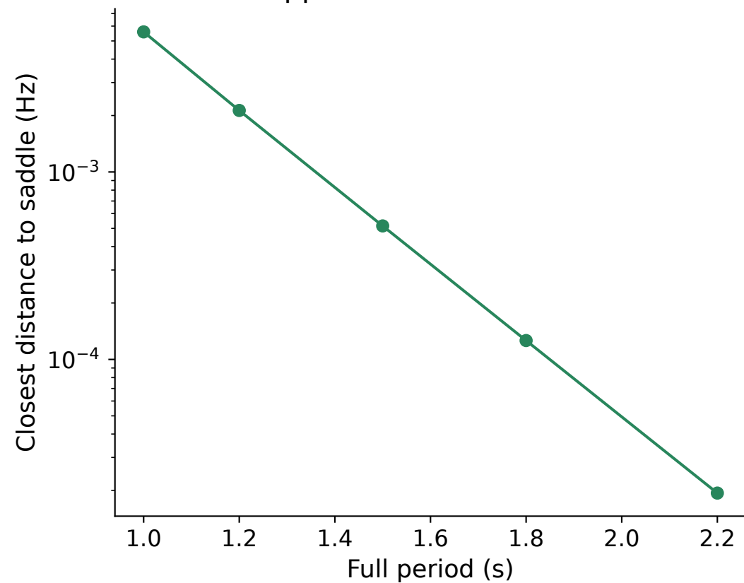
Orbit approaches the same saddle
