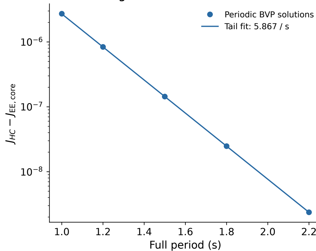
Convergence to the homoclinic limit
