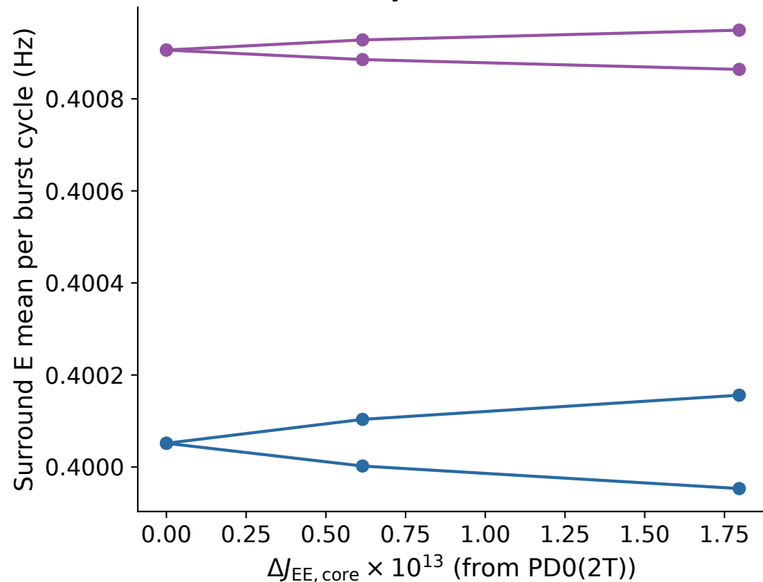
Four distinct cycles on the 4T branch
