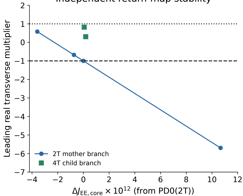
Independent return-map stability
