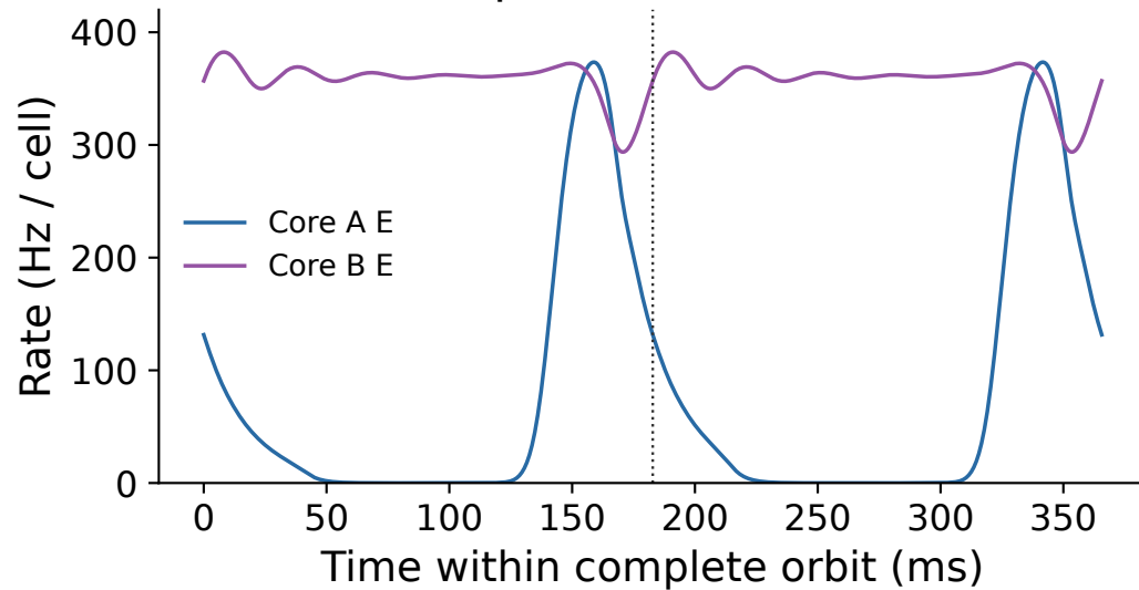
PD2: complete 2T = 365.632 ms
