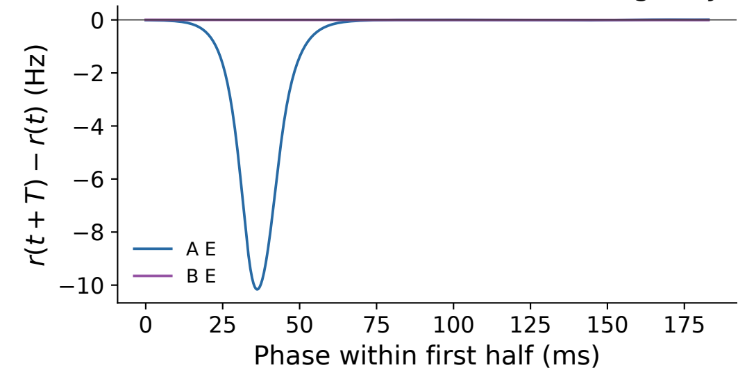
Unstable 2T ; subcritical toward higher J
