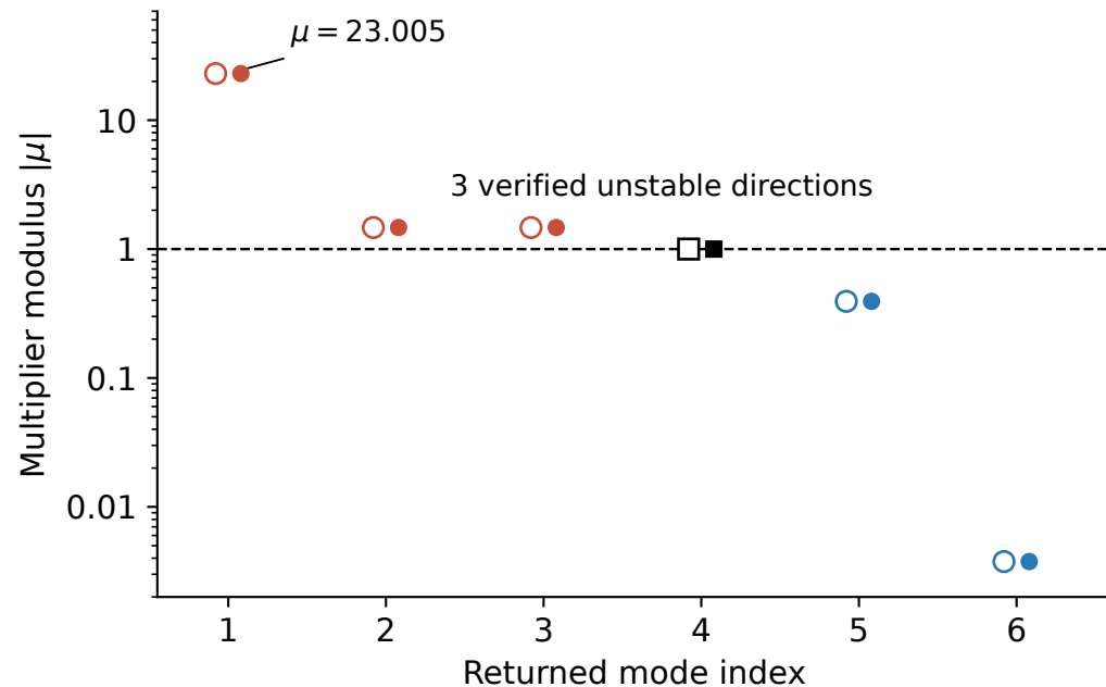
B All six returned modes
