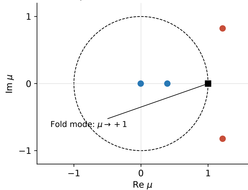
A Spectrum near the unit circle
