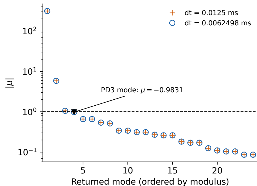
A Three unstable directions
