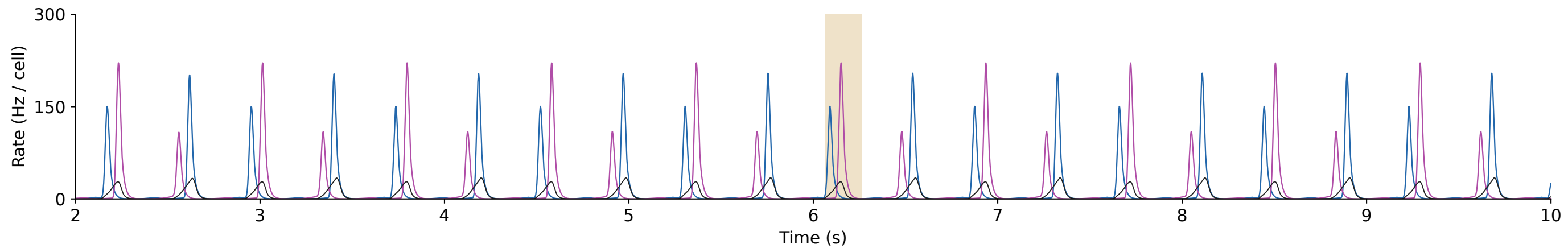
b H1 < J < H2 : alternating intervals, J=0.942 — autonomous spatial rate model
