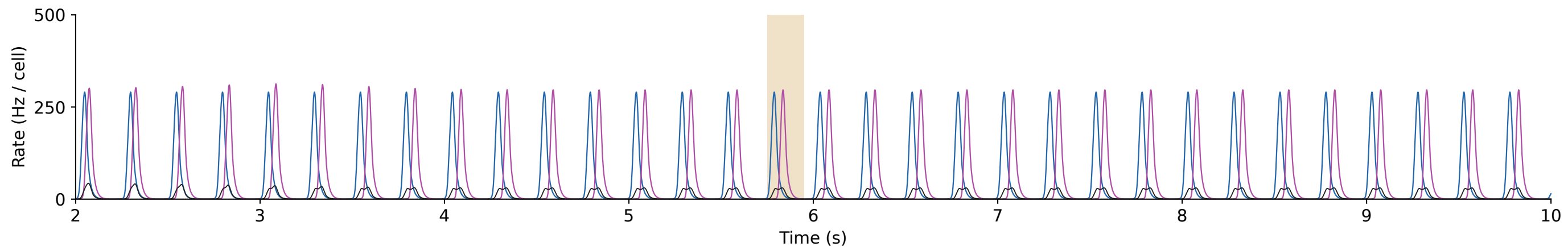
d Regular bursts, J=1.3 — autonomous spatial rate model
