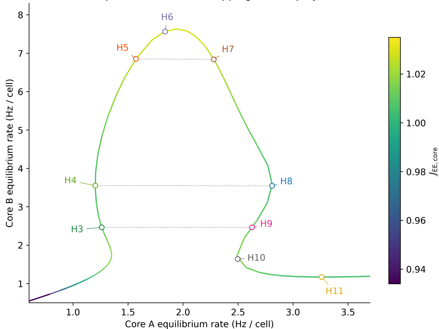
Different equilibria behind overlapping branch projections
