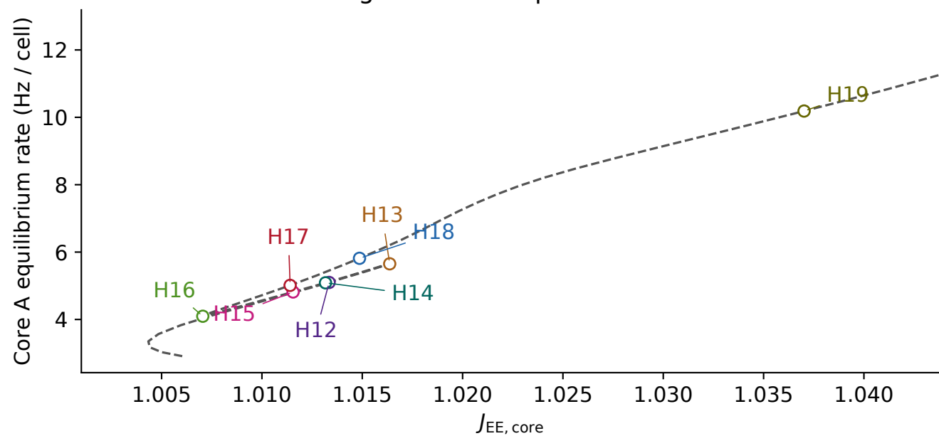
A Higher folded equilibria: Core A
