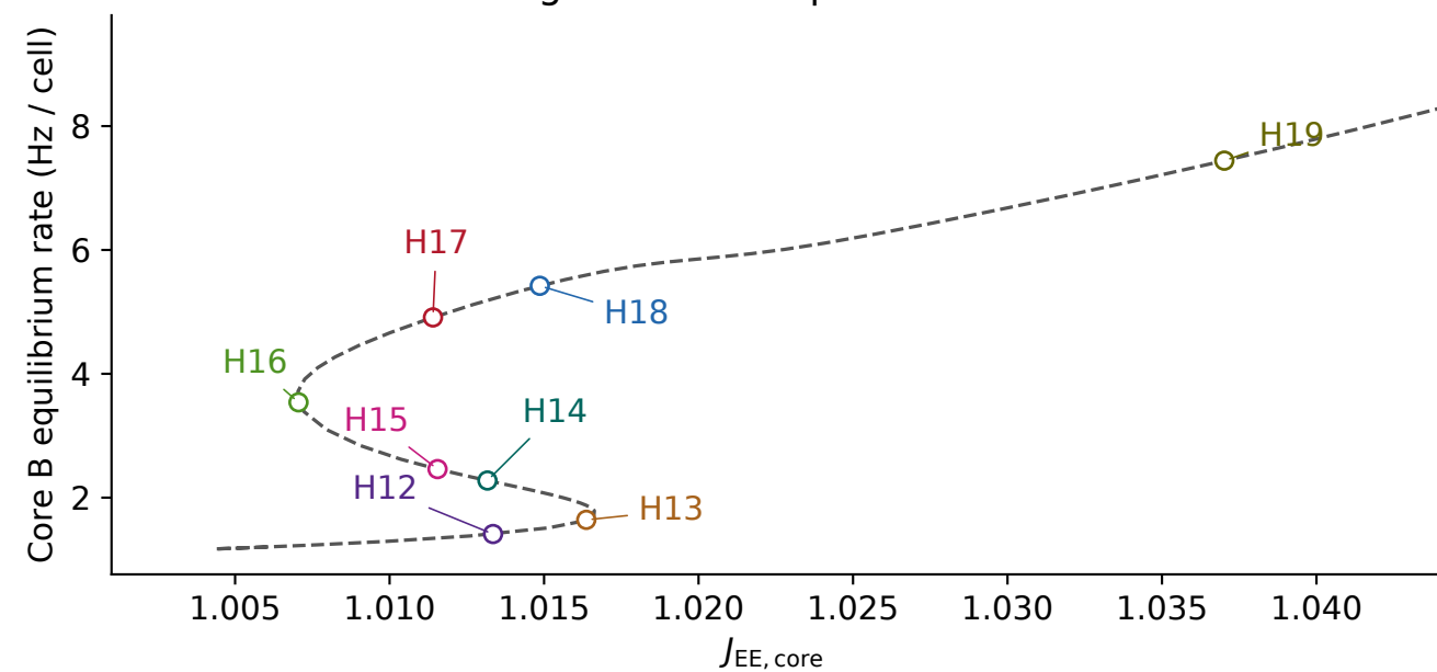
B Higher folded equilibria: Core B
