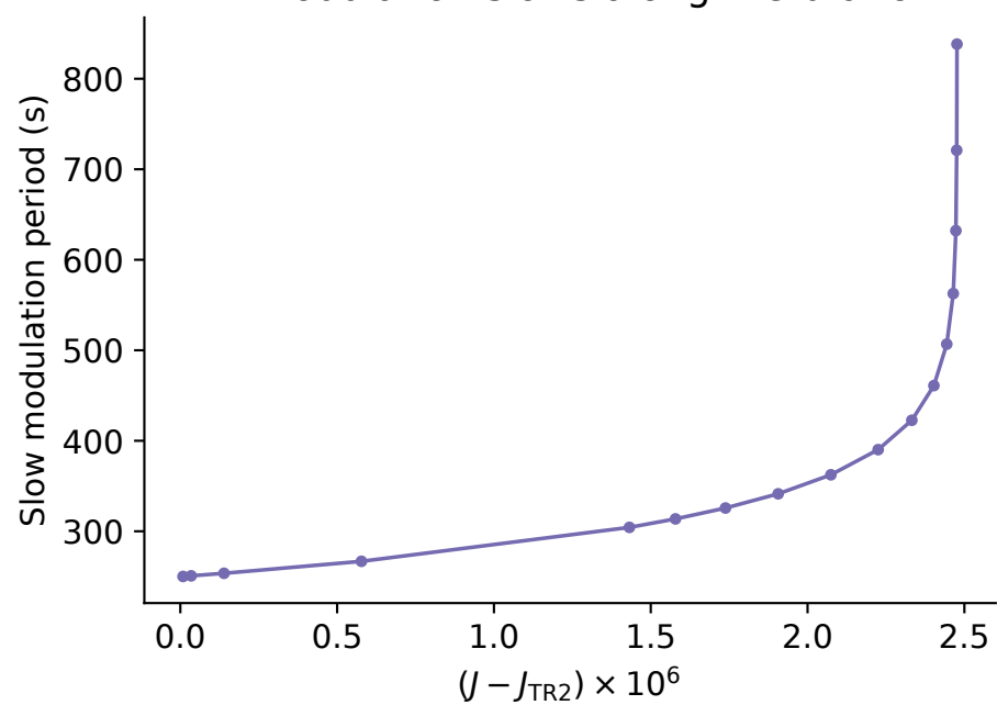
B Modulation slows along the branch
