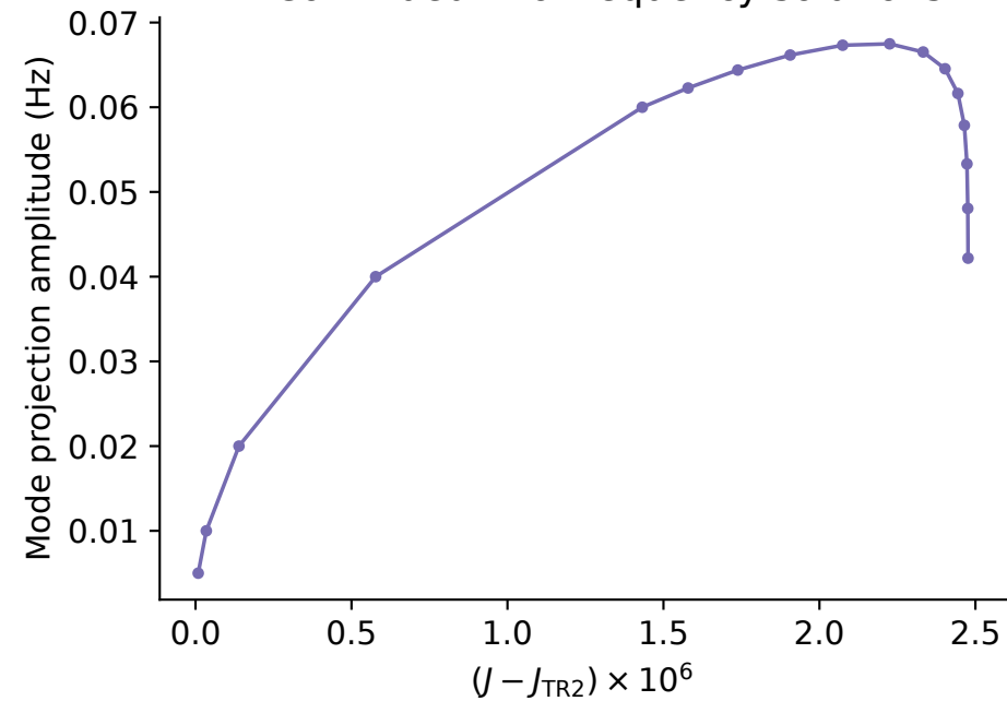
A Continued two-frequency solutions
