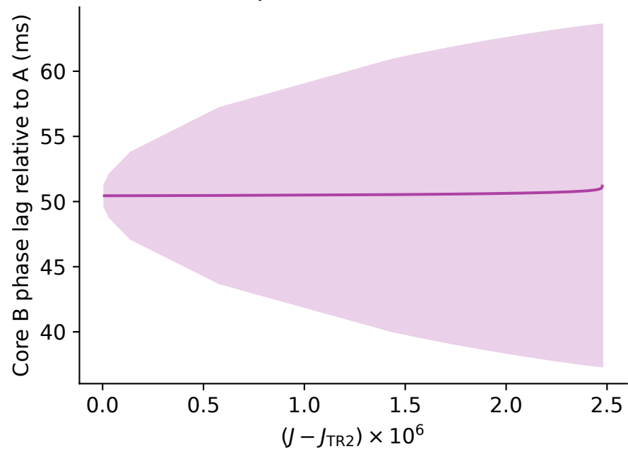
D Relative phase varies within a torus
