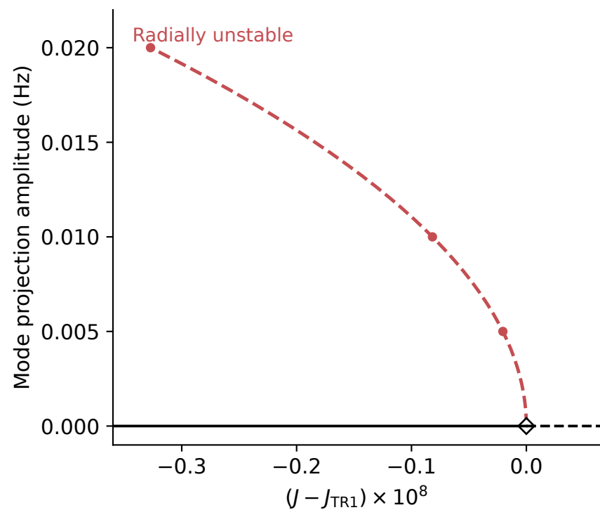
B TR1: subcritical
