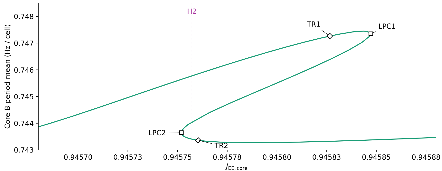
A Two torus bifurcations on the folded H1 branch
