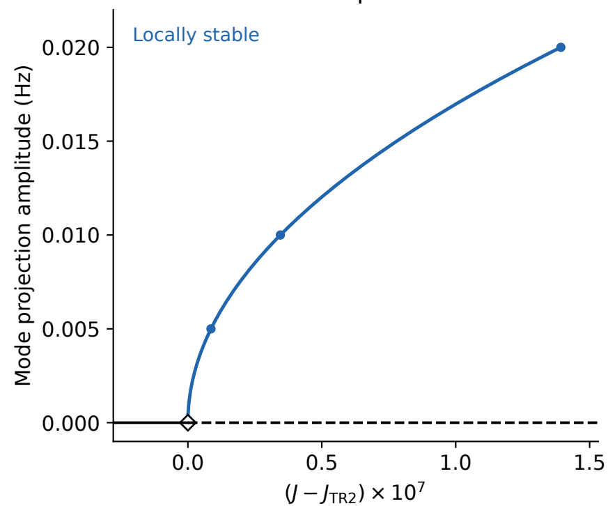
C TR2: supercritical
