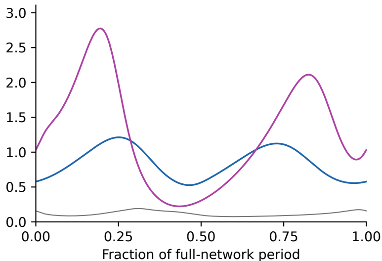
LPC14 | J_{EE, \text{core}} = 0.947681 T = 303.39 ms; A:B harmonics = 2:1
