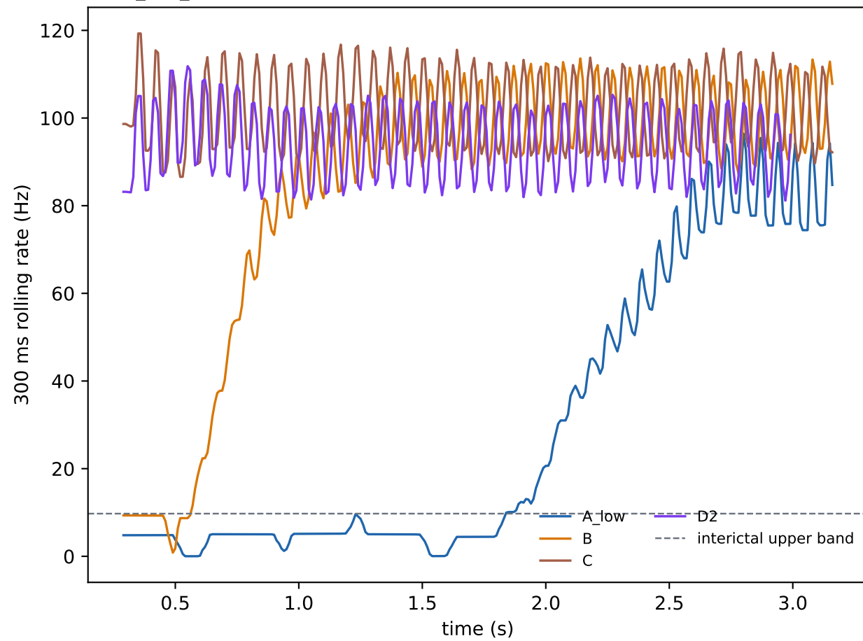
c H6_k05_r10: healthy self-escalation and failed X return
