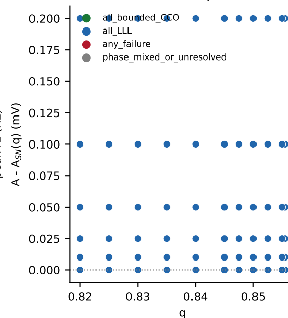
C Instantaneous A steps all reach LLL
