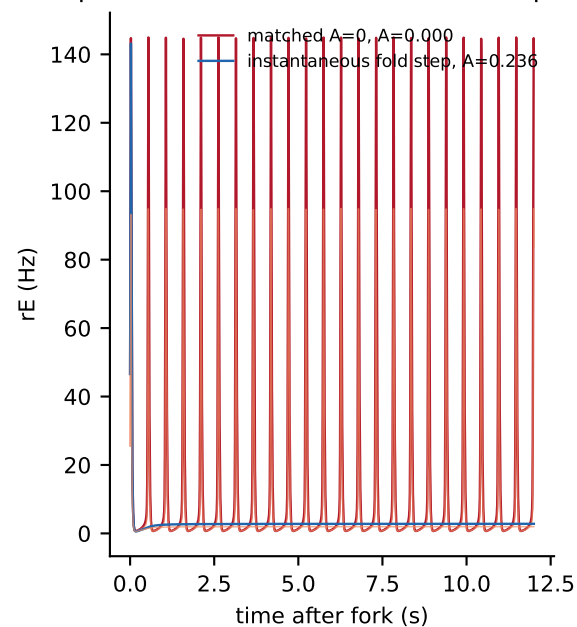
E Representative event-locked fork at q=0.8400
