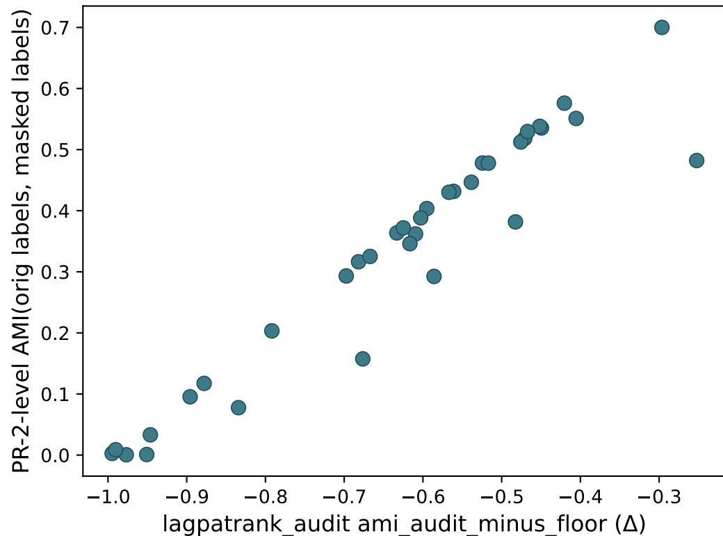
Sanity: audit signal vs PR-2 rerun AMI
