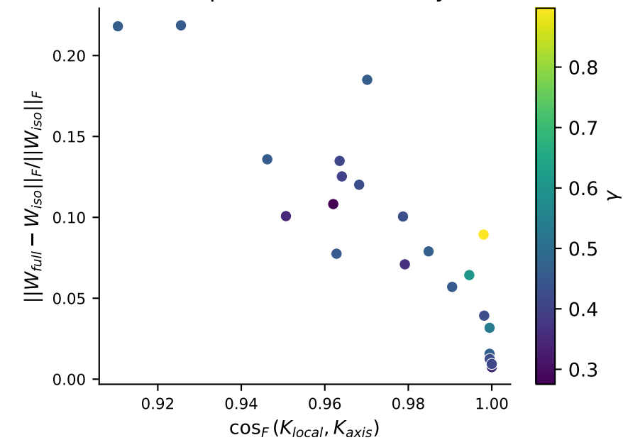
C Operator identifiability
