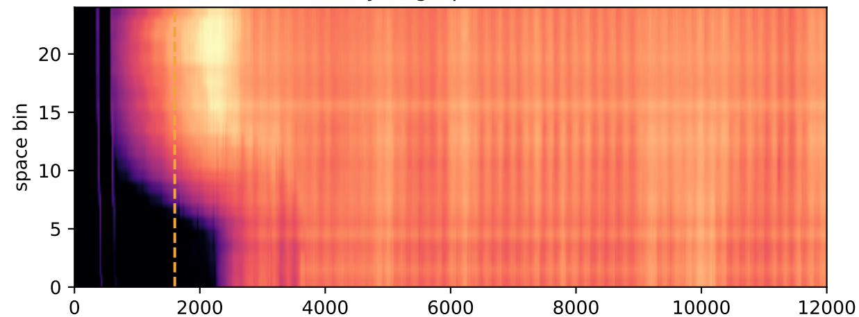
kymograph: transverse
