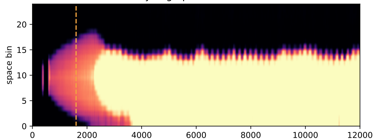
kymograph: transverse
