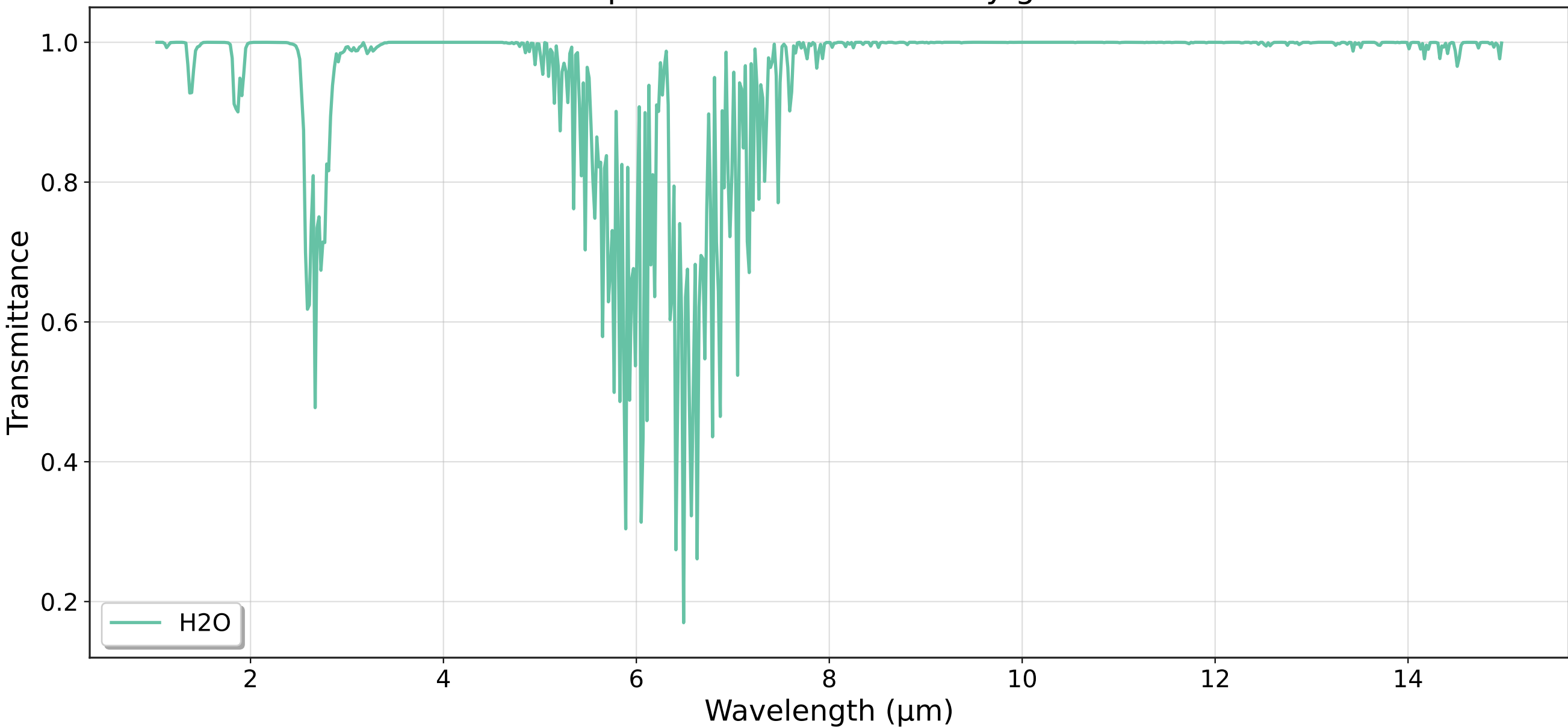
Spectral transmittance by gas
