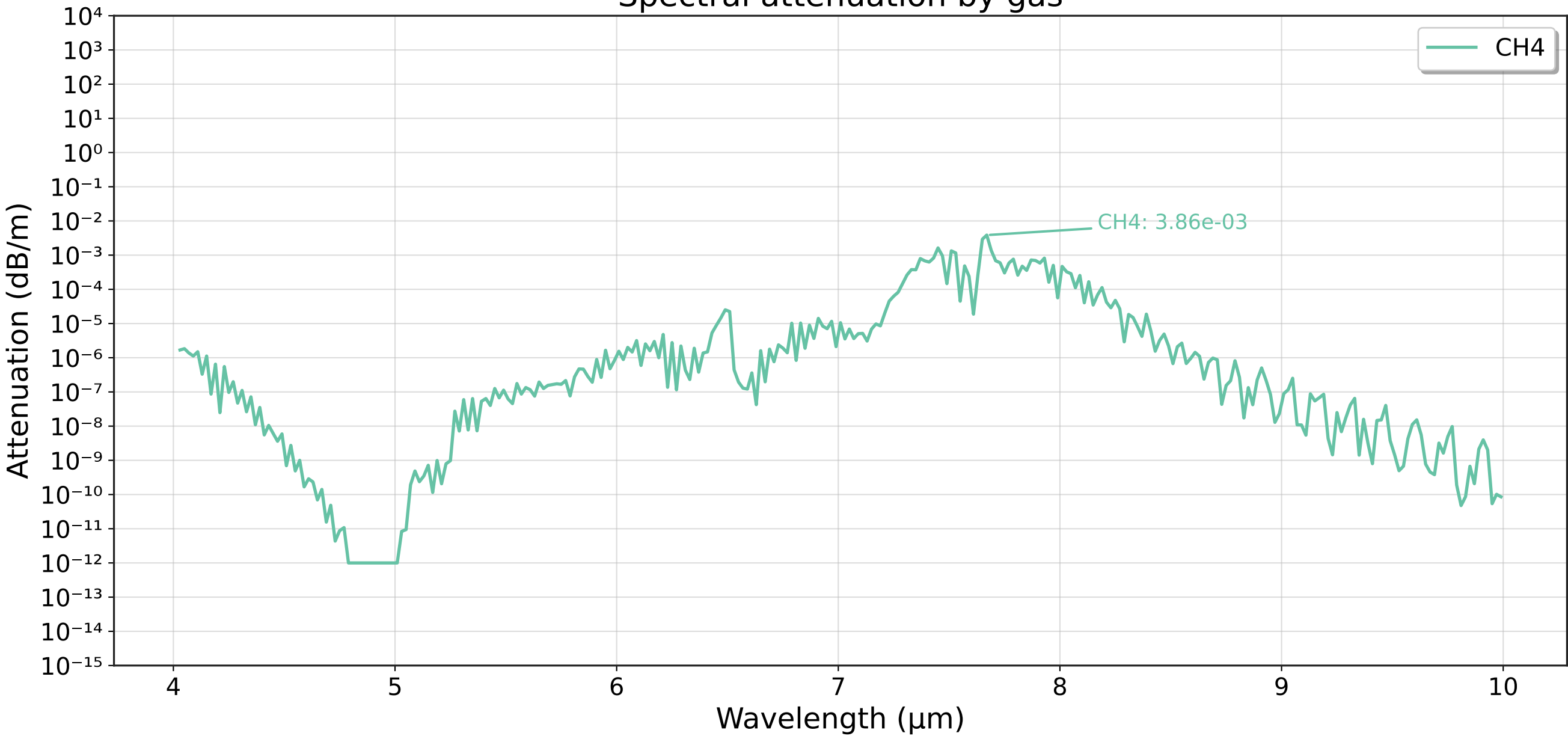
Spectral attenuation by gas
