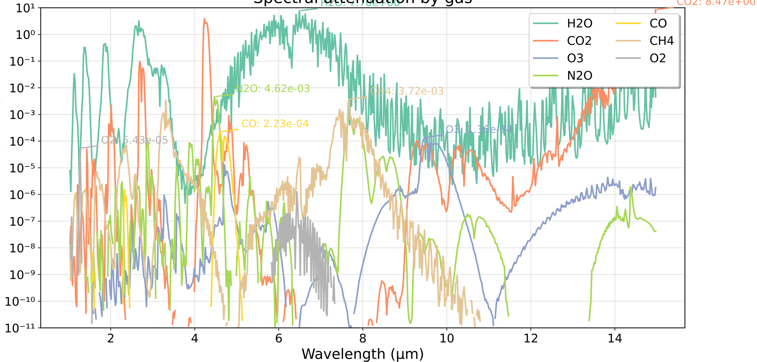
Spectral attenuation by gas
