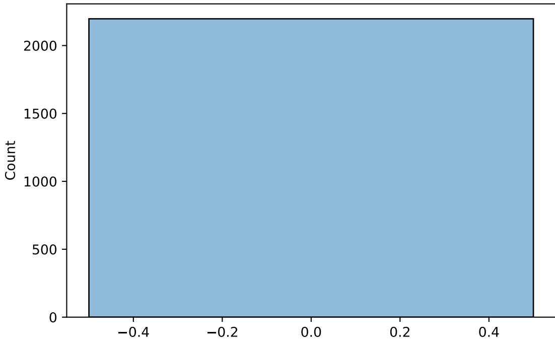
Chaos Distribution (Lyapunov Estimates)
