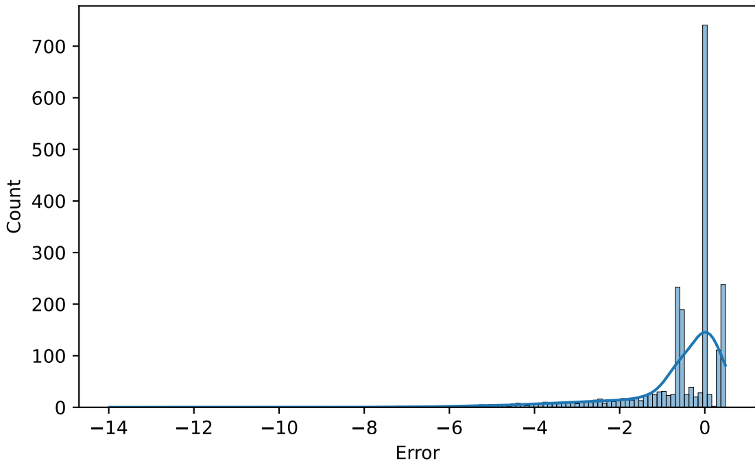
Prediction Error Distribution
