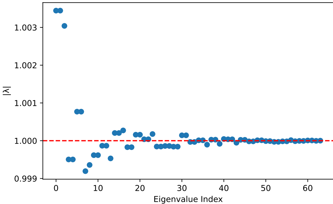
Spectral Radius of Contraction Map ( I - \eta(I - W) )
