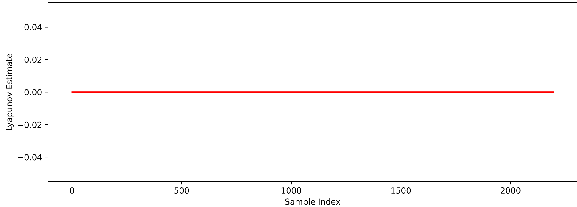
Chaos Map (Lyapunov Exponent Trajectory)
