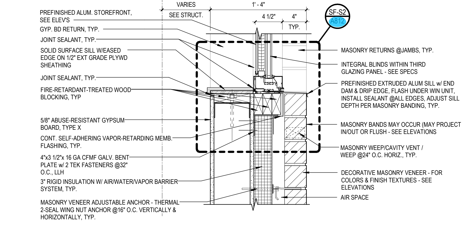
9 TYPICAL DETAIL SCALE: 1 1/2" = 1'-0" REF. FROM: 7 / A540
