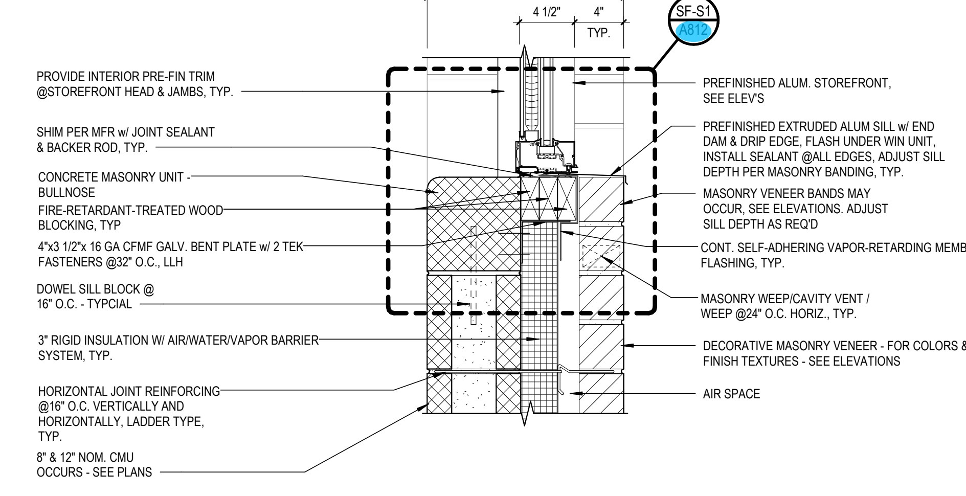
10 TYPICAL DETAIL SCALE: 1 1/2" = 1'-0" REF. FROM: 1 / A512
