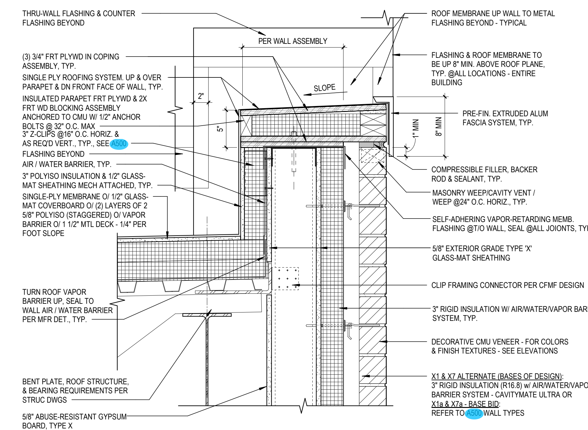
1 TYPICAL COPING DETAIL - BRICK VENEER / CFM SCALE: 1 1/2" = 1'-0" REF. FROM: 5 / A540
