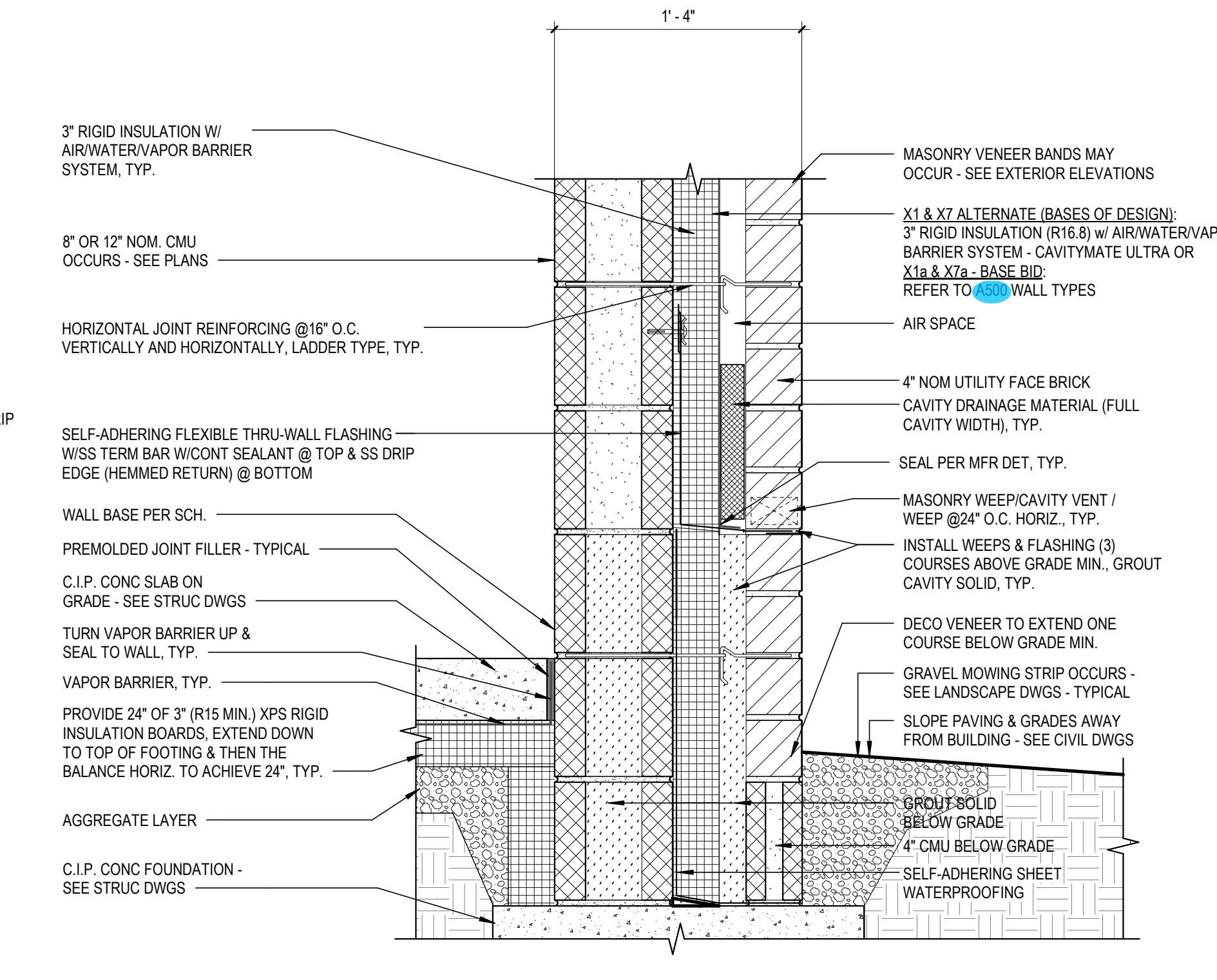
13 TYPICAL DETAIL SCALE: 1 1/2" = 1'-0" REF. FROM: 1 / A511
