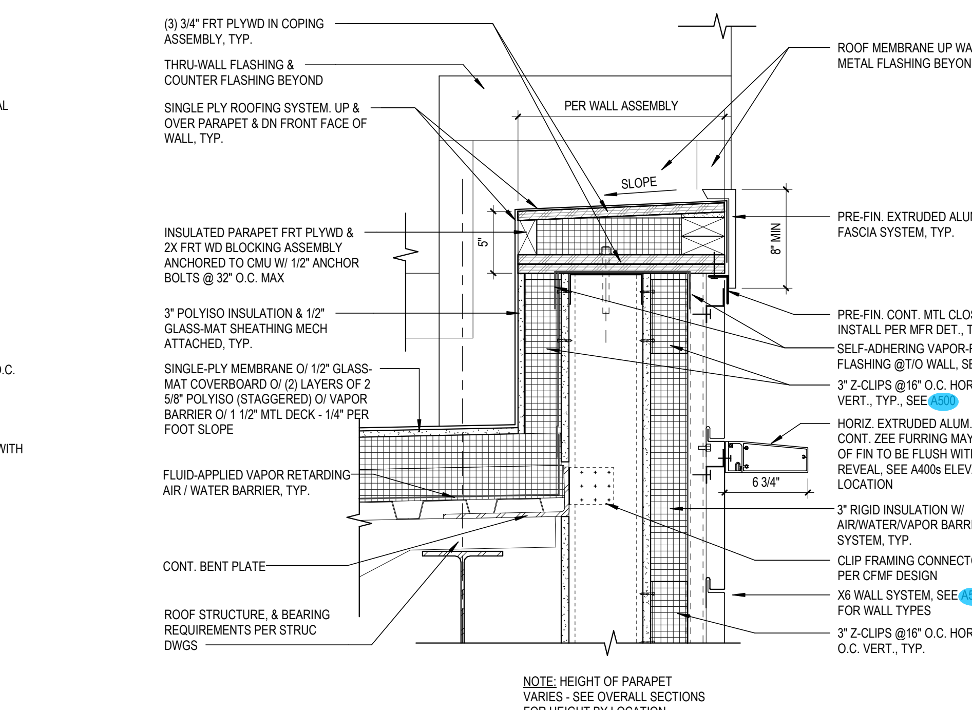
4 TYPICAL COPING DETAIL - RAINSCREEN / CFM SCALE: 1 1/2" = 1'-0" REF. FROM: 4 / A521
