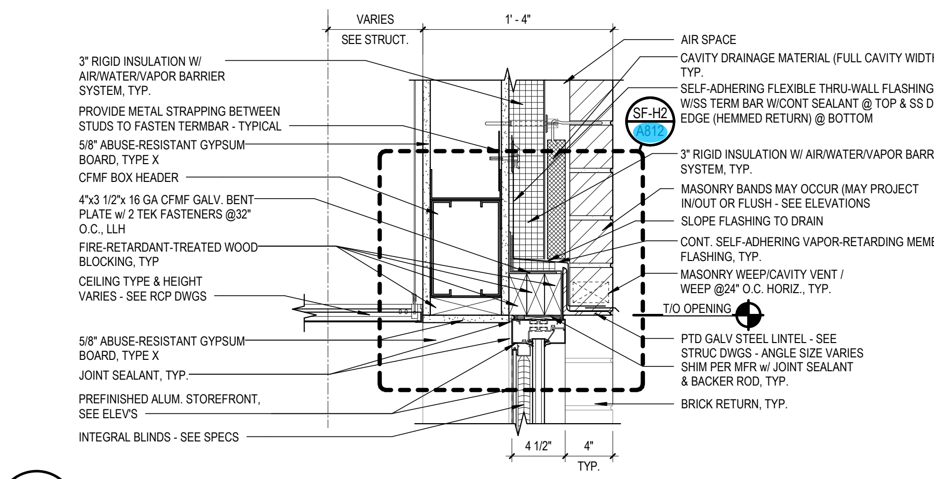
5 TYPICAL DETAIL SCALE: 1 1/2" = 1'-0" REF. FROM: 7 / A540
