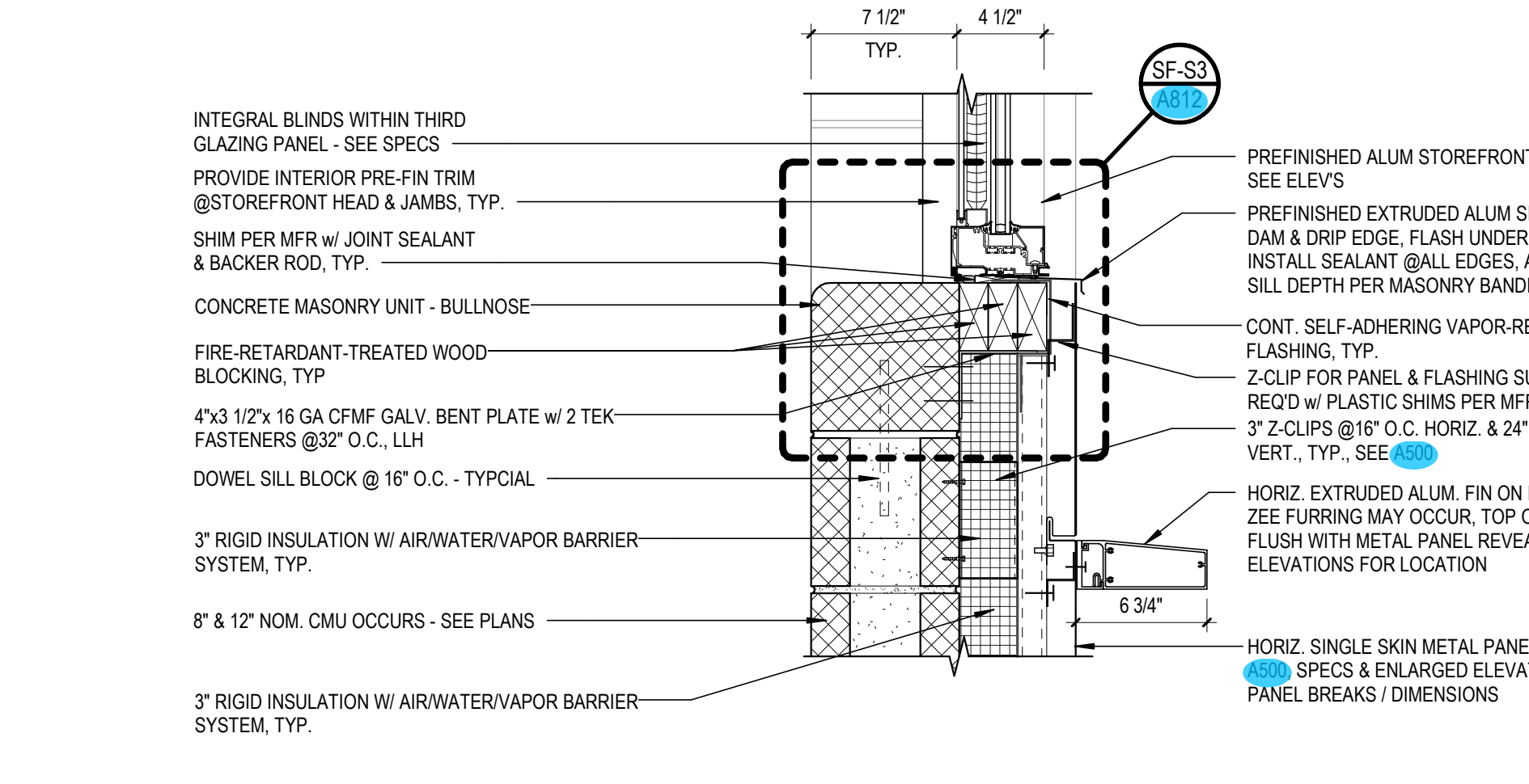
11 TYPICAL DETAIL SCALE: 1 1/2" = 1'-0" REF. FROM: 1 / A521
