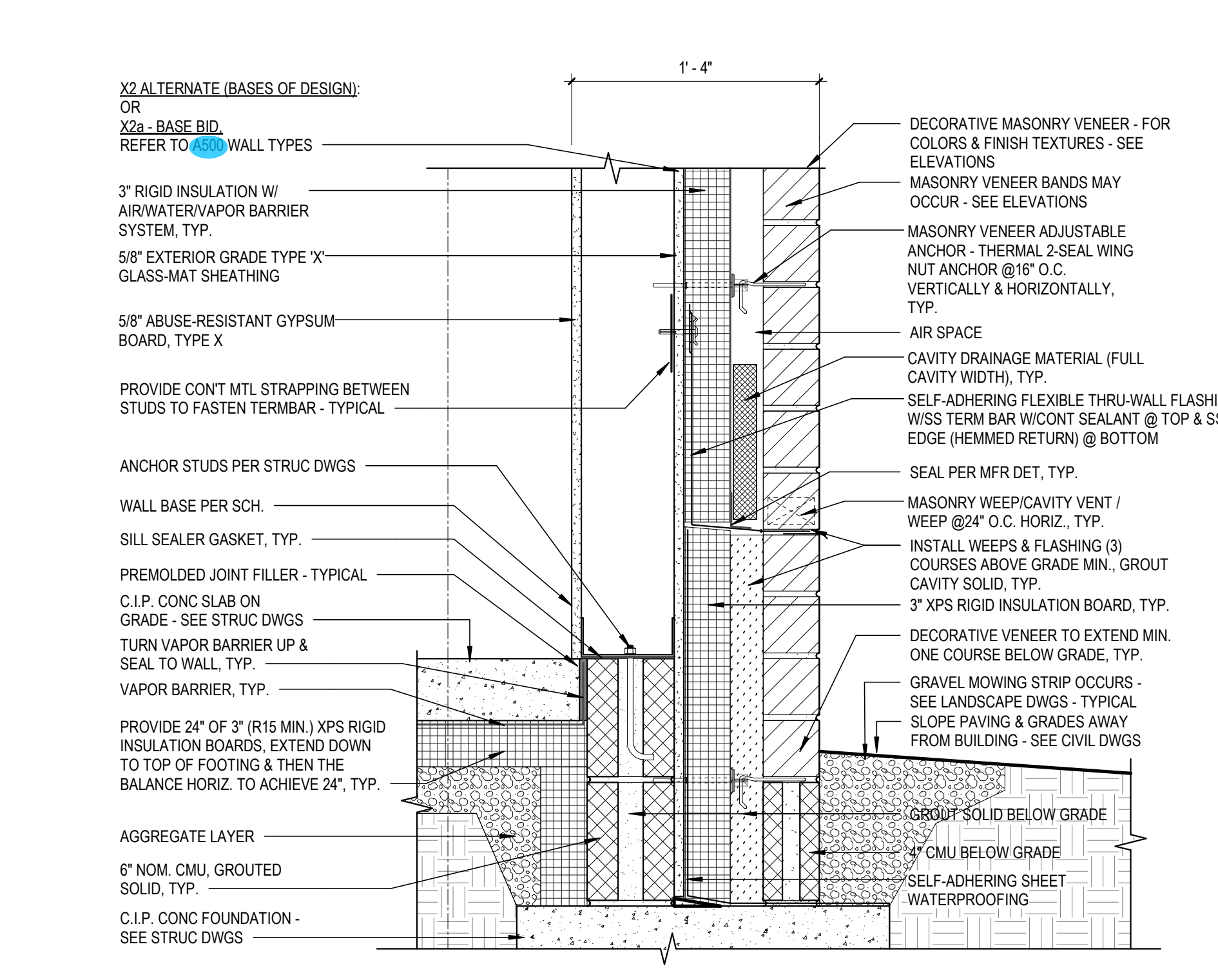
12 TYPICAL DETAIL SCALE: 1 1/2" = 1'-0" REF. FROM: 5 / A540
