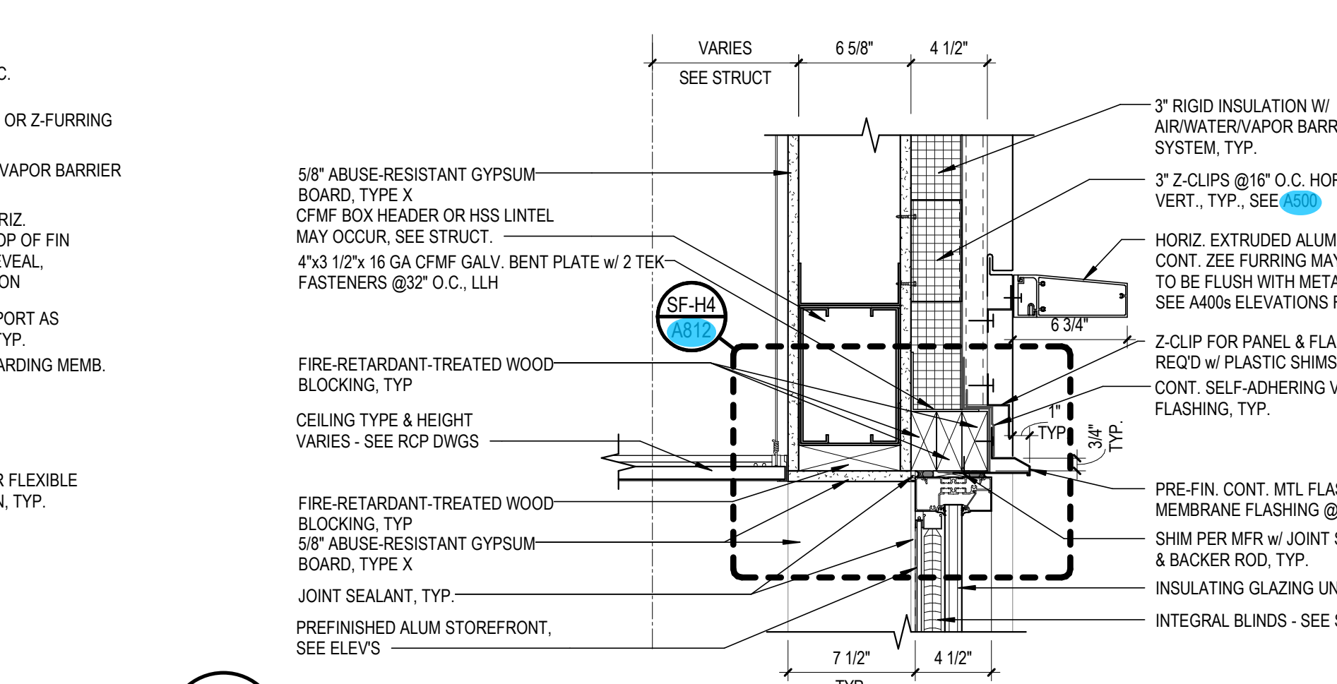
8 TYPICAL DETAIL SCALE: 1 1/2" = 1'-0" REF. FROM: 4 / A521
