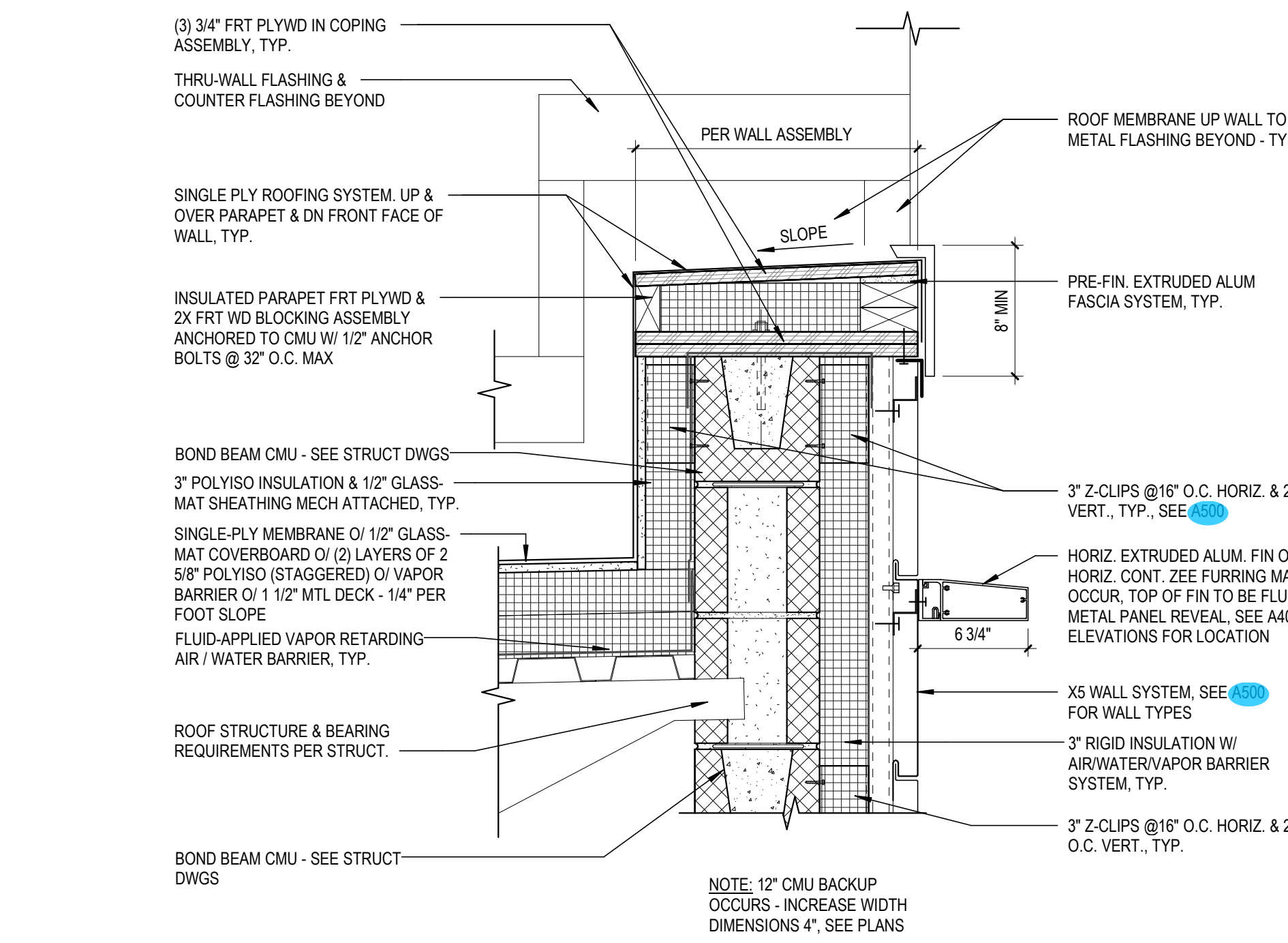
3 TYPICAL COPING DETAIL - RAINSCREEN / CMU SCALE: 1 1/2" = 1'-0" REF. FROM: 1 / A521
