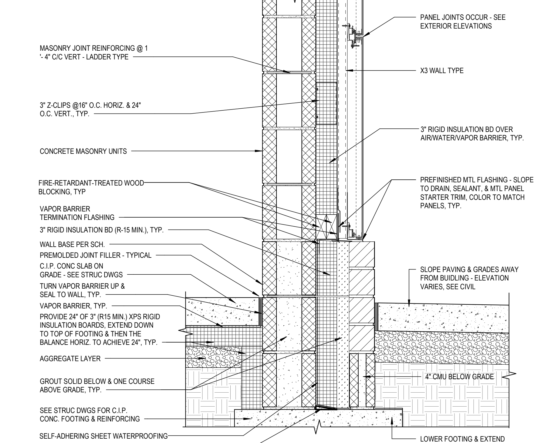
14 TYPICAL DETAIL SCALE: 1 1/2" = 1'-0" REF. FROM: 6 / A521
