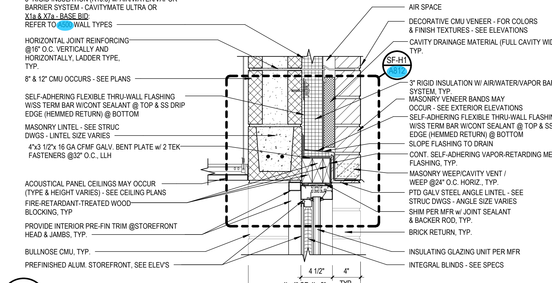
6 TYPICAL DETAIL SCALE: 1 1/2" = 1'-0" REF. FROM: 1 / A512
