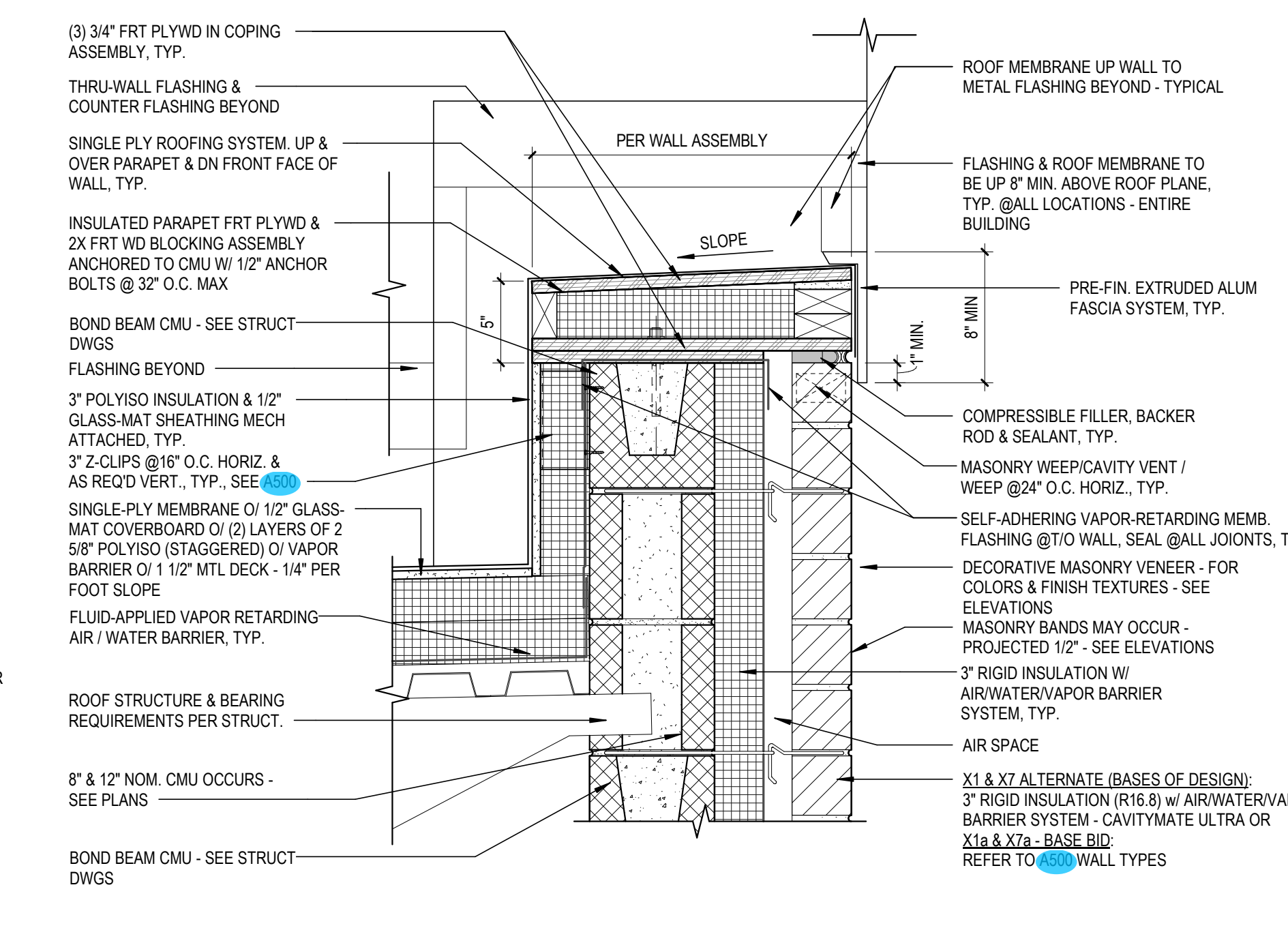
2 TYPICAL COPING DETAIL - BRICK VENEER / CMU SCALE: 1 1/2" = 1'-0" REF. FROM: 5 / A510
