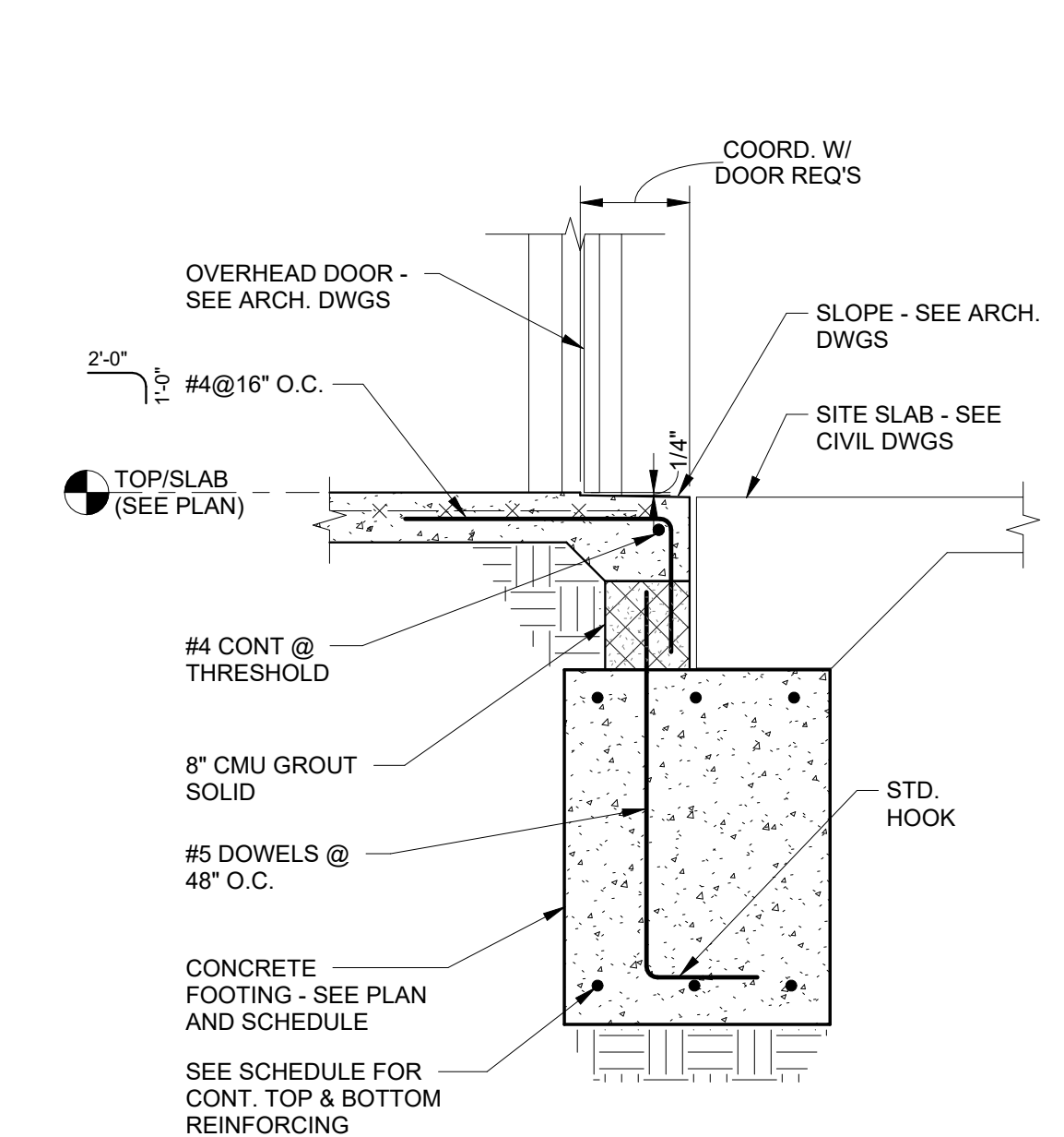
TYPICAL THICKENED SLAB DETAIL
