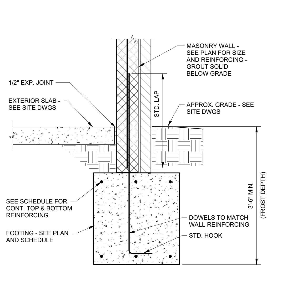
MASONRY SCREEN WALL DETAIL
