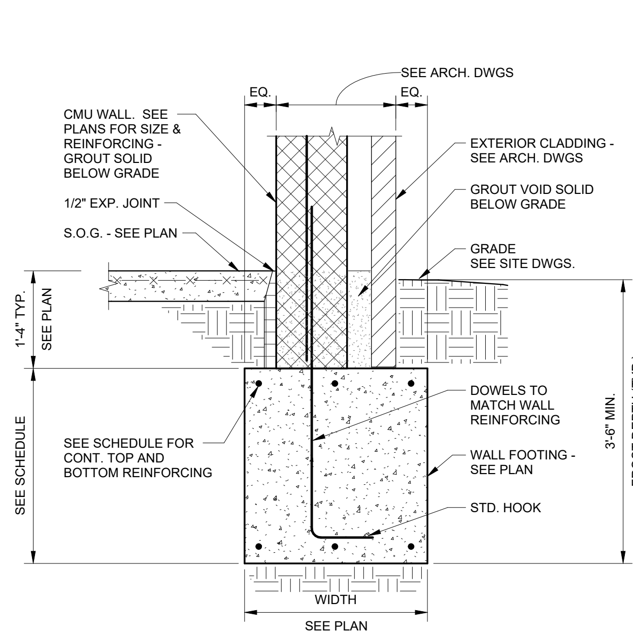
EXTERIOR TRENCH FOOTING DETAIL
