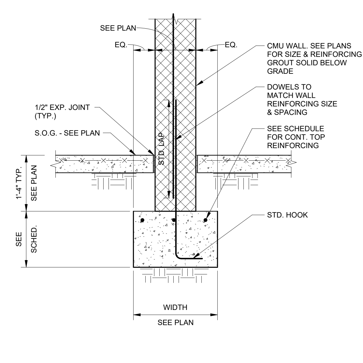
INTERIOR TRENCH FOOTING DETAIL
