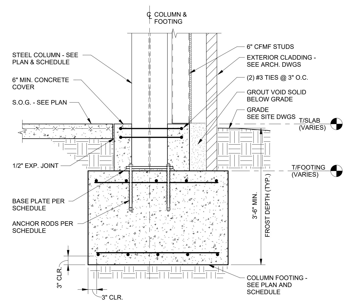
EXTERIOR COLUMN FOOTING DETAIL
