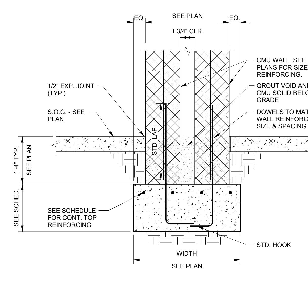
FIREWALL TRENCH FOOTING DETAIL
