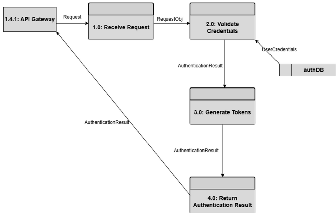
DFD Figure – 1.4.2.0.0.1 –
