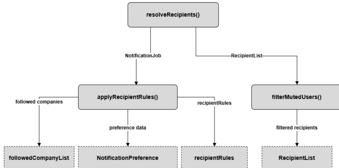
SC Figure 1.10.6.1 – resolveRecipient()
