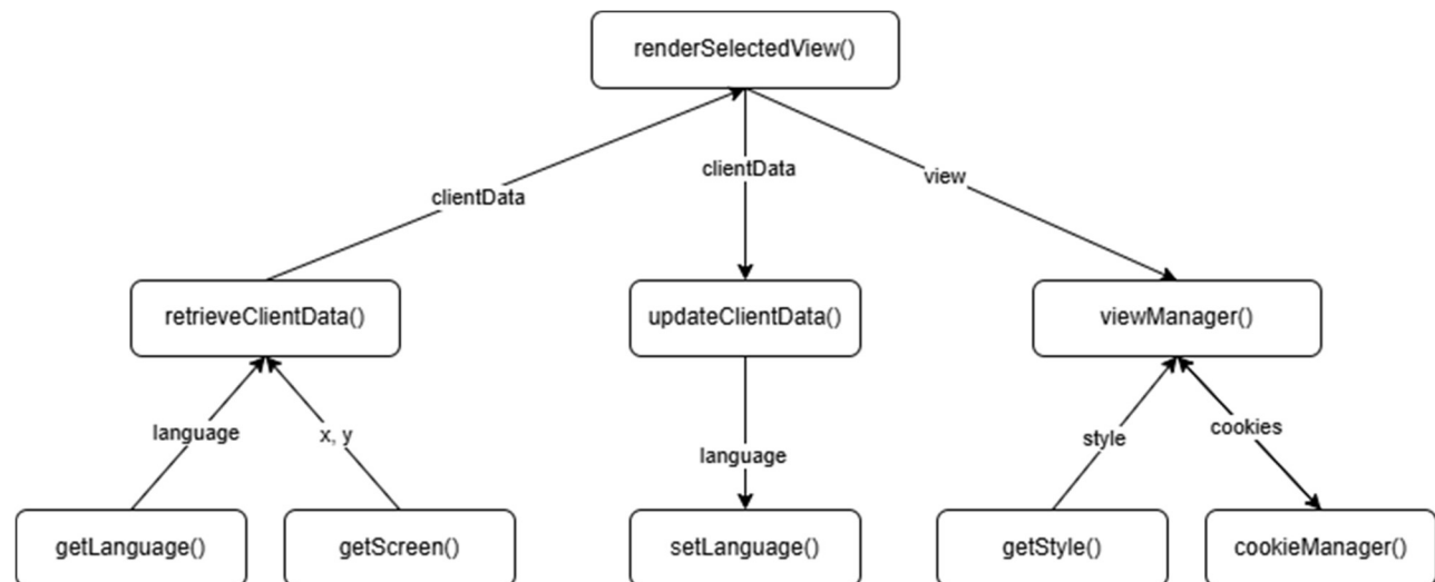
SC Figure 1.2.0.1 & 1.3.0.1 – renderSelectedView()
