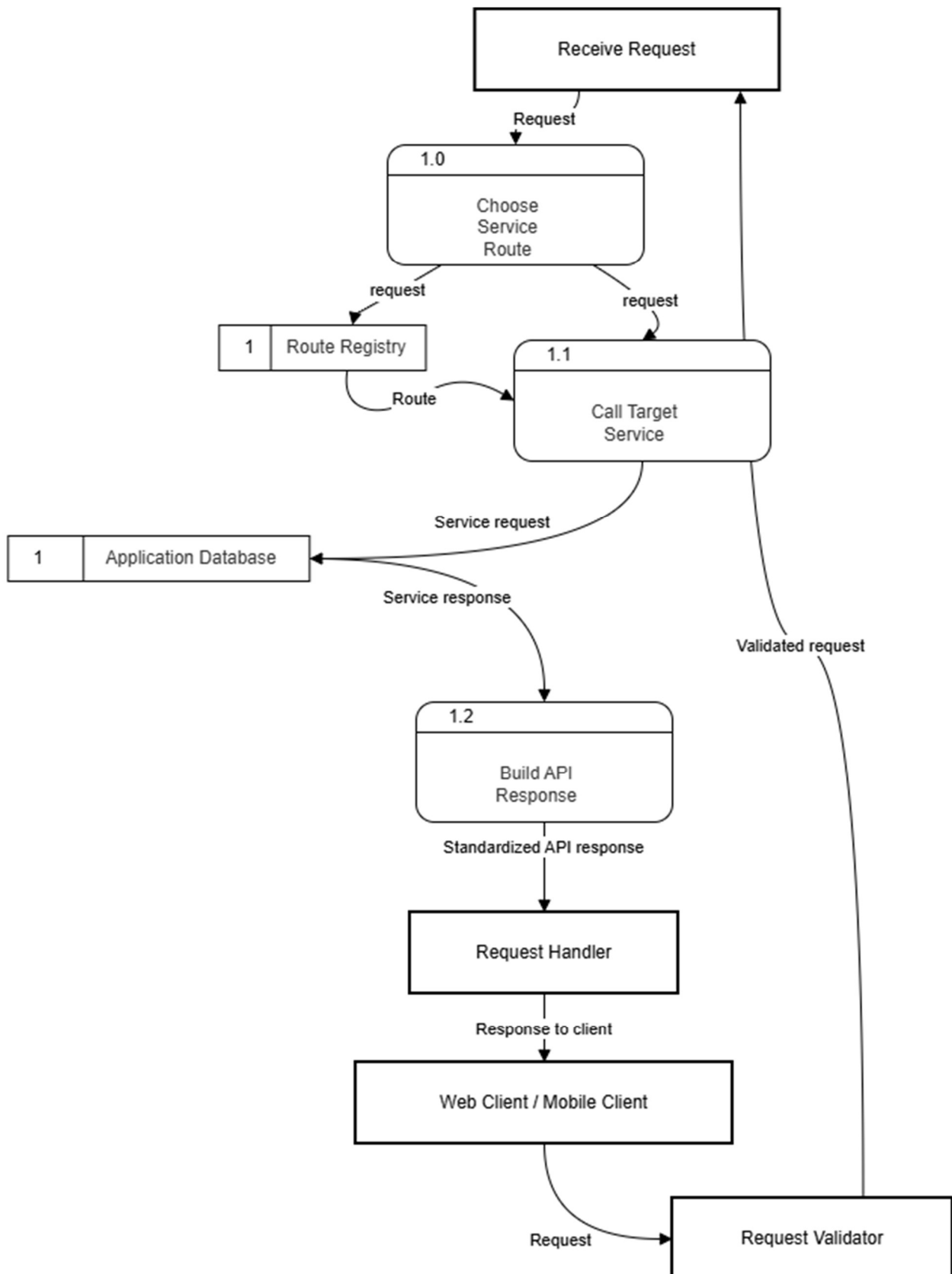
DFD Figure – 1.4.5.0.0.1 – Service Orchestrator Pattern
