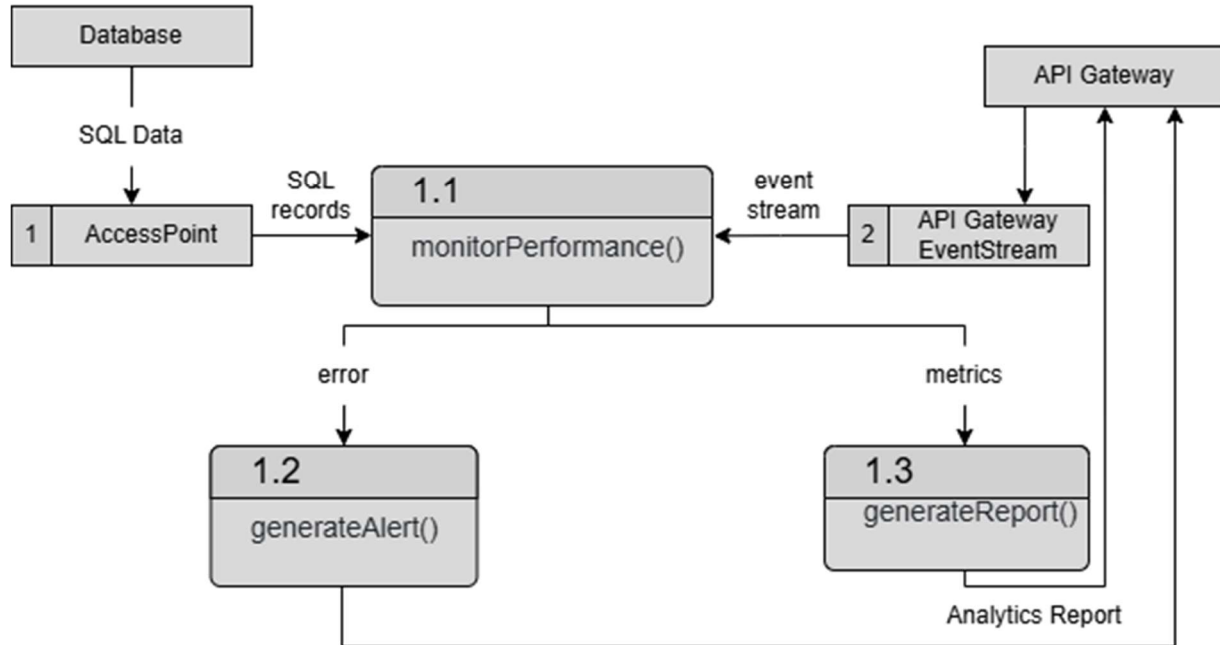
DFD 1.13.0.0.5 — Performance Monitor
