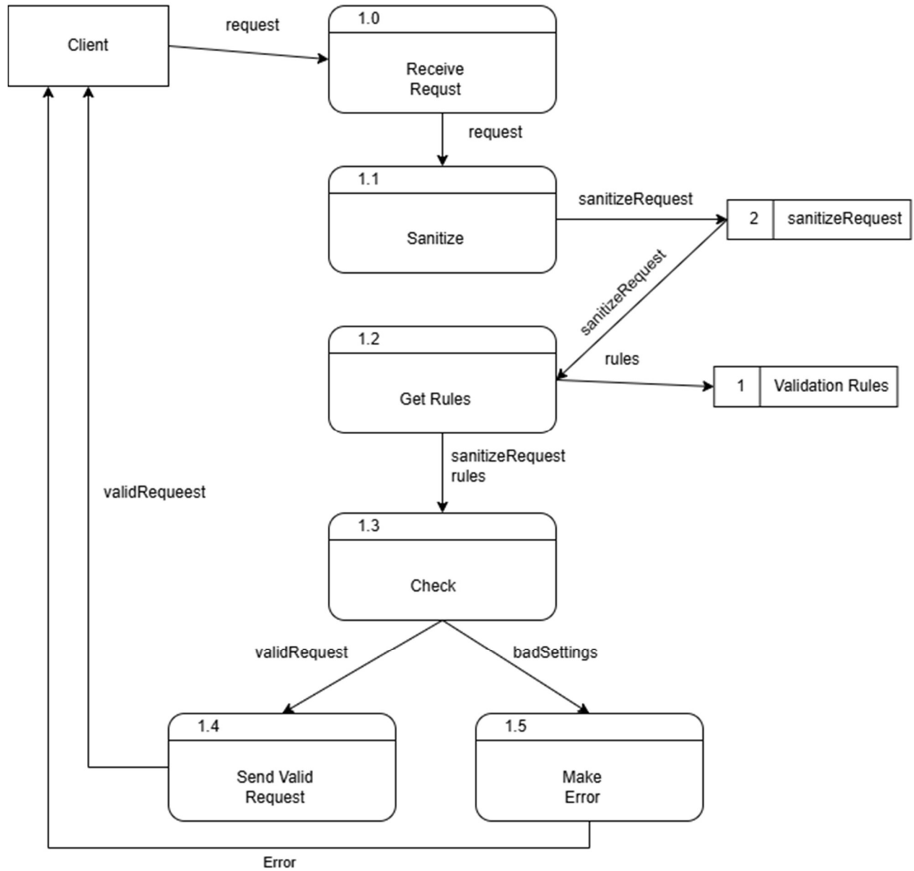
DFD Figure – 1.4.4.0.0.1 – Request Validator
