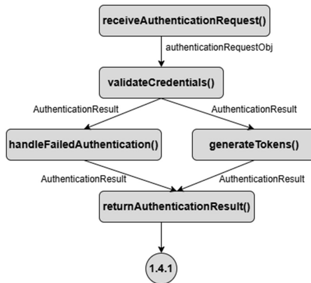
SC Figure 1.4.0.11 – External Services Orchestrator
