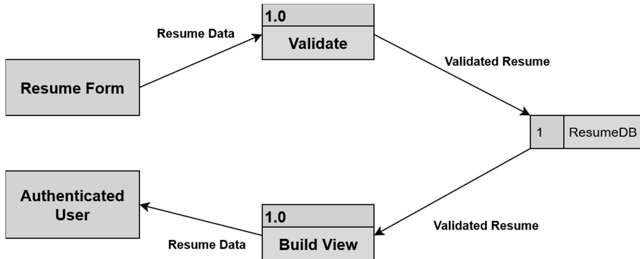
DFD Figure 1.7.0.0.2 — Submission and Storage Workflow
