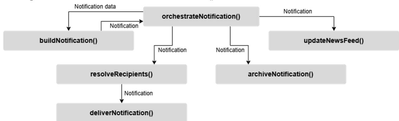
SC Figure 1.10.3.1 – orchestrateNotification()
