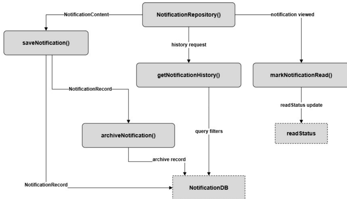
SC Figure 1.10.5.1 – notificationRepository()
