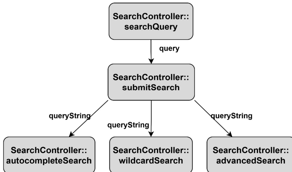
SC Figure 1.9.0.1 – SearchQuery()
