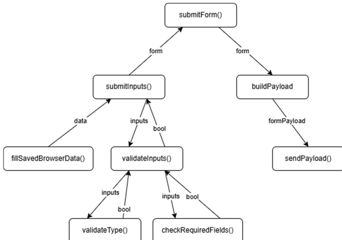
SC Figure 1.2.0.2 & 1.3.0.2 – submitForm()
