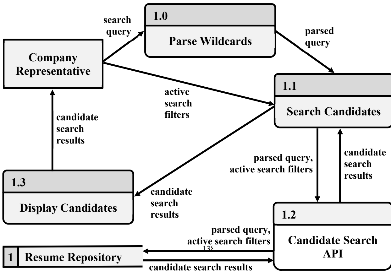
DFD Figure 1.13.2.0.0.1 — Candidate Search Workflow
