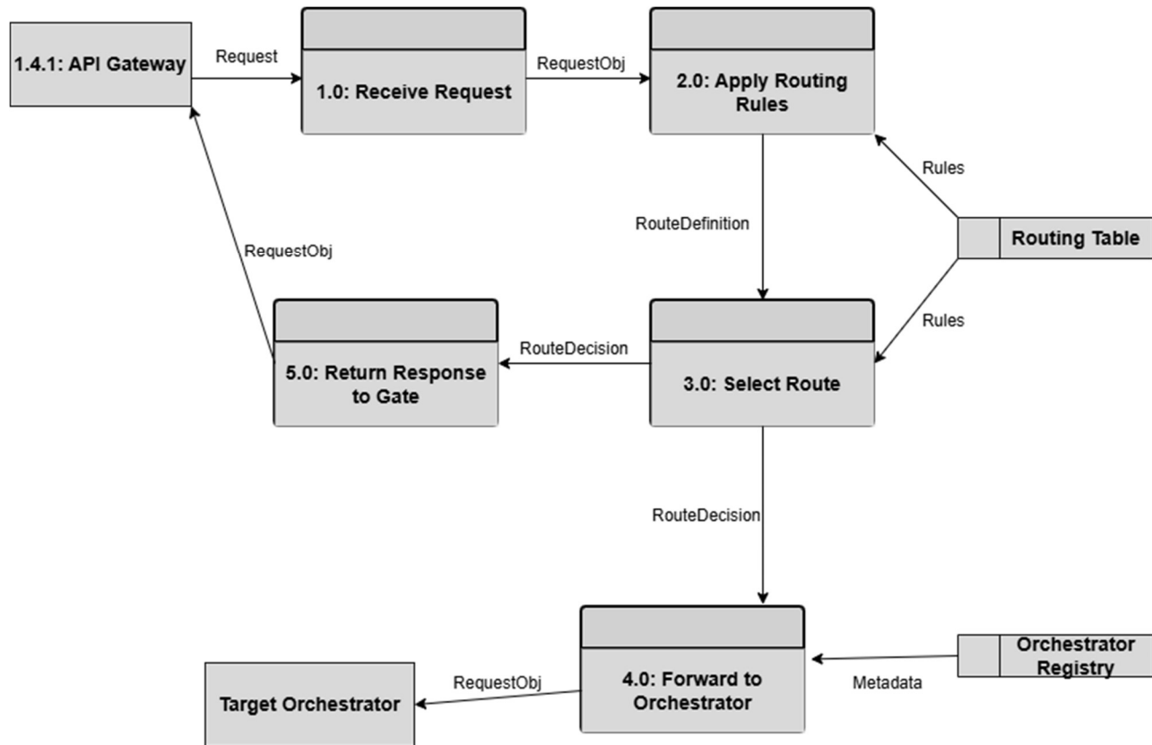
DFD Figure – 1.4.3.0.0.1 –
