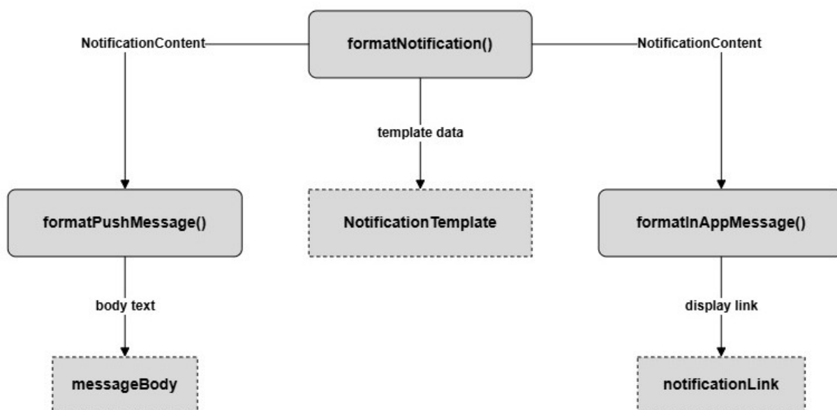
SC Figure 1.10.4.1 – formatNotification()
