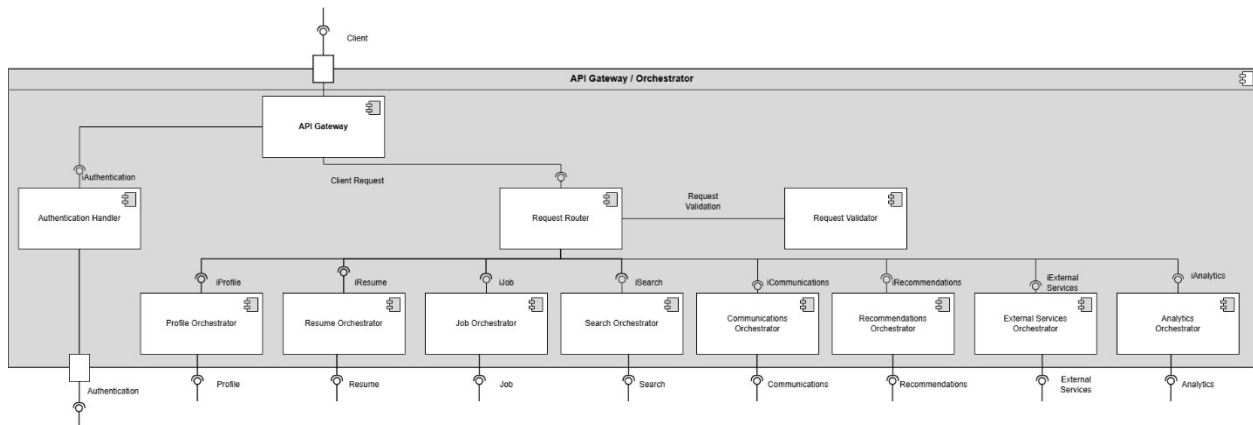
Figure 1.4 – API Gateway / Orchestrator Detail
