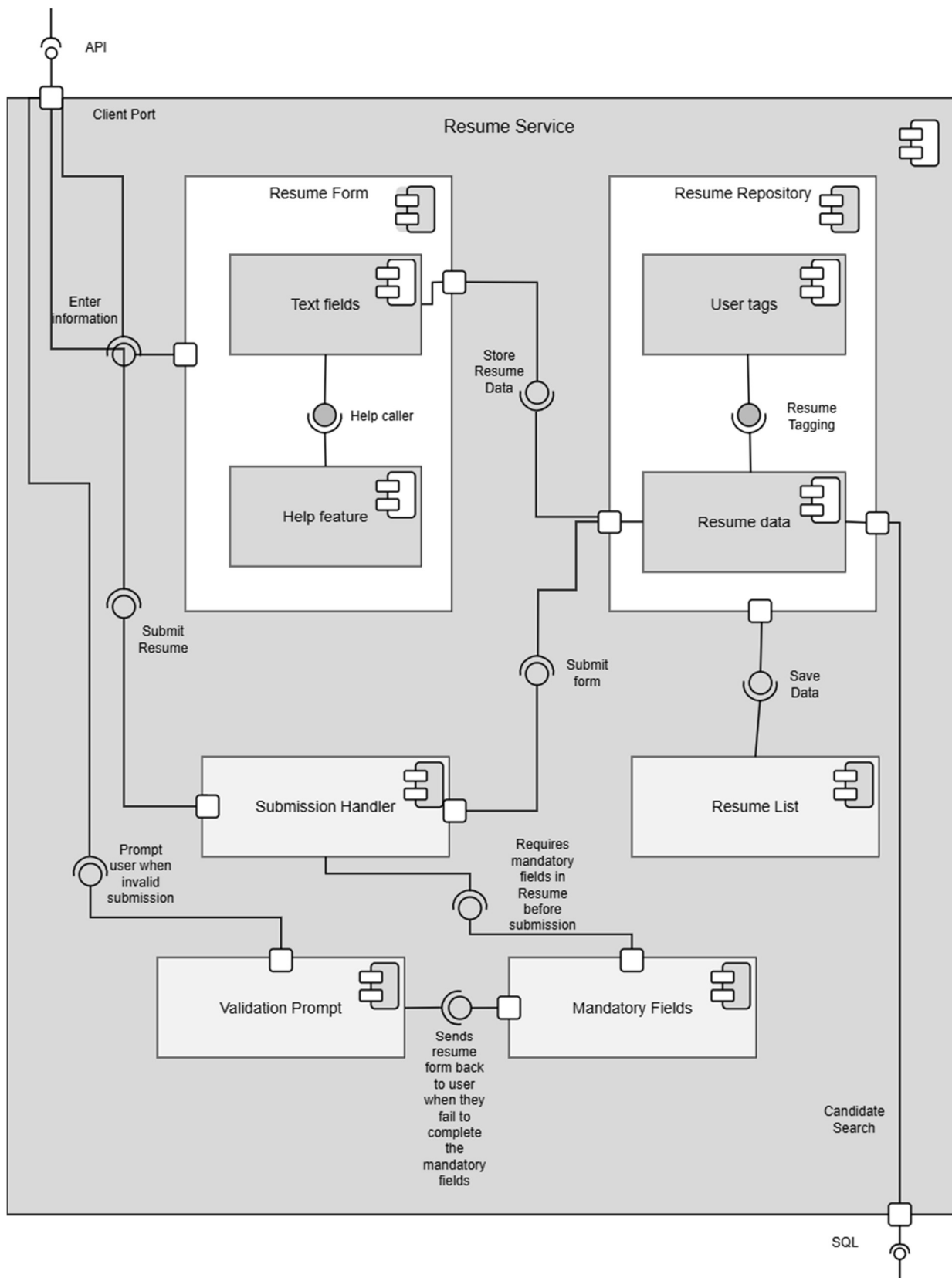
Figure 1.7 – Resume Service
