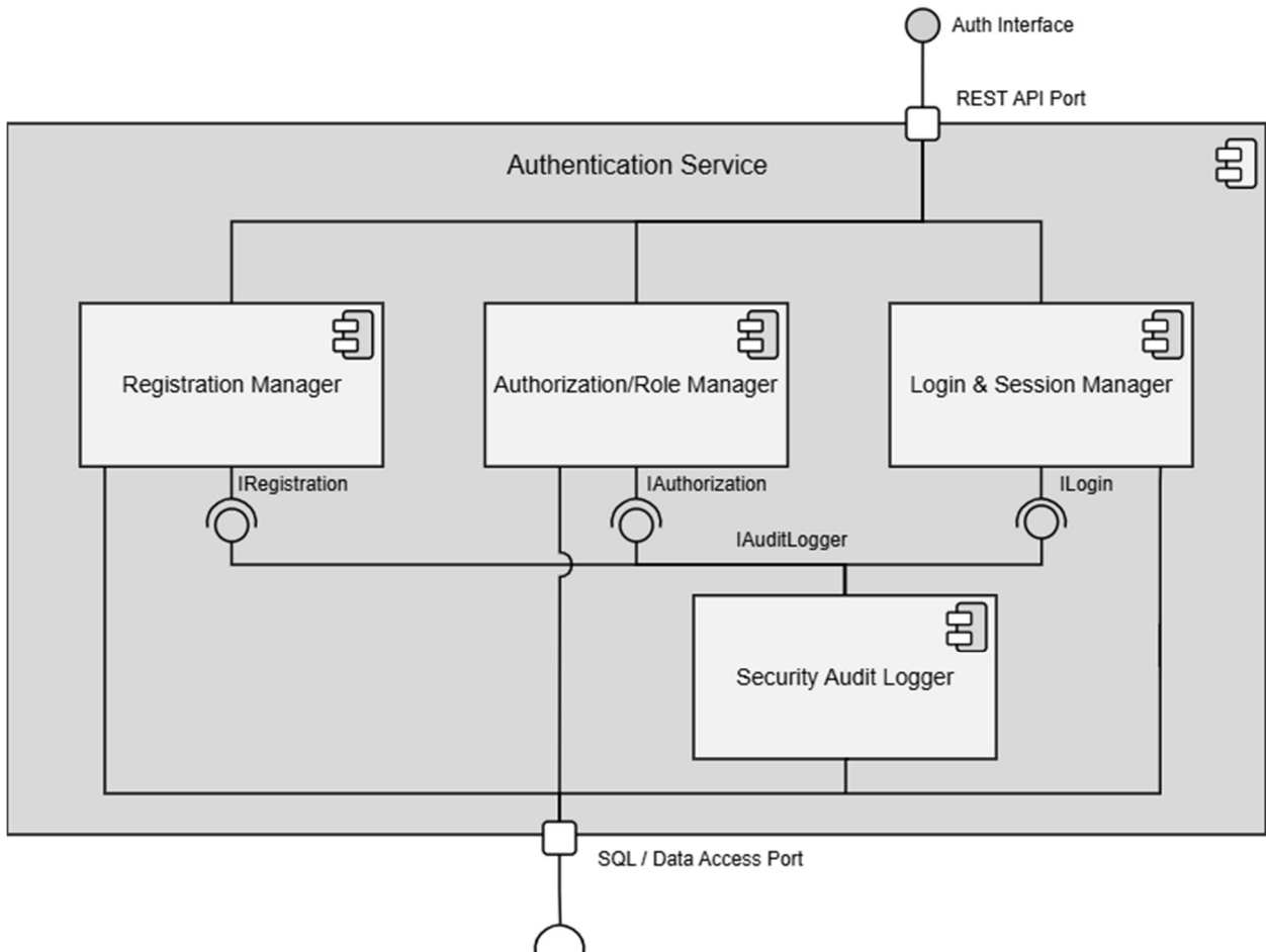
Figure 1.5 – Authentication Service
