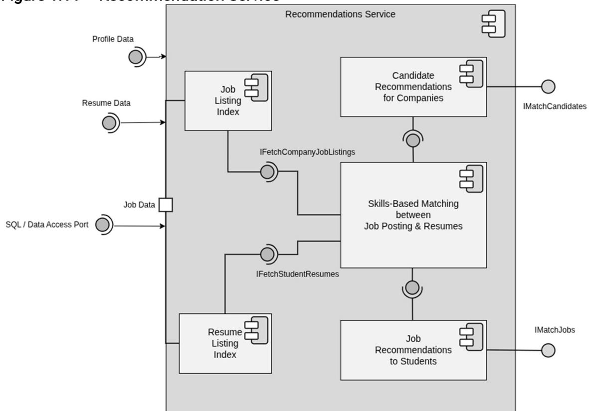
Figure 1.11 – Recommendation Service
