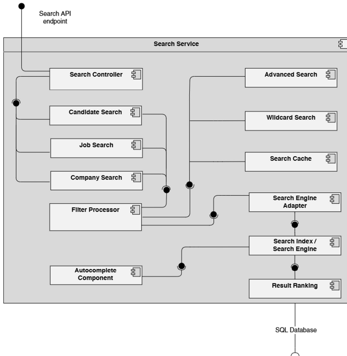
Figure 1.9 – Search Service
