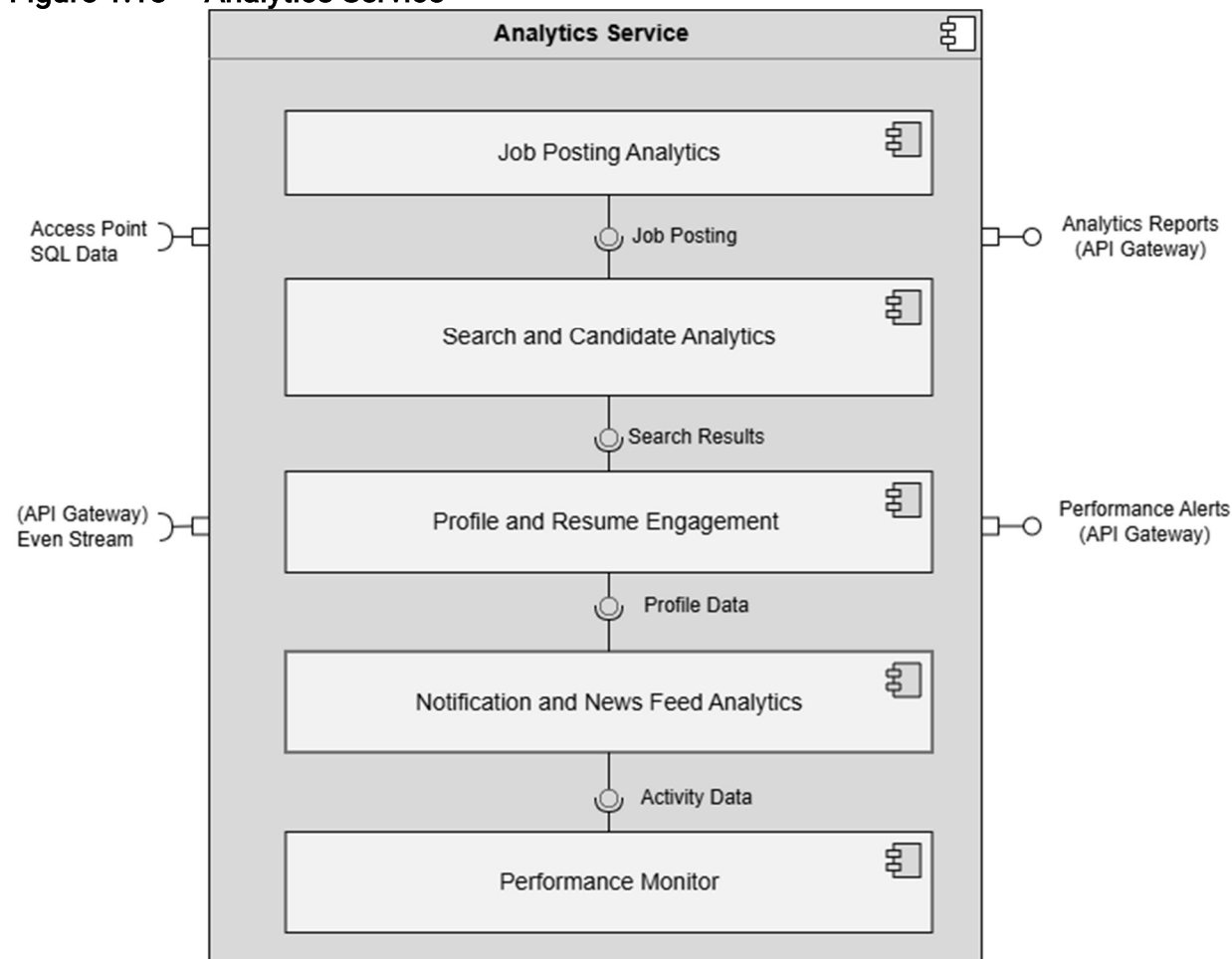
Figure 1.13 – Analytics Service
