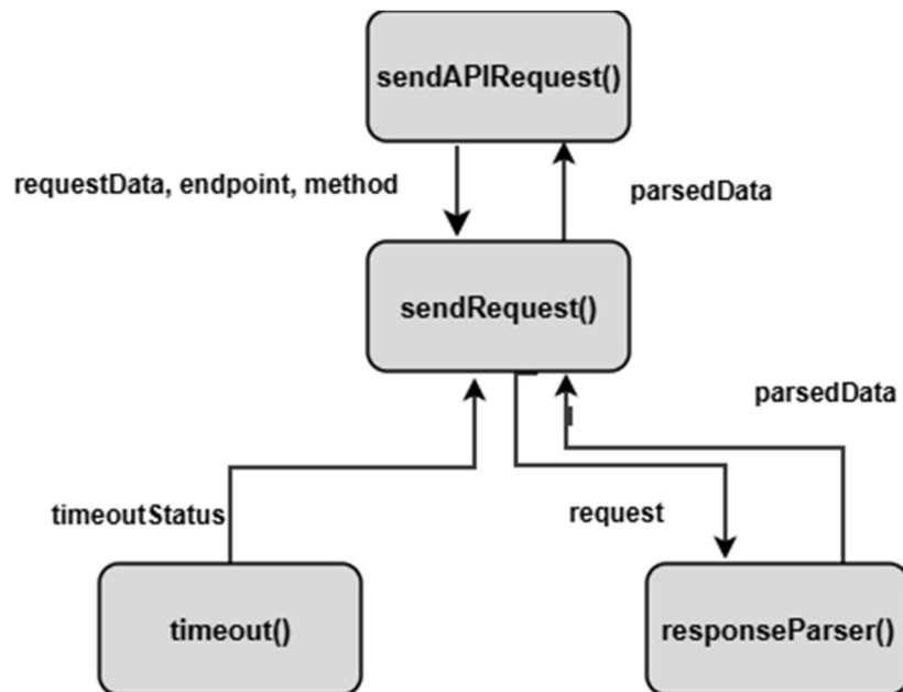
SC Figure 1.2.0.3 &amp; 1.3.0.3 – sendAPIRequest()
