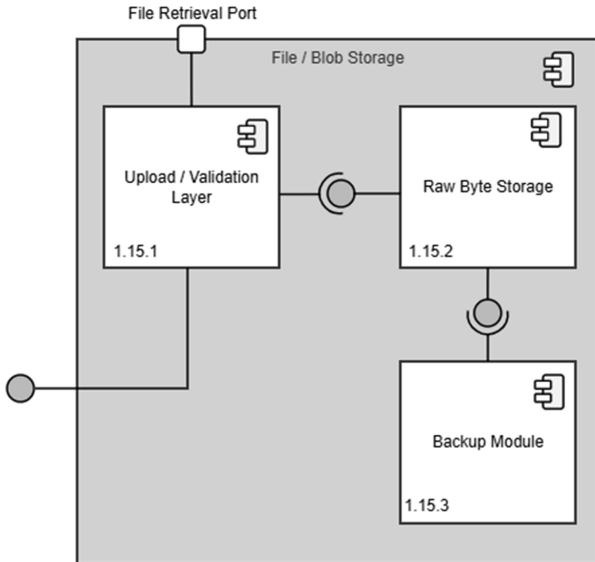
Figure 1.15 — File / Blob Storage Detail
