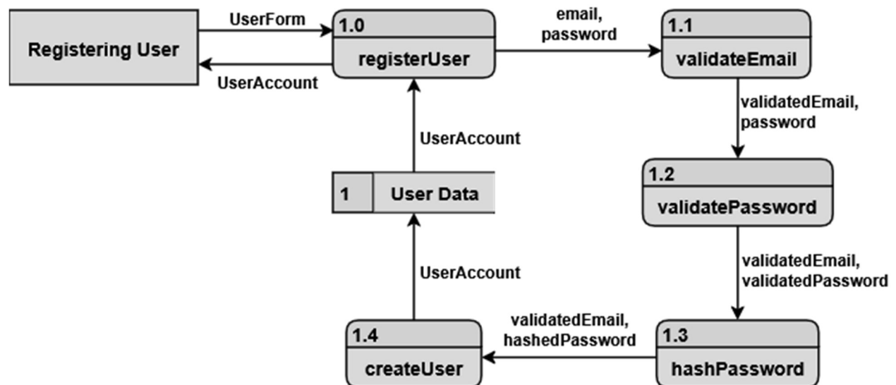
DFD Figure 1.5.0.0.1 — Register User
