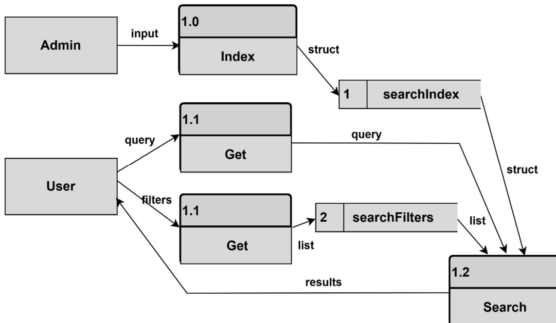
DFD Figure 1.9.0.0.4 – Search Index / Search Engine
