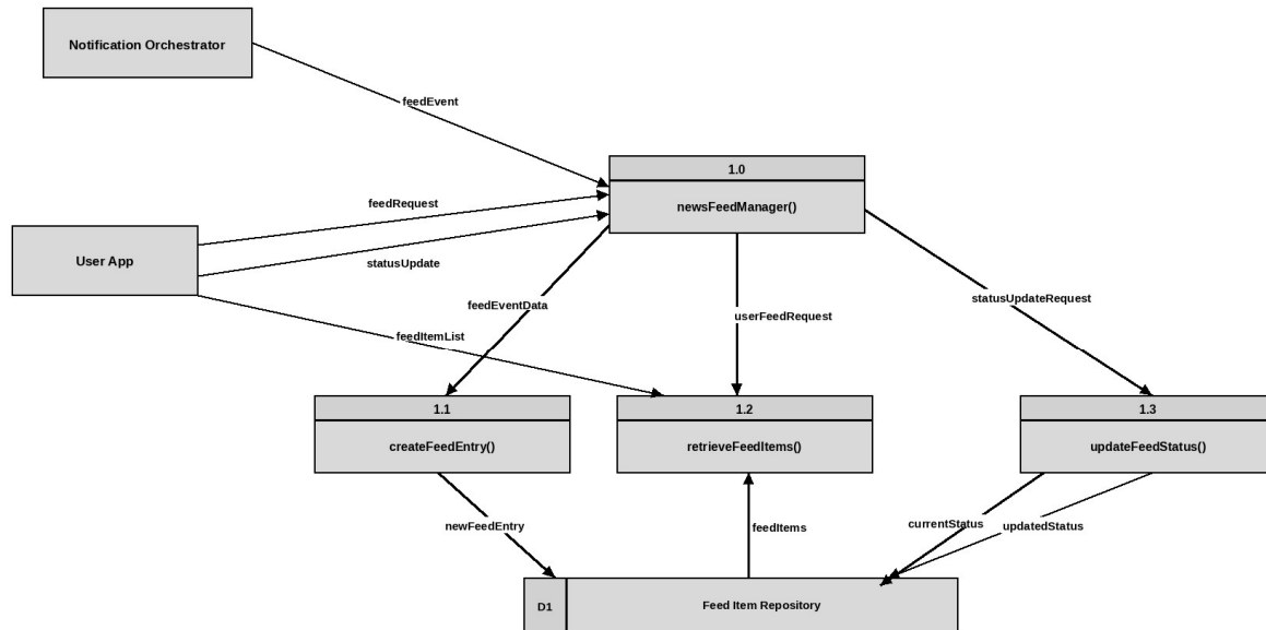
DFD Figure 1.10.0.0.8 — News Feed Manager
