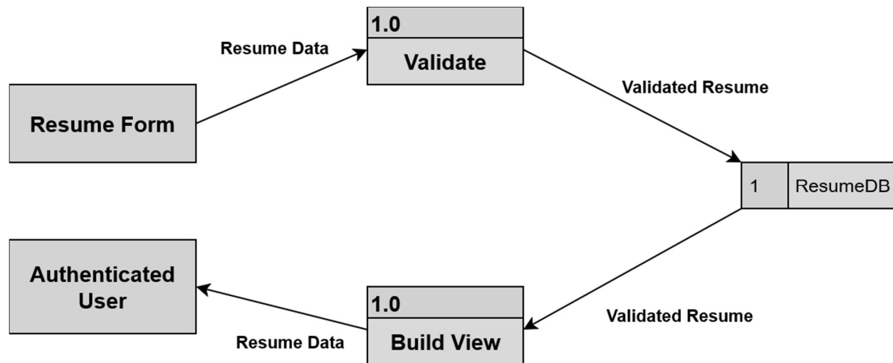
DFD Figure 1.7.0.0.2 — Submission and Storage Workflow
