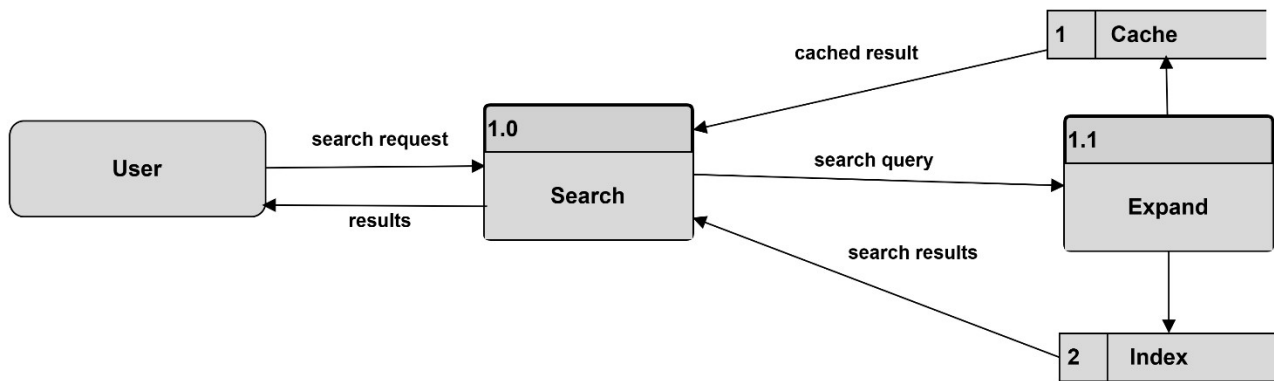
DFD Figure 1.9.0.0.3 – Search Engine Adapter
