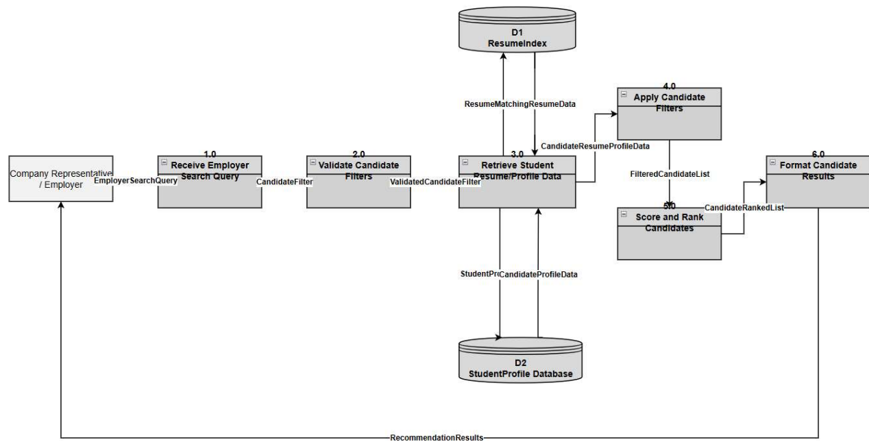
DFD Figure 1.11.0.0.1 – Employer Candidate Search Filter and Recommendation
