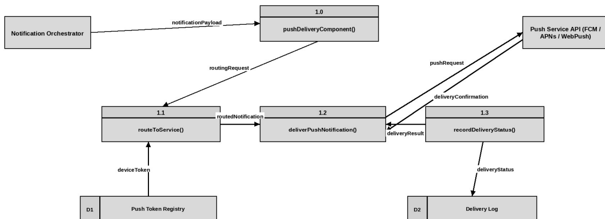
DFD Figure 1.10.0.0.7 — Push Delivery Component
