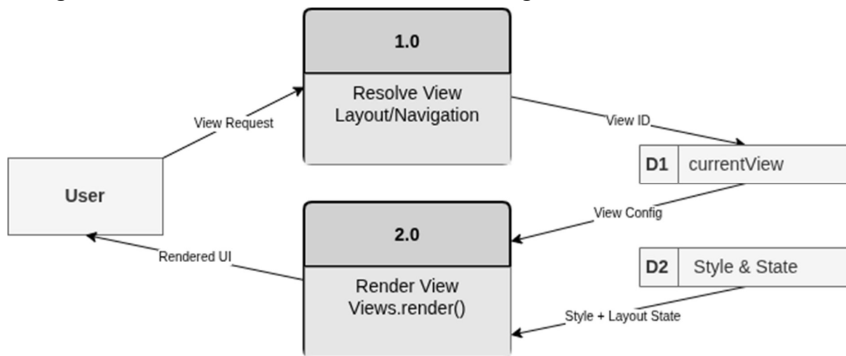
DFD Figure 1.2.0.0.1 & 1.3.0.0.1 – UI View Rendering Data Flow
