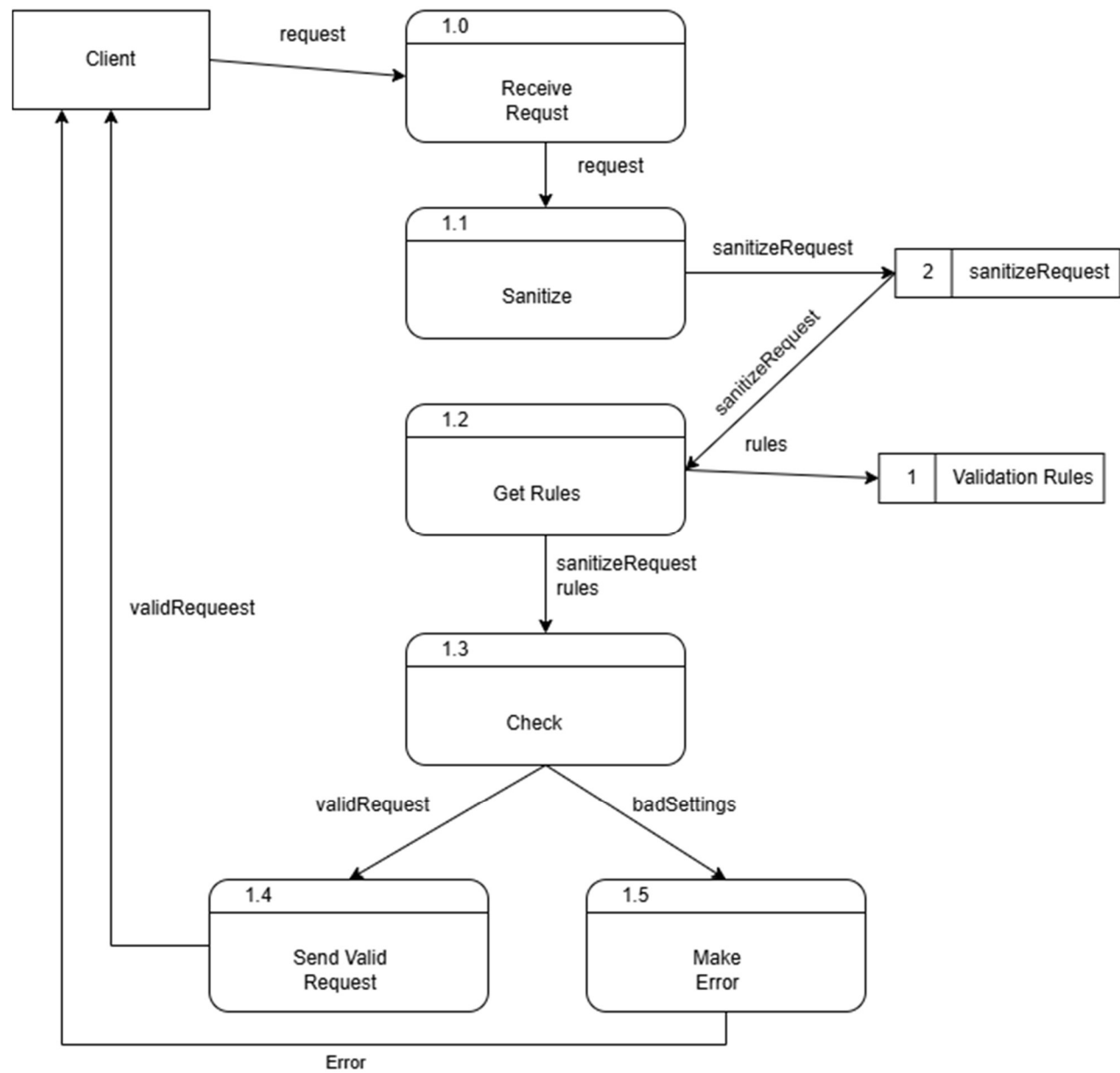
DFD Figure 1.4.0.0.4 – Request Validator
