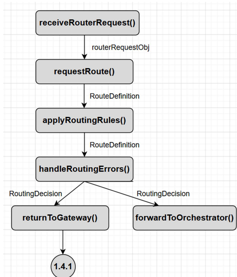
SC Figure 1.4.0.8 – Receive Router Request
