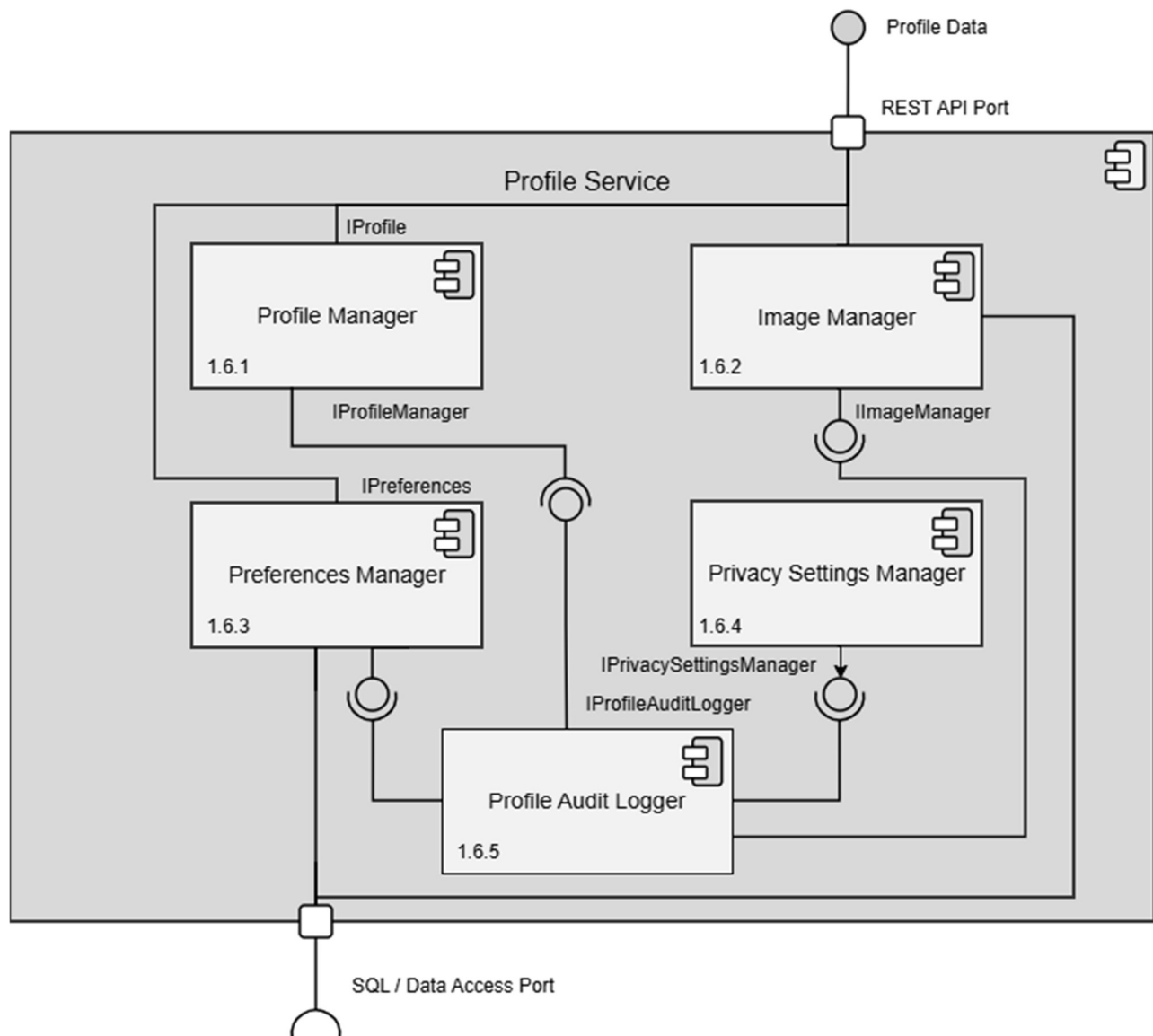
Figure 1.6 — Profile Management Service Detail
