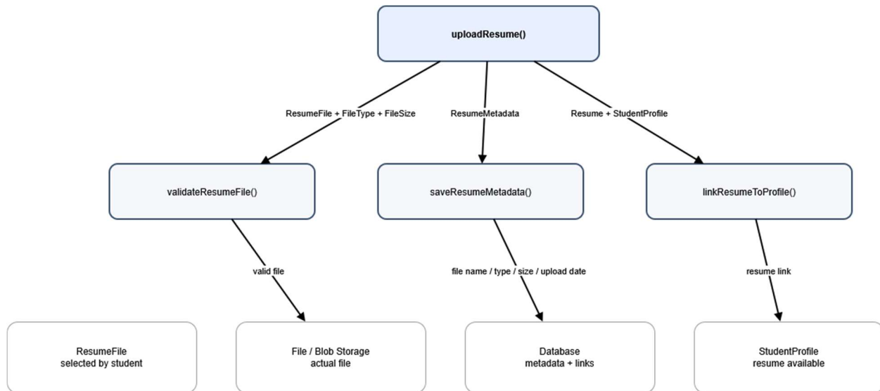
SC Figure 1.7.0.2 — uploadResume()
