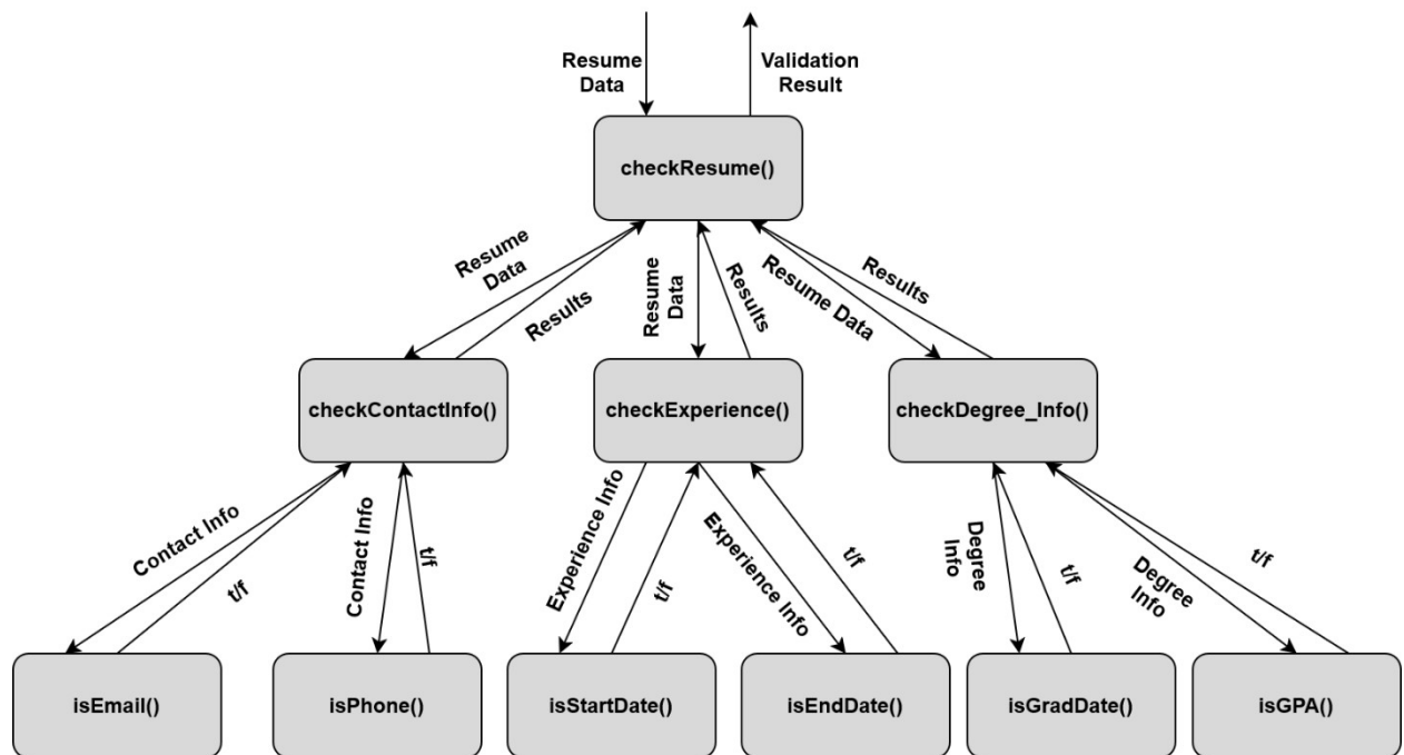
SC Figure 1.7.0.4 — checkResume()
