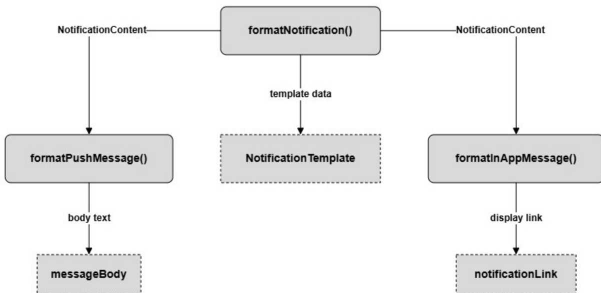
SC Figure 1.10.0.4 – formatNotification()
