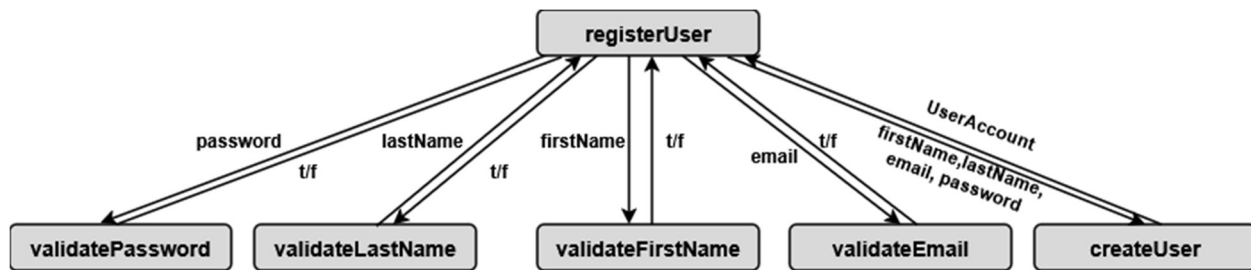
SC Figure 1.6.0.1 — ProfileCreation()
