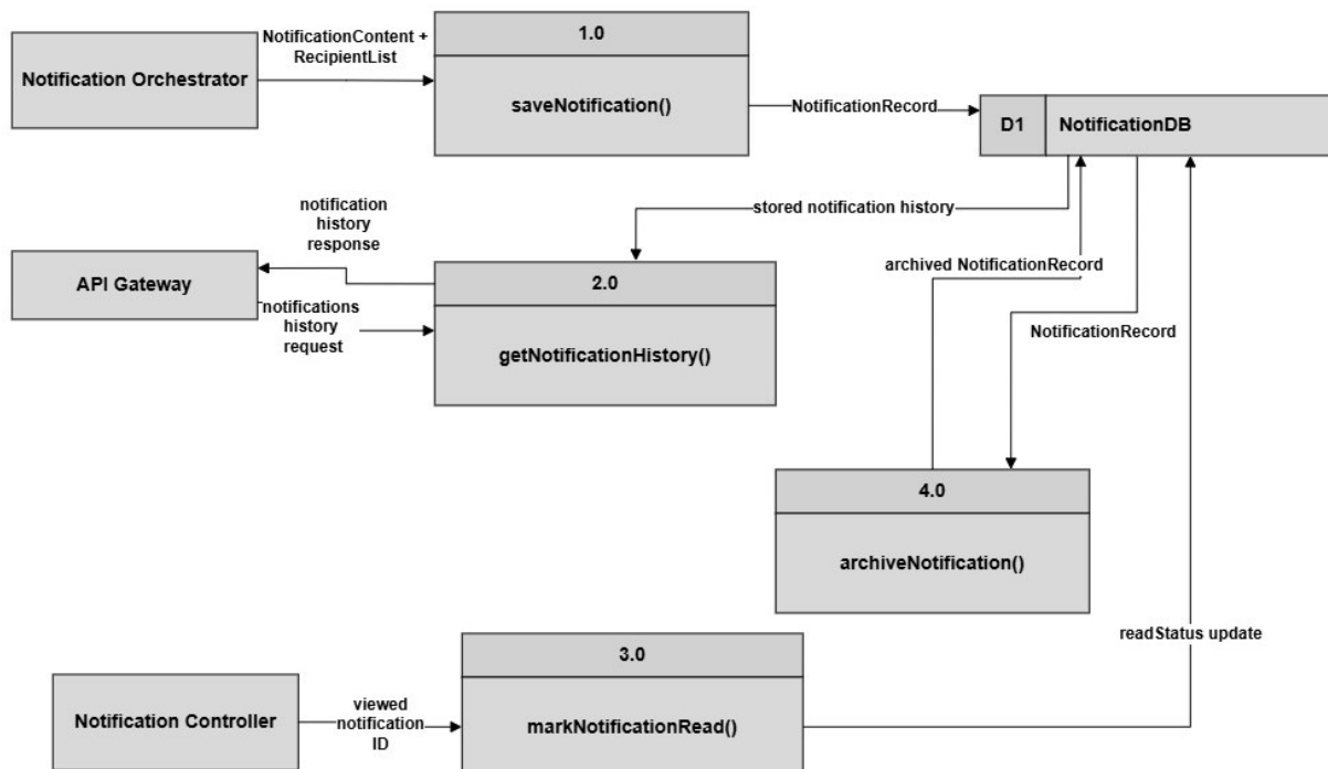
DFD Figure 1.10.0.0.5 – Notification Repository
