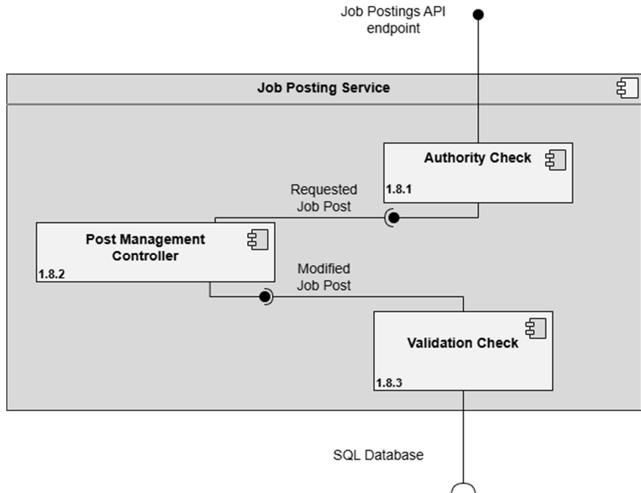
Figure 1.8 — Job Posting Service Detail
