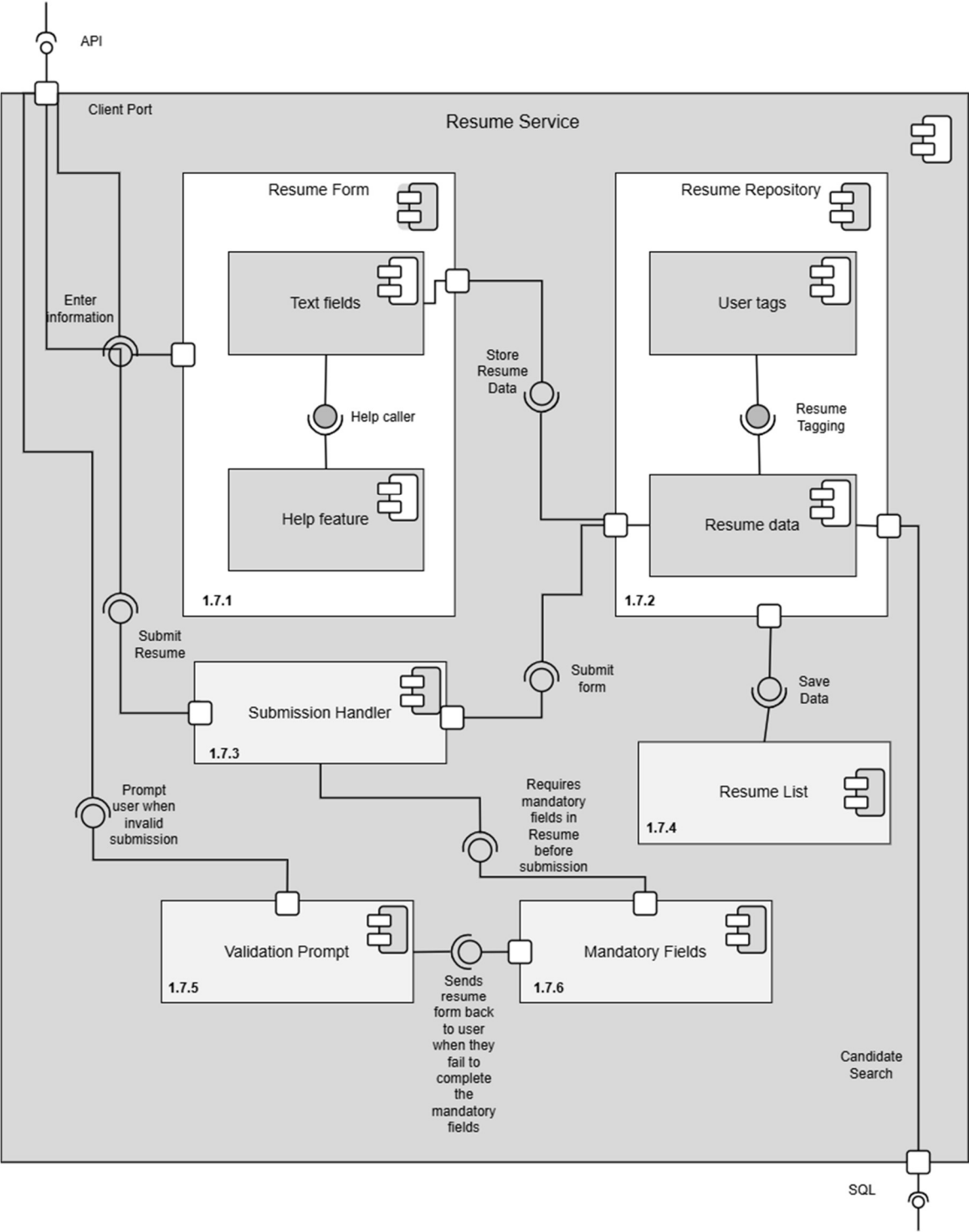
Figure 1.7 — Resume Service Detail
