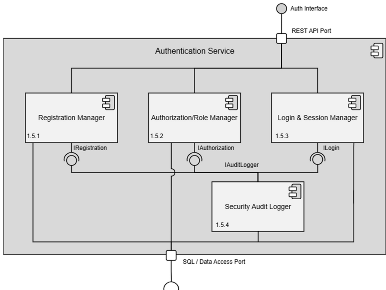
Figure 1.5 — Authentication Service Detail
