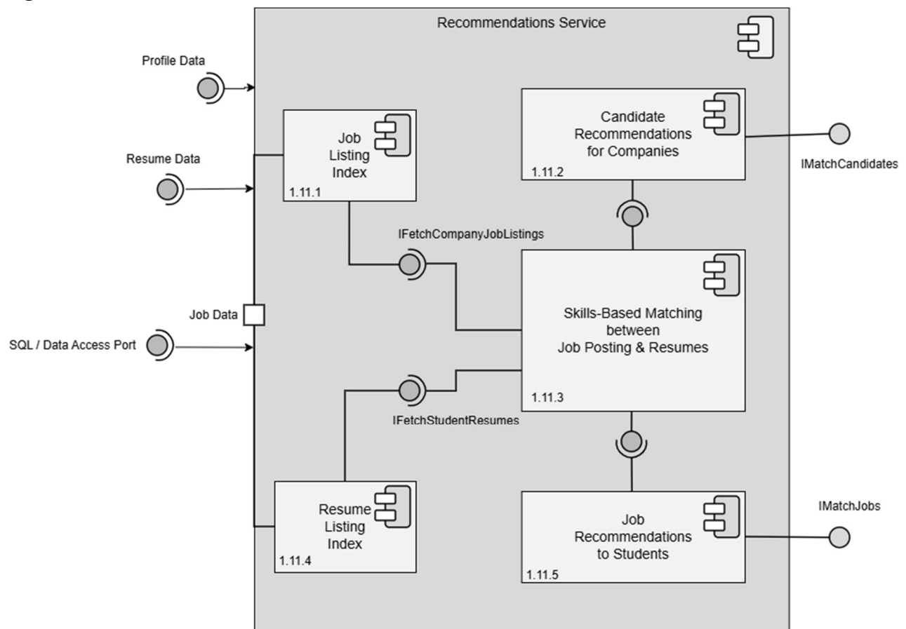
Figure 1.11 — Recommendation Service Detail
