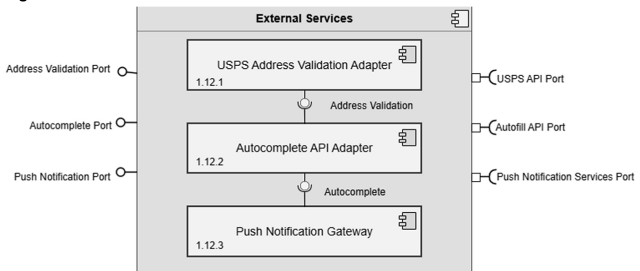
Figure 1.12 — External Services Detail
