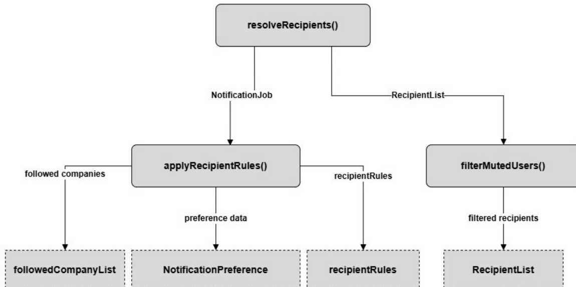
SC Figure 1.10.0.6 – resolveRecipient()
