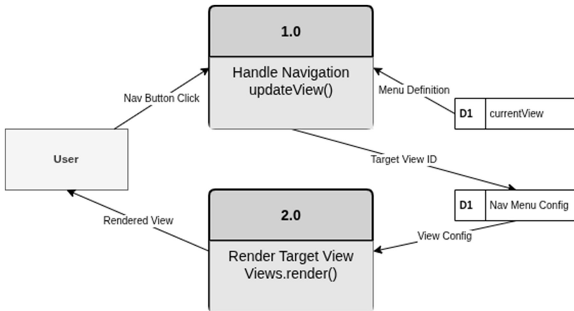
DFD Figure 1.2.0.0.3 &amp; 1.3.0.0.3 – Navigation Selection Data Flow
