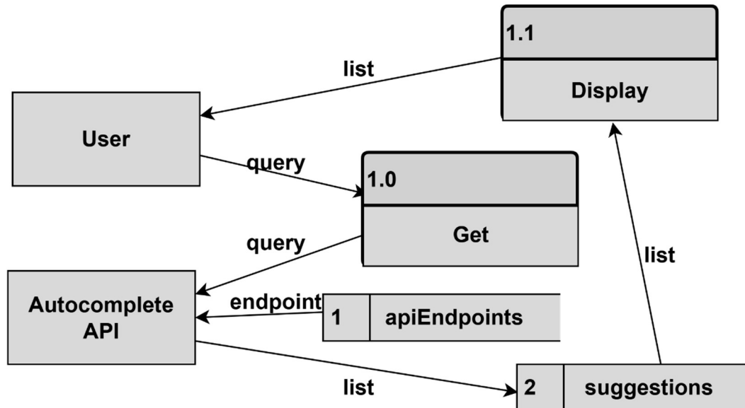
DFD Figure 1.9.0.0.5 – Autocomplete
