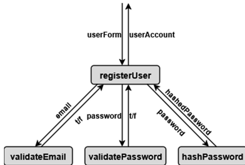
SC Figure 1.5.0.1 — RegisterUser()
