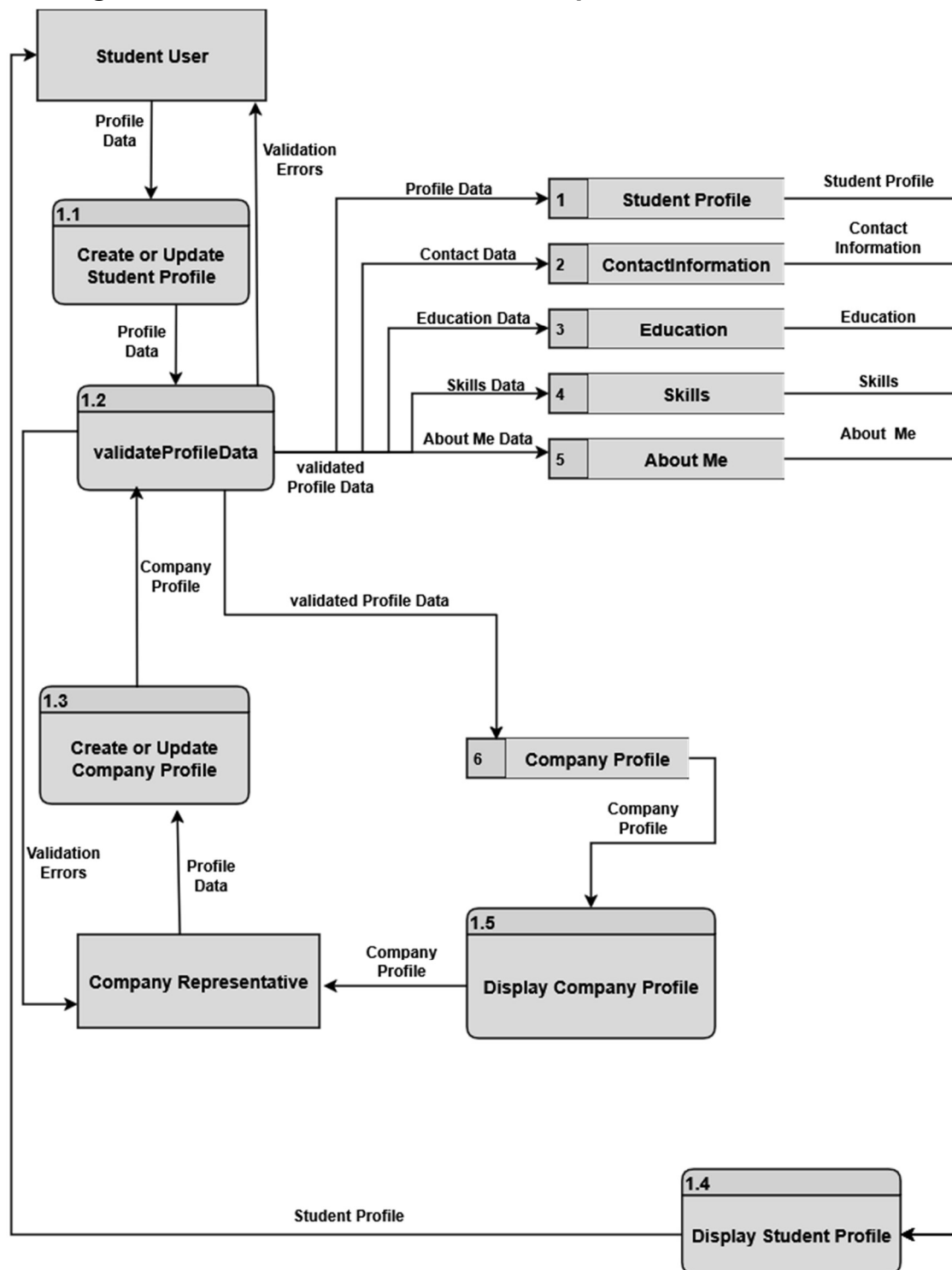
DFD Figure 1.6.0.0.1 - Profile Creation and Update
