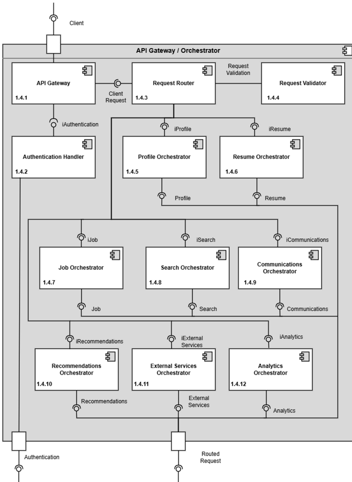
Figure 1.4 — API Gateway / Orchestrator Detail
