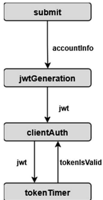
SC Figure 1.5.0.2 — AuthRoleVerification()
