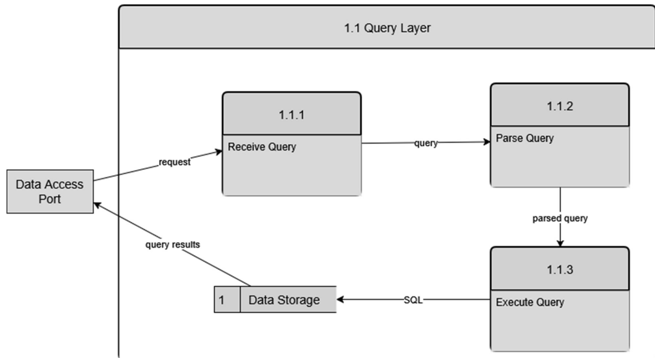
DFD Figure 1.14.0.0.1 – Query Processing and Data Retrieval
