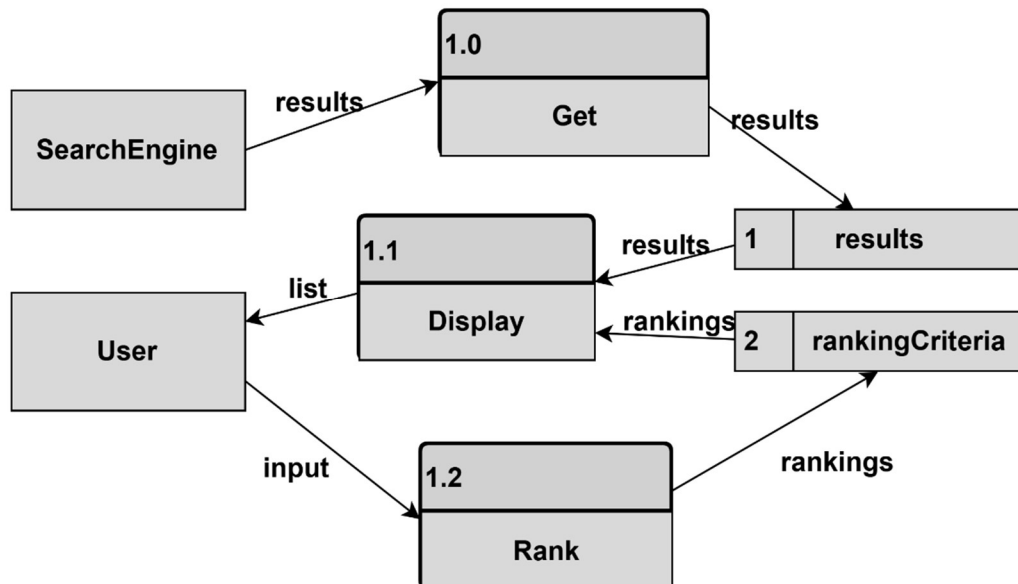
DFD Figure 1.9.0.0.6 – Ranking Results
