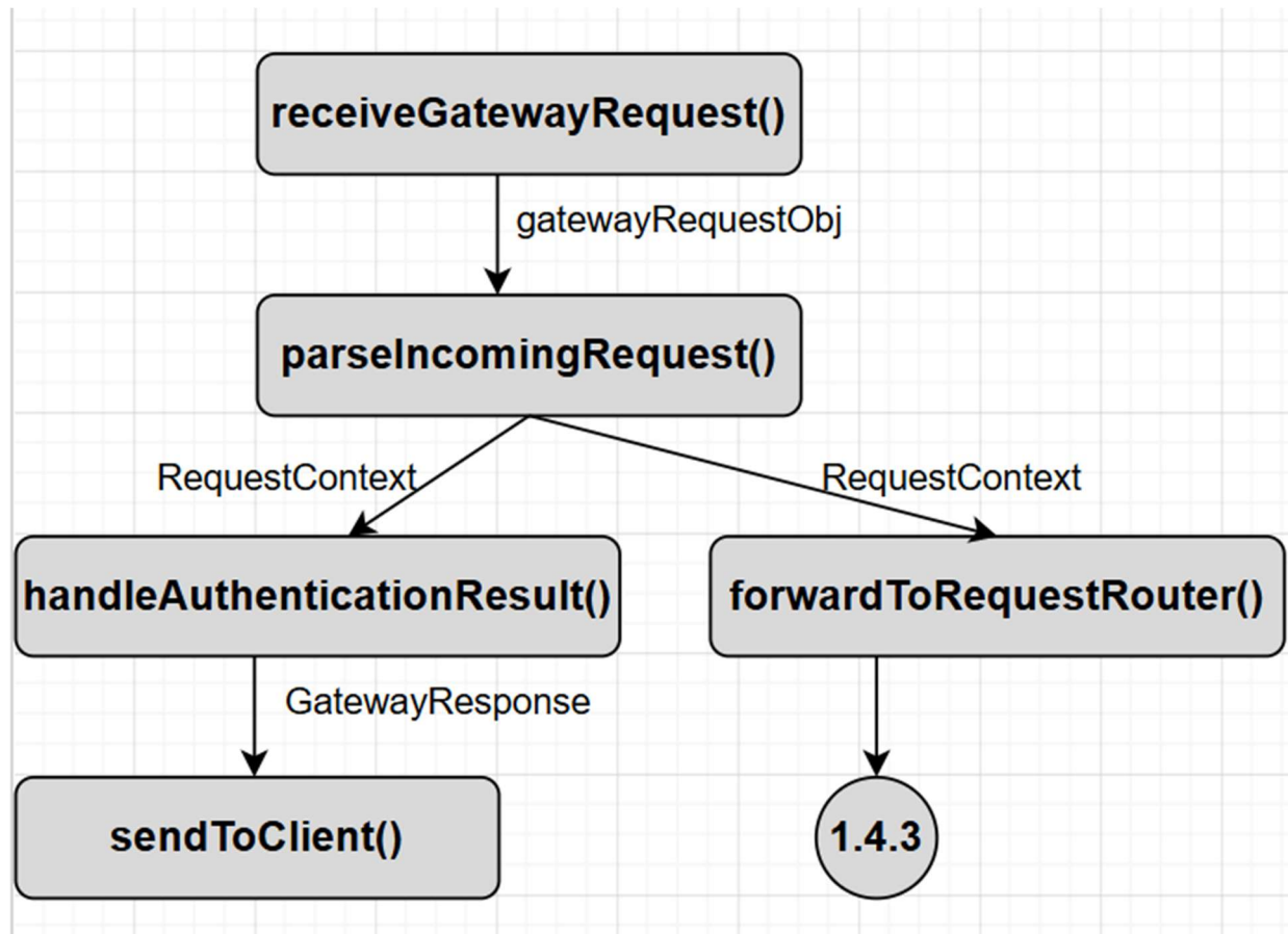
SC Figure 1.4.0.6 – Receive Gateway Request
