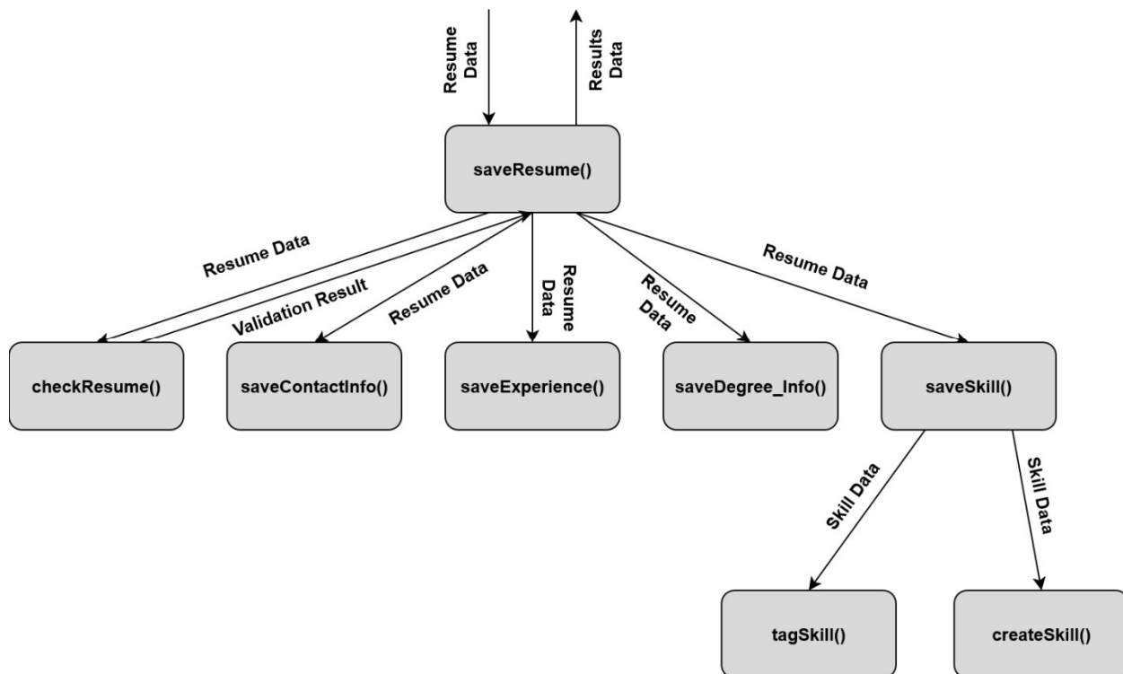
SC Figure 1.7.0.3 — saveResume()
