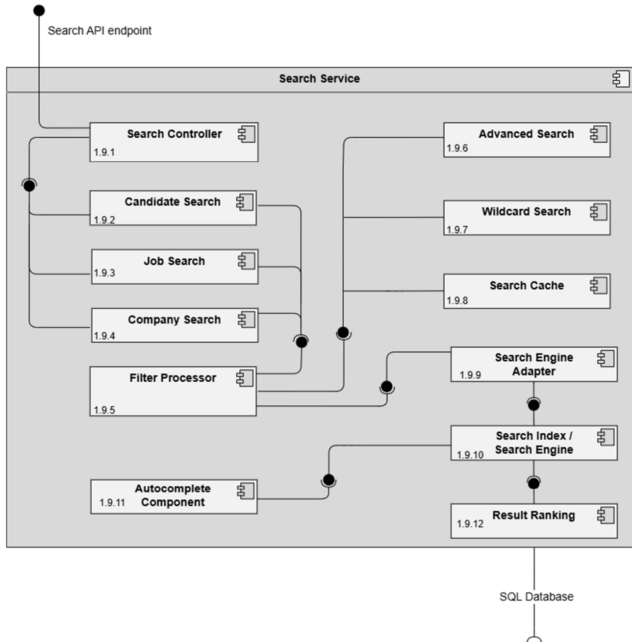
Figure 1.9 — Search Service Detail
