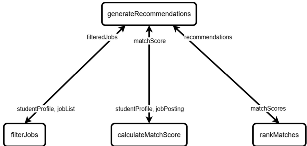
SC Figure 1.11.0.2 — generateRecommendations()
