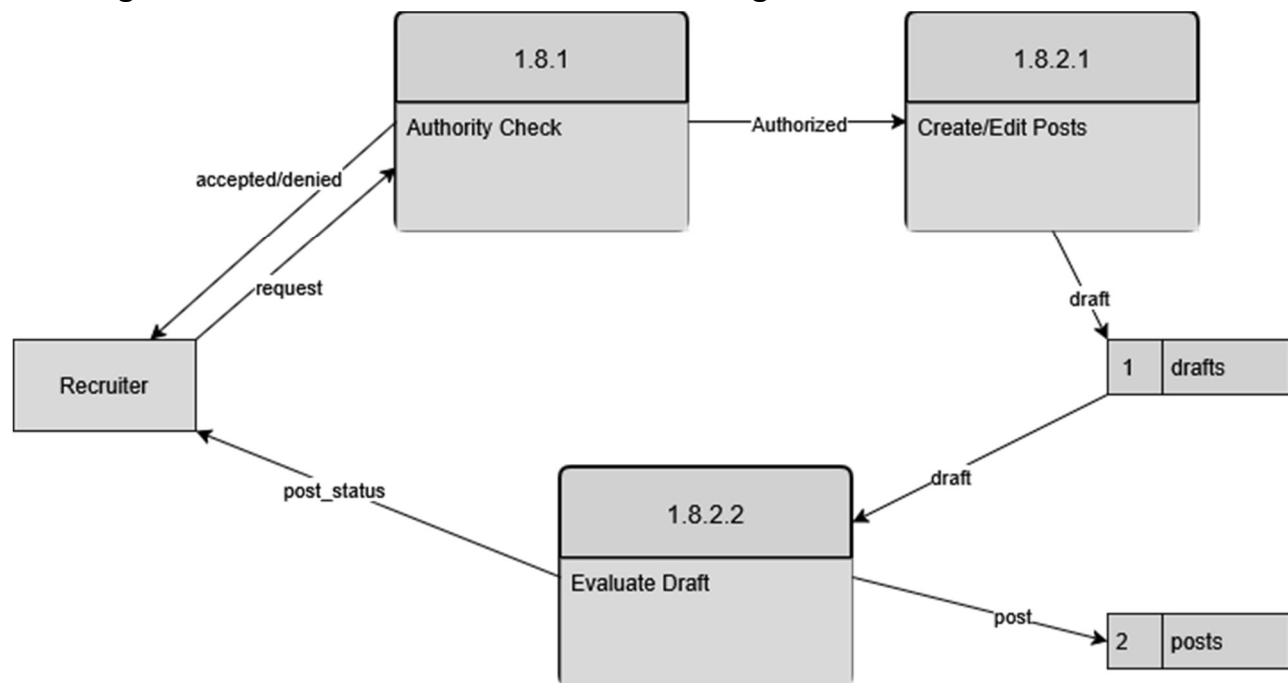
DFD Figure 1.8.0.0.1 – Job Post Creation &amp; Management
