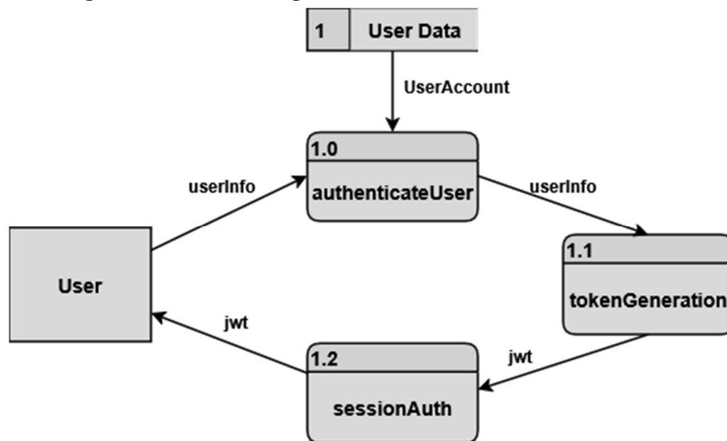
DFD Figure 1.5.0.0.2 — Login Session Validation
