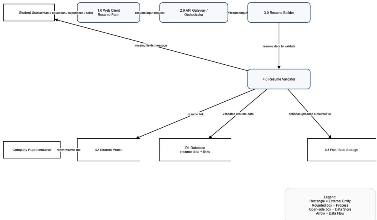
DFD Figure 1.7.0.0.1 — Resume Input and Builder
