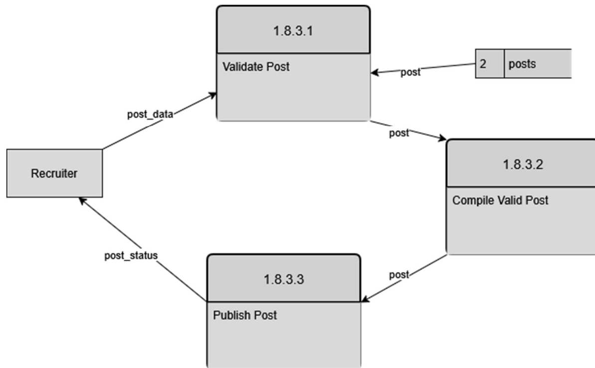
DFD Figure 1.8.0.0.2 – Post Validation &amp; Publishing
