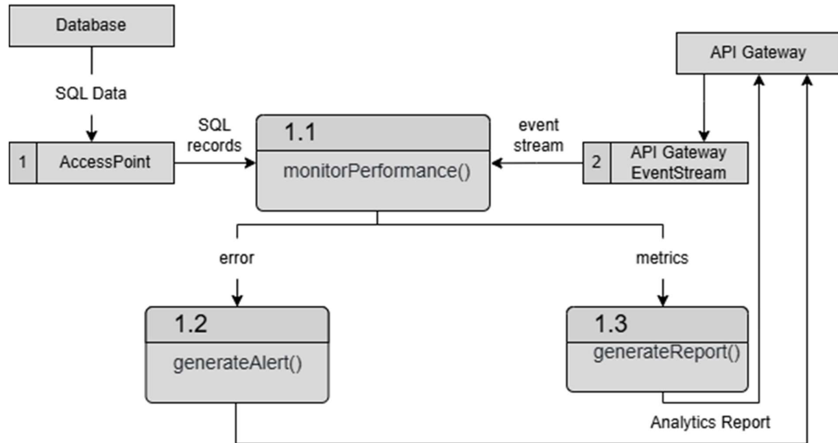
DFD Figure 1.13.0.0.5 – Performance Monitor
