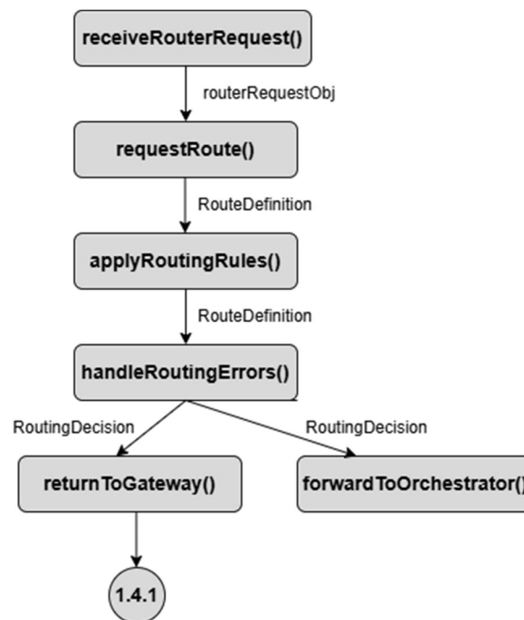
SC Figure 1.4.0.2 – recieveRouterRequest()
