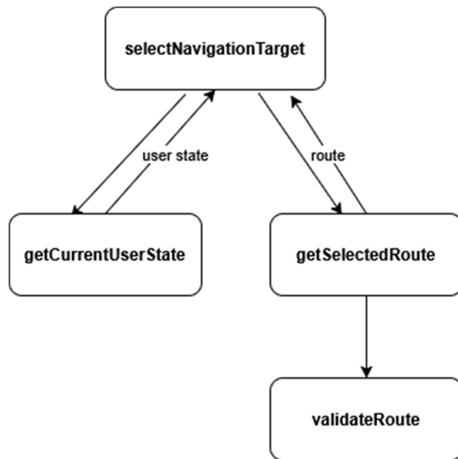
SC Figure 1.2.0.5 &amp; 1.3.0.5 – selectNavigationTarget()
