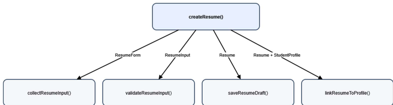
SC Figure 1.7.0.1 — createResume()
