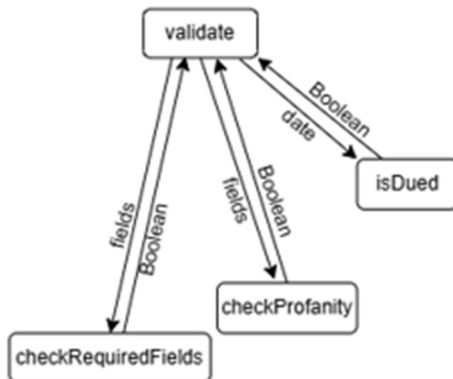
SC Figure 1.8.0.2 – validate()
