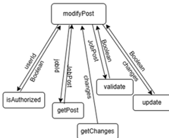
SC Figure 1.8.0.3 – modifyPost()
