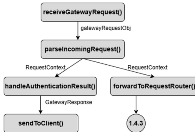
SC Figure 1.4.0.1 – recieveGatewayRequest()
