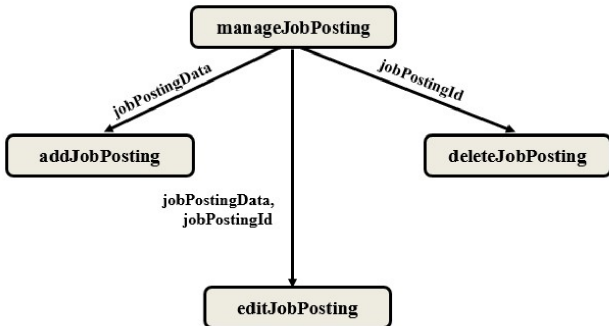
SC Figure 1.13.0.7 — manageJobPosting()
