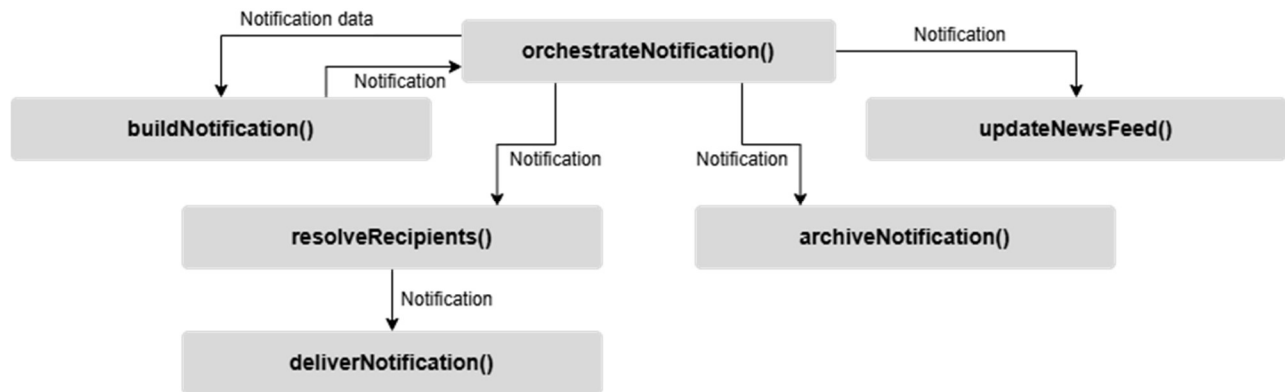
SC Figure 1.10.0.3 – orchestrateNotification()
