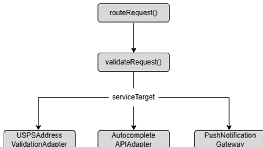
SC Figure 1.4.0.5 – External Services Orchestrator()
