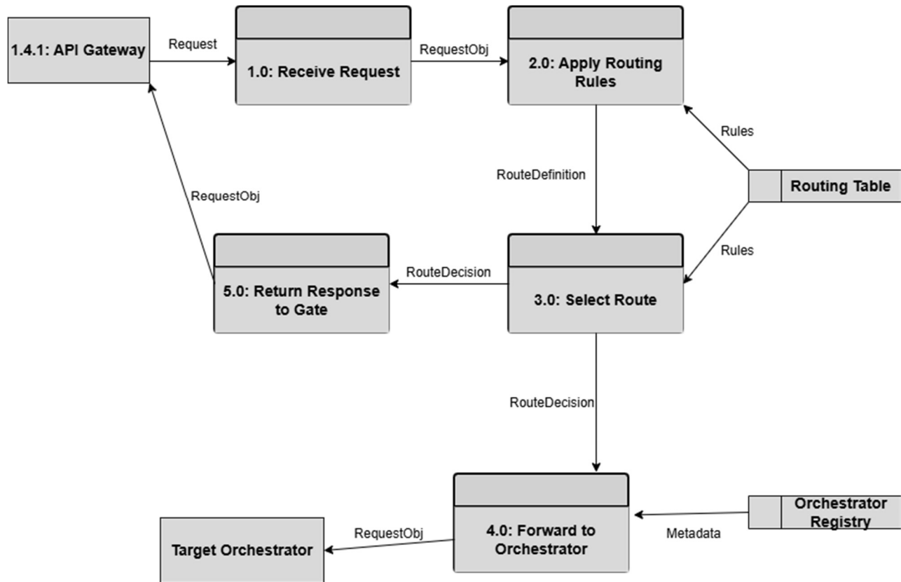
DFD Figure 1.4.0.0.3 – Request Routing
