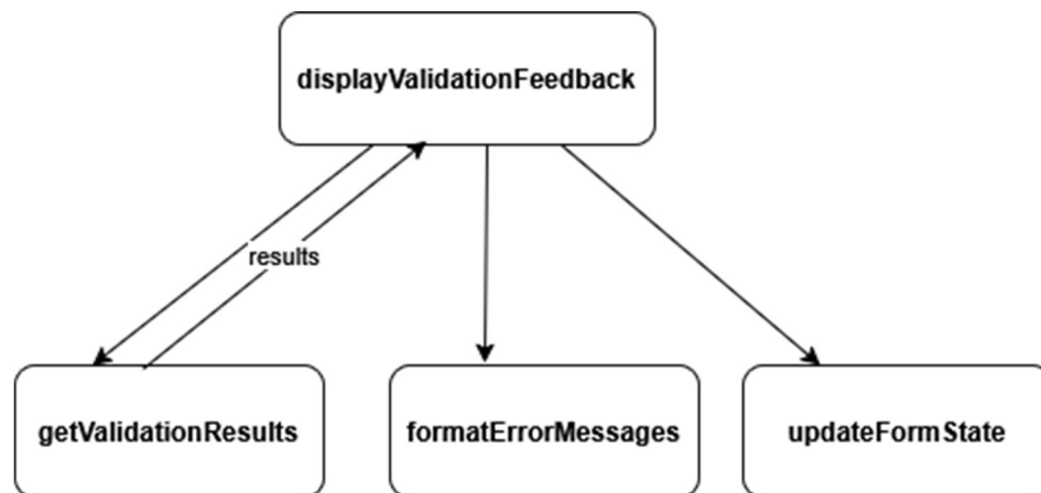
SC Figure 1.2.0.6 &amp; 1.3.0.6 – displayValidationFeedback()
