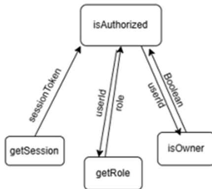
SC Figure 1.8.0.4 – isAuthorized()
