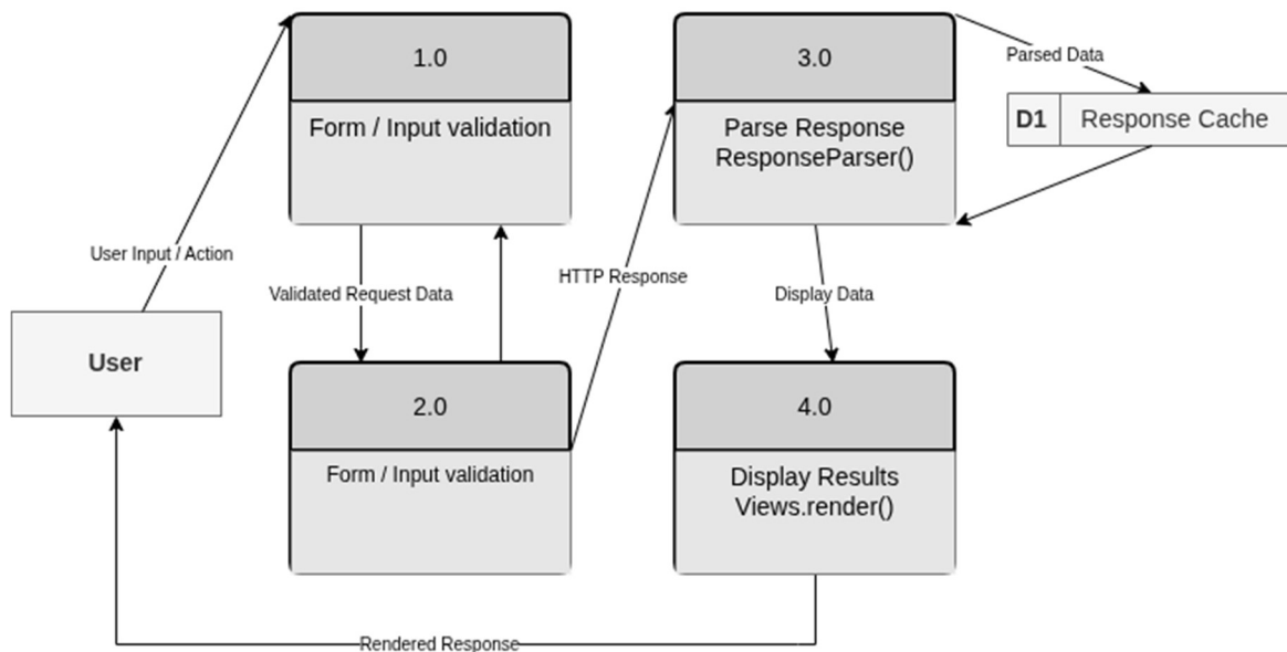
DFD Figure 1.2.0.0.4 &amp; 1.3.0.0.4 – Client API Response Display Data Flow
