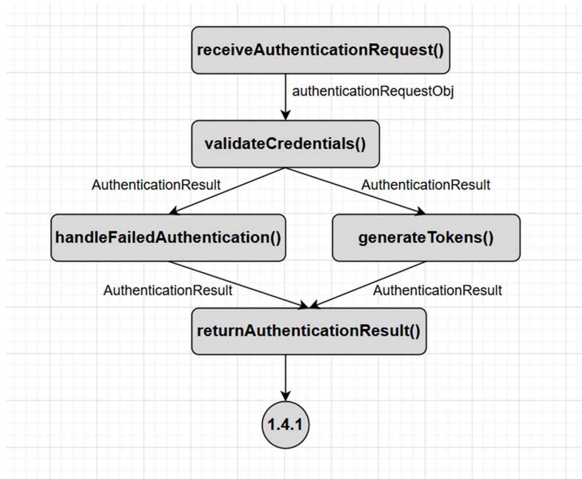
SC Figure 1.4.0.7 – Receive Authentication Request
