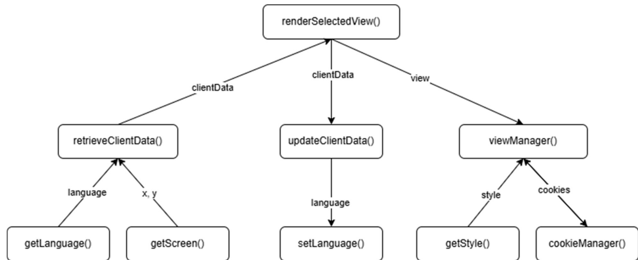
SC Figure 1.2.0.1 &amp; 1.3.0.1 – renderSelectedView()
