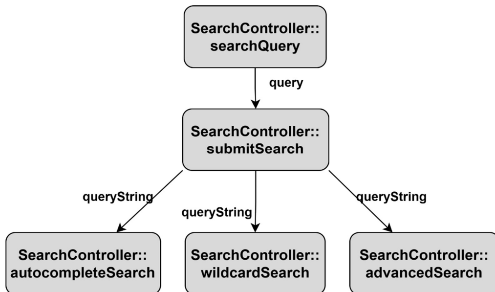
SC Figure 1.9.0.1 – SearchQuery()
