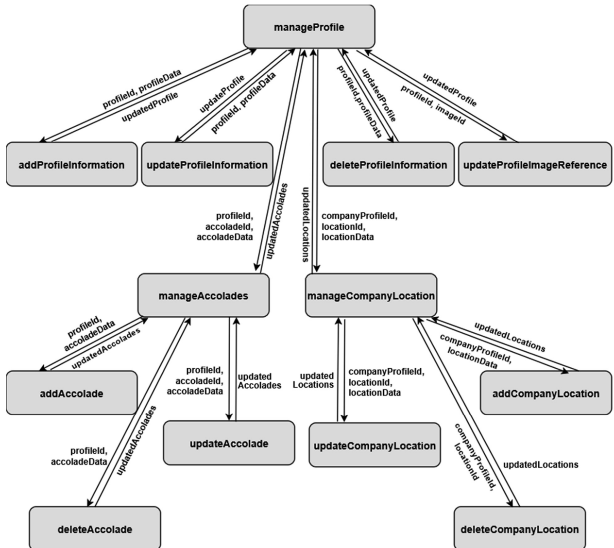
SC Figure 1.6.0.2 — ProfileInformationManager()
