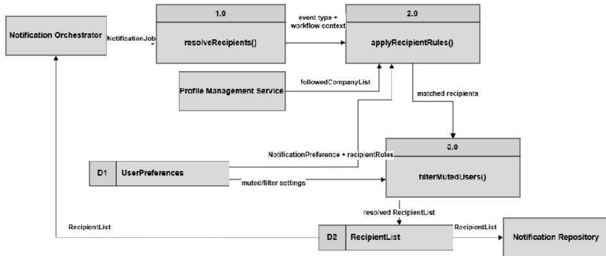
DFD Figure 1.10.0.0.6 – Recipient Resolver
