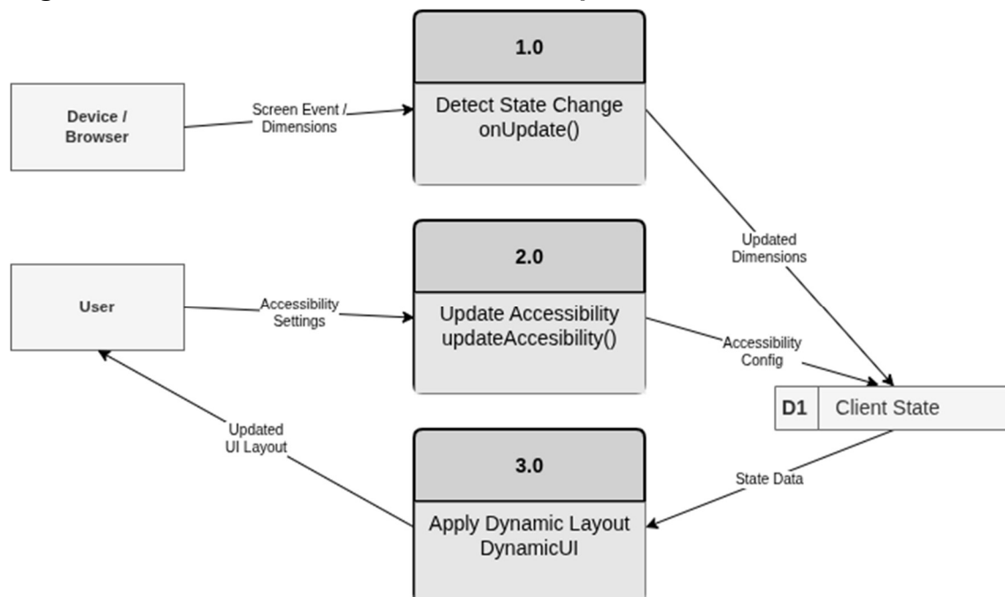
DFD Figure 1.2.0.0.2 & 1.3.0.0.2 – Client State Update Data Flow
