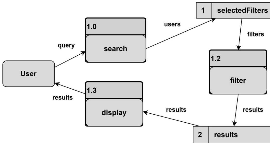
DFD Figure 1.9.0.0.1 – Job Search
