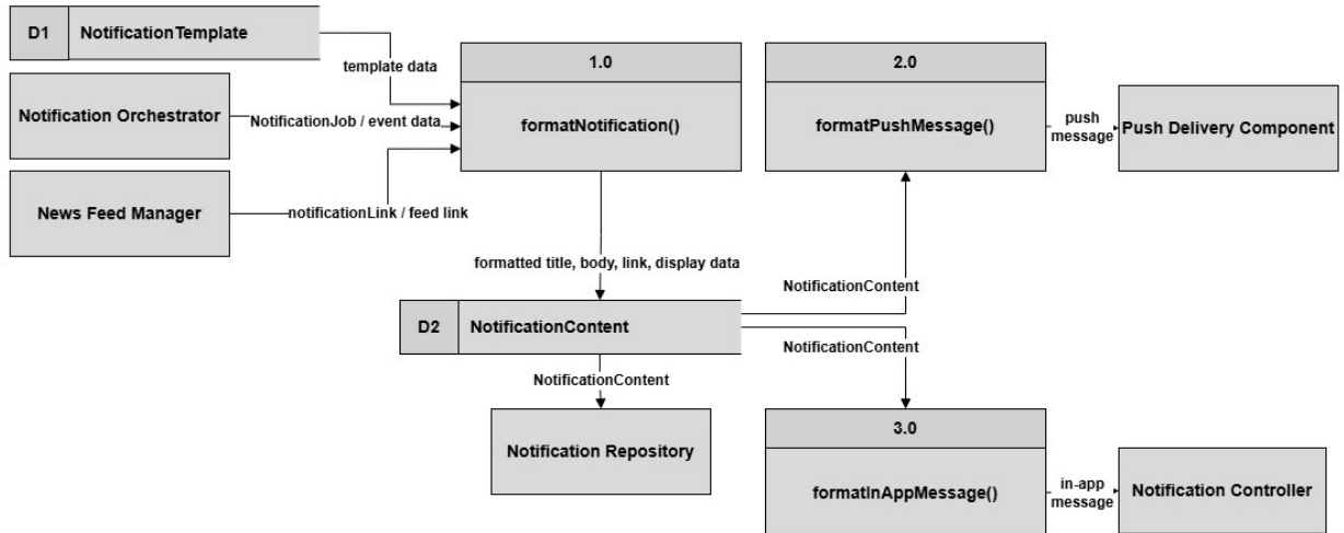
DFD Figure 1.10.0.0.4 – Notification Formatter
