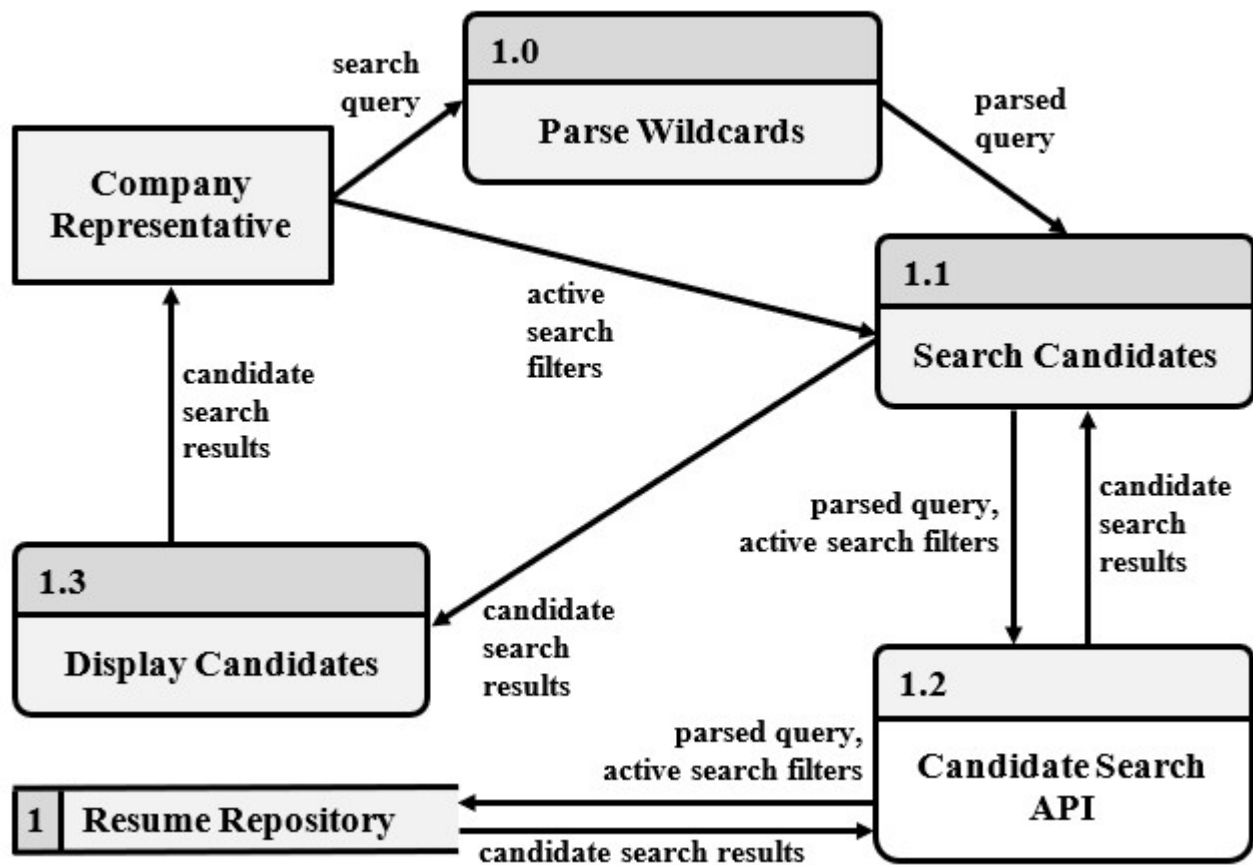
DFD Figure 1.13.0.0.6 — Candidate Search Workflow
