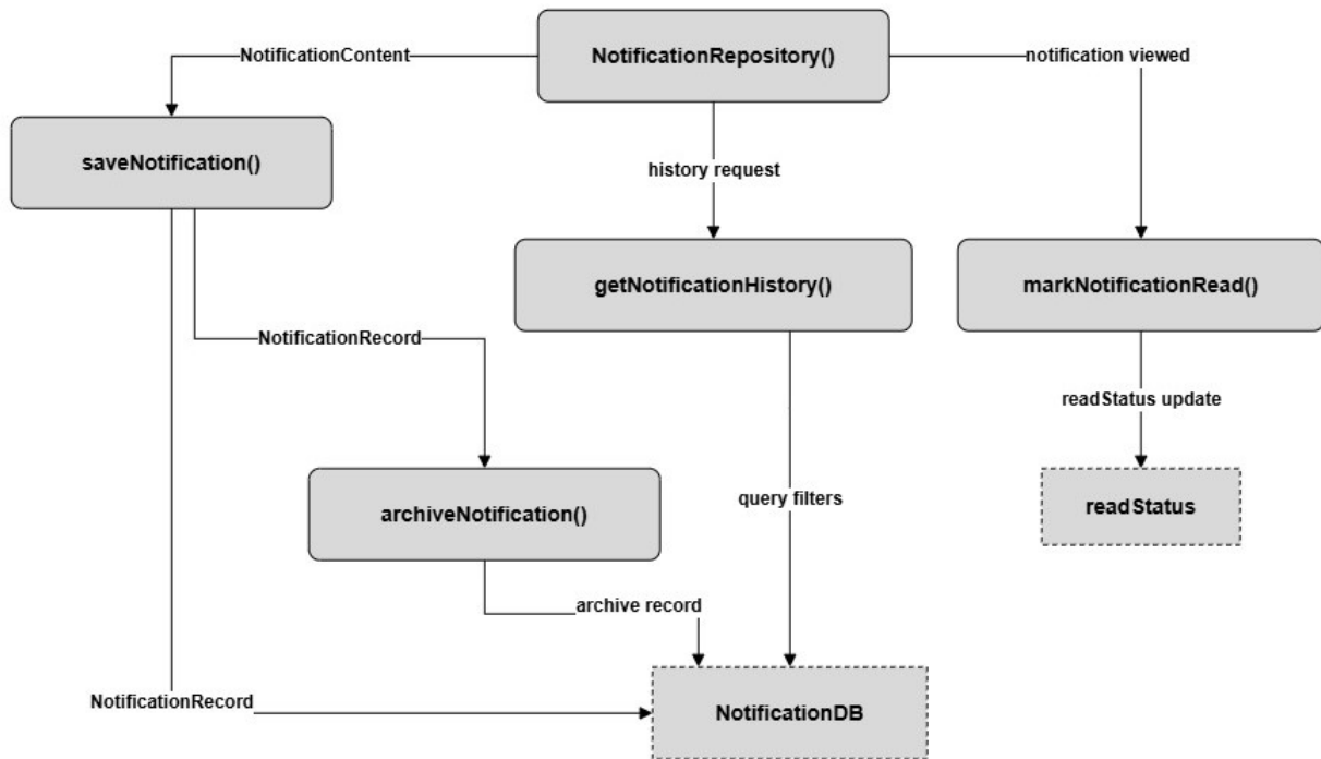
SC Figure 1.10.0.5 – notificationRepository()
