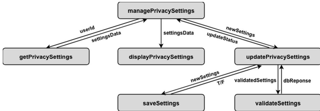
SC Figure 1.6.0.4 — ManagePrivacySettings()
