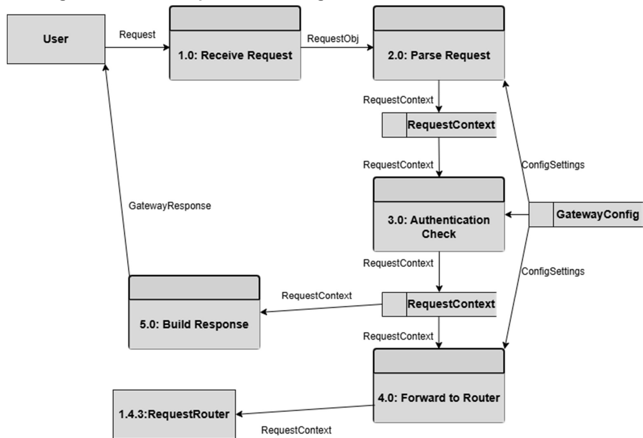
DFD Figure 1.4.0.0.1 –Request Processing
