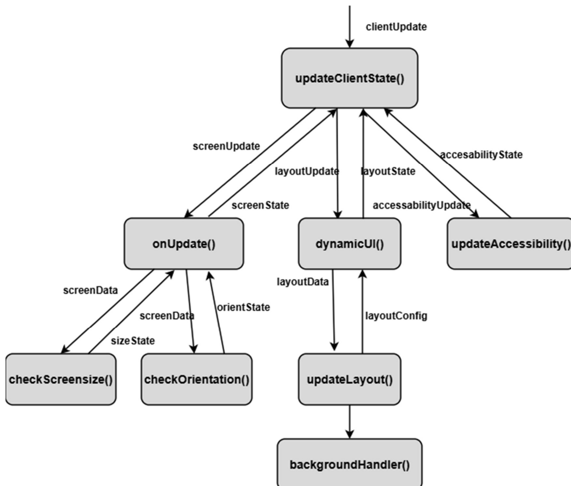
SC Figure 1.2.0.4 &amp; 1.3.0.4 – updateClientState()
