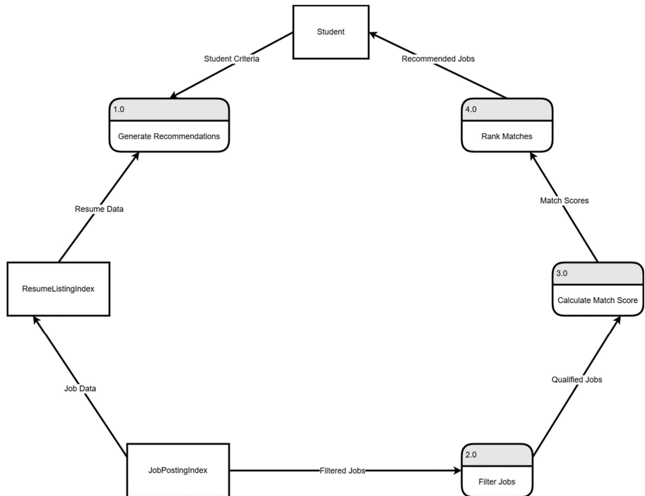
DFD Figure 1.11.0.0.2 – Student-to-Job Matching
