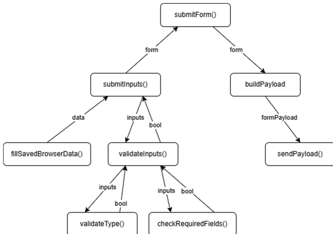
SC Figure 1.2.0.2 &amp; 1.3.0.2 – submitForm()
