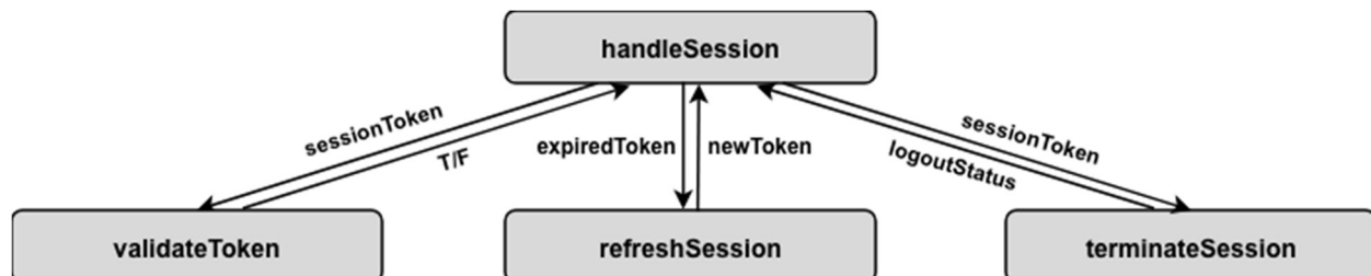
SC Figure 1.5.0.5 — HandleSession()
