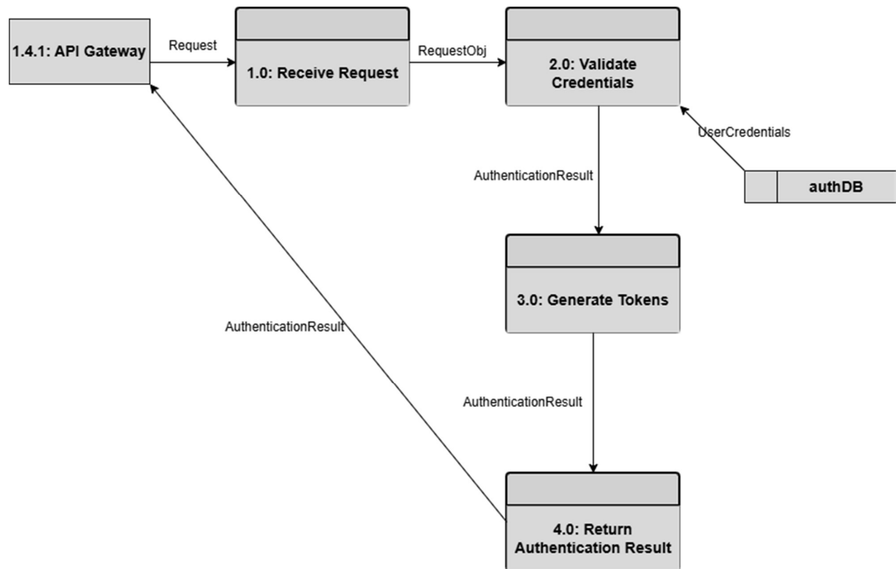
DFD Figure 1.4..0.0.2 – Authentication Validation
