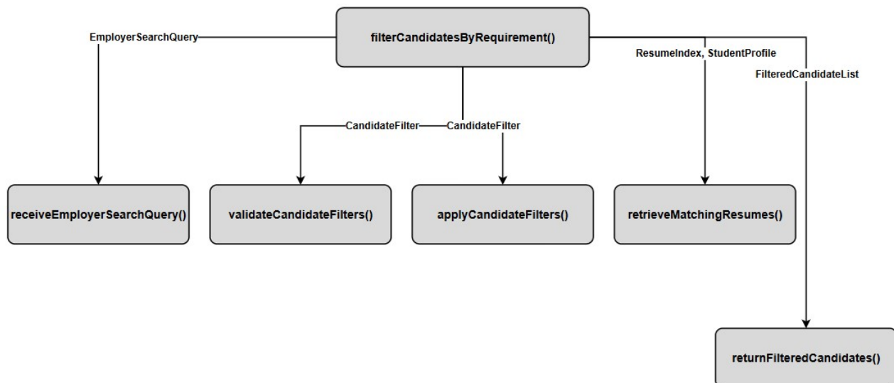
SC Figure 1.11.0.1 — filterCandidatesByRequirement()
