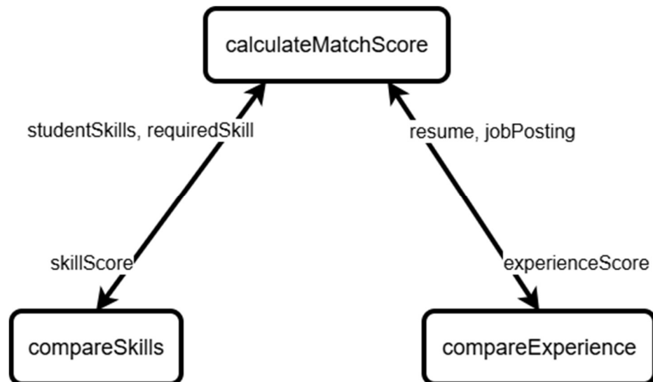
SC Figure 1.11.0.3 — calculateMatchScore()
