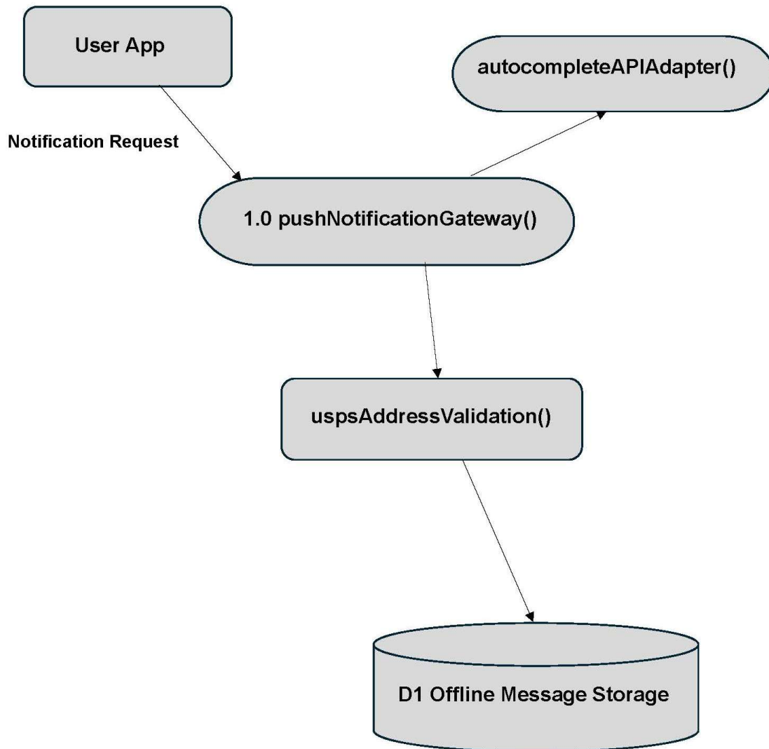
DFD Figure 1.12.0.0.3 — Push Notification Gateway
