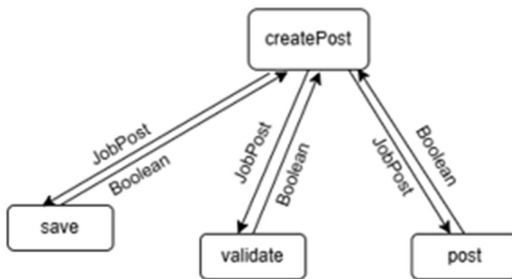
SC Figure 1.8.0.1 – createPost()
