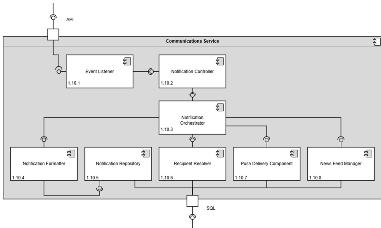
Figure 1.10 — Communication Services (Notifications + News Feed) Detail
