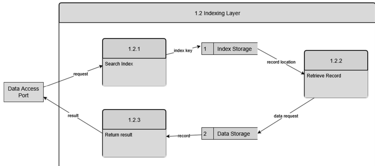
DFD Figure 1.14.0.0.2 – Indexed Data Lookup
