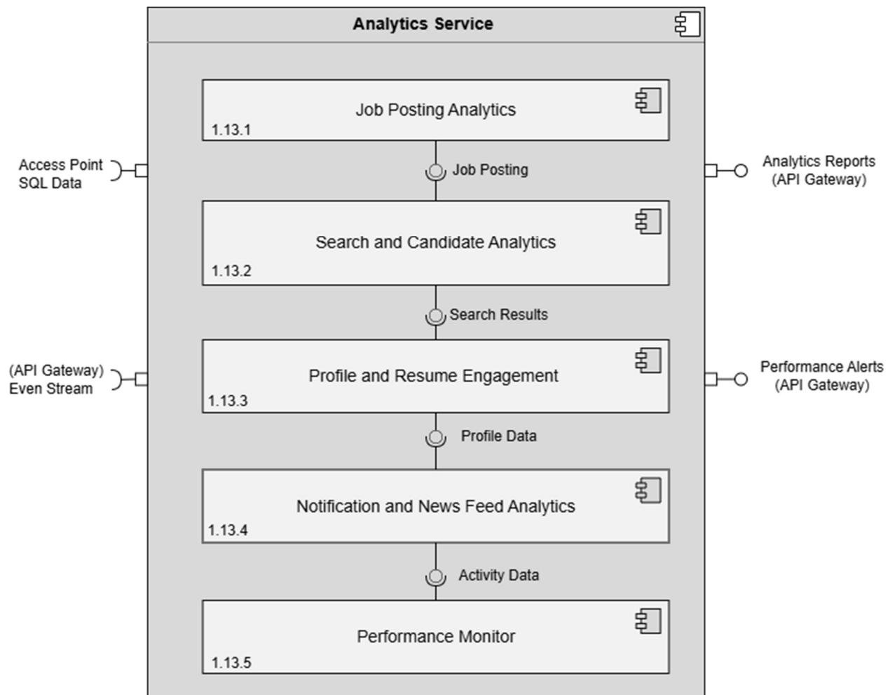
Figure 1.13 — Analytics Service Detail
