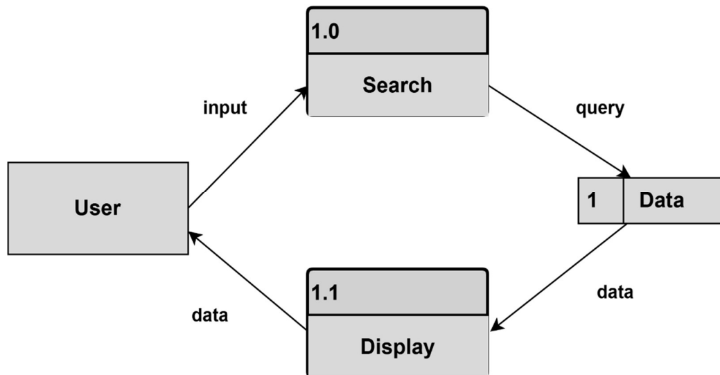
DFD Figure 1.9.0.0.2 – Company Search
