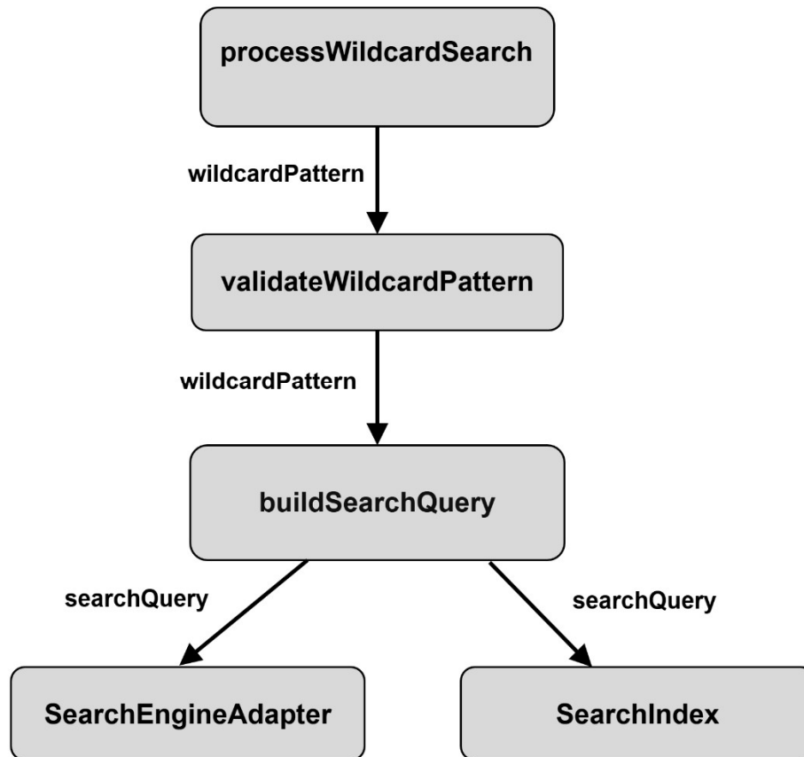
SC Figure 1.9.0.5 – processWildcardSearch()
