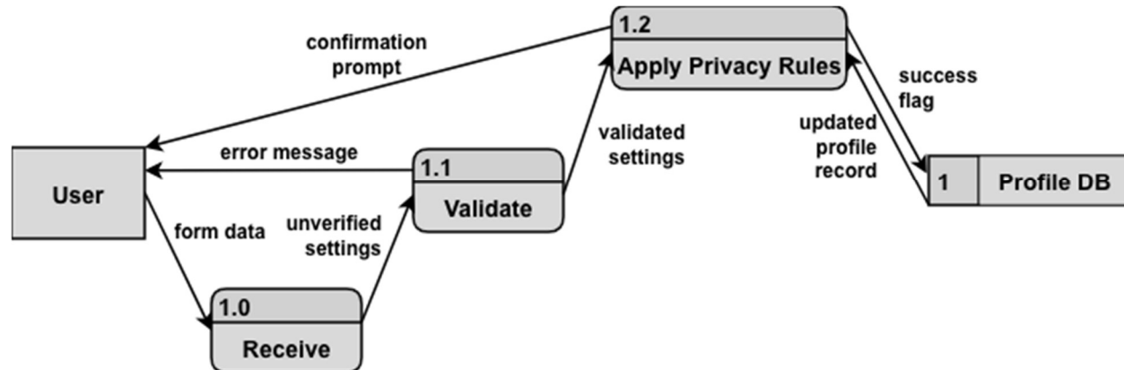
DFD Figure 1.6.0.0.2 — Privacy Settings Update
