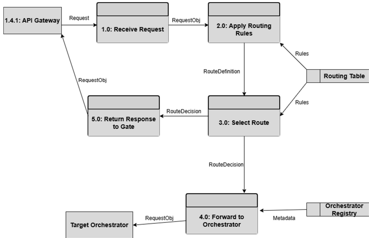
DFD Figure 1.4.0.0.3 – Request Routing
