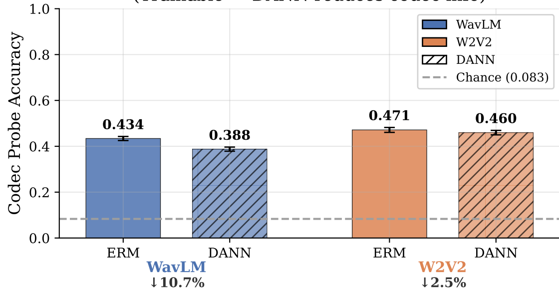
(b) Projection Layer Probes (WavLM & W2V2) (Trainable — DANN reduces codec info)
