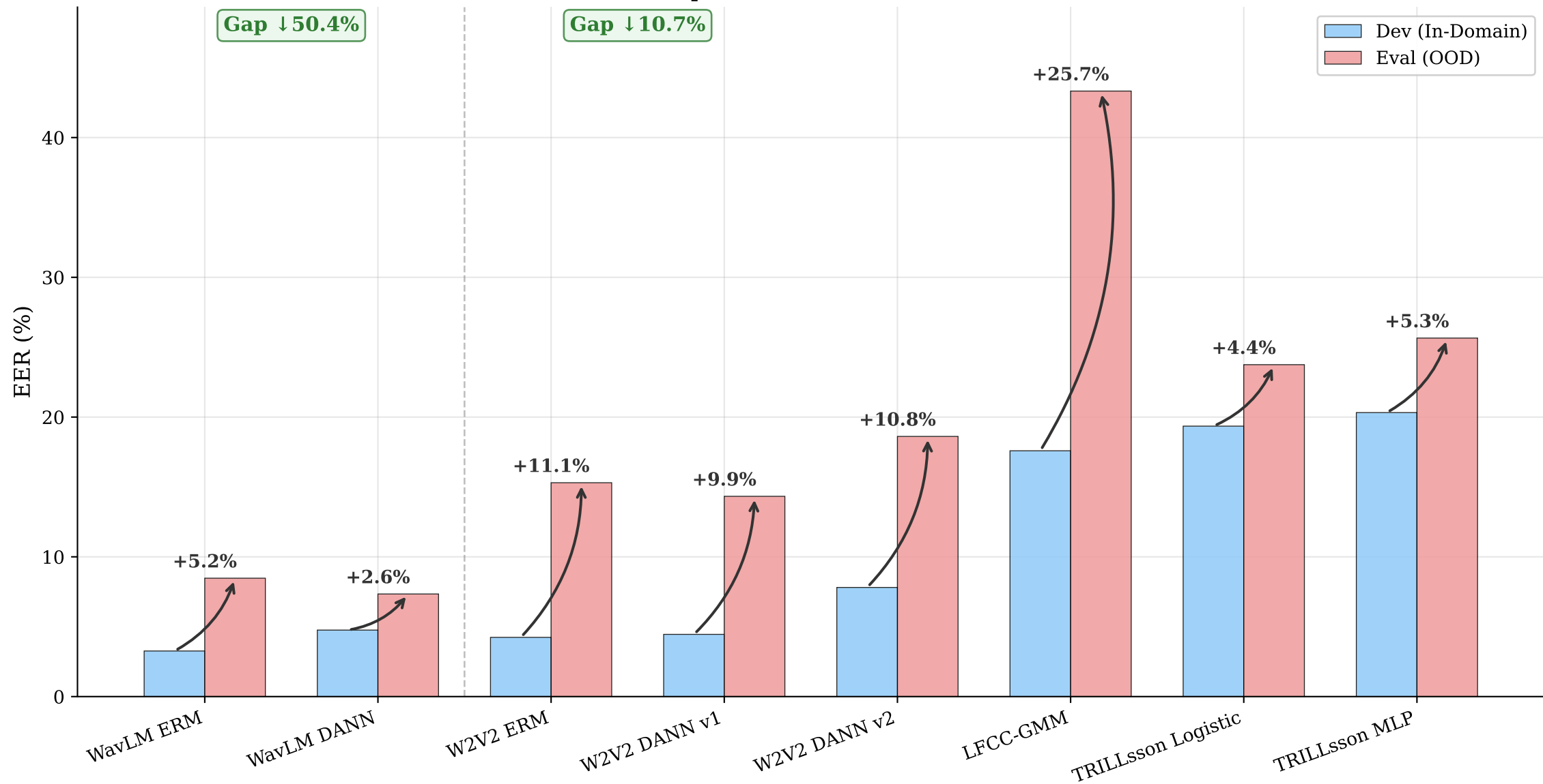
OOD Generalization Gap: Dev (In-Domain) vs Eval (Out-of-Domain)
