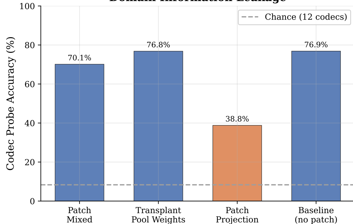
Domain Information Leakage
