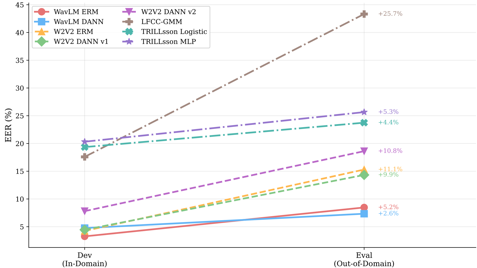
OOD Generalization: Dev \rightarrow Eval Transition
