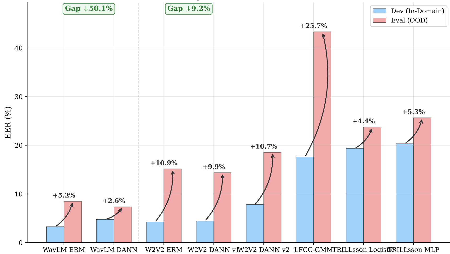
OOD Generalization Gap: Dev (In-Domain) vs Eval (Out-of-Domain)
