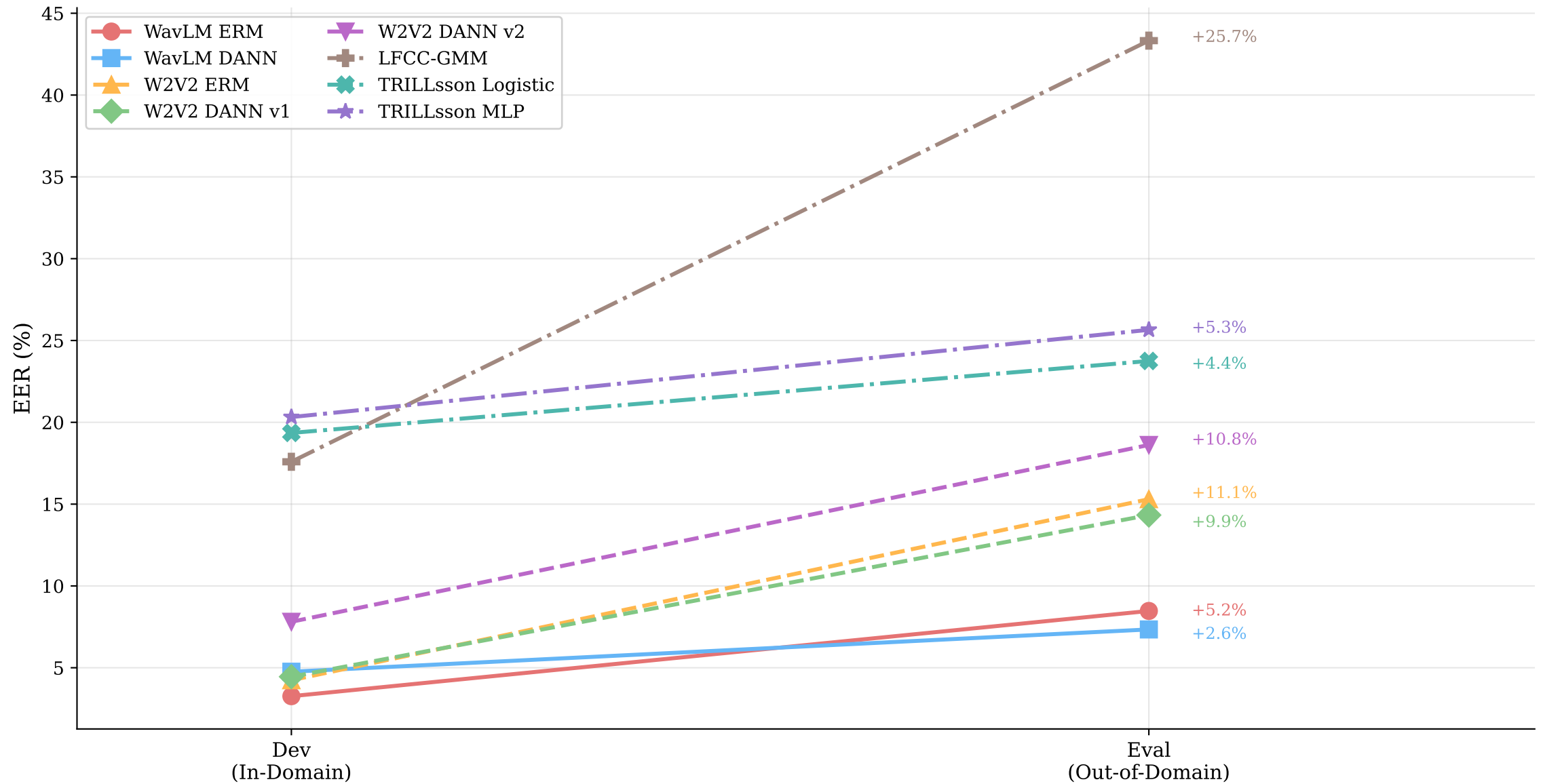
OOD Generalization: Dev → Eval Transition
