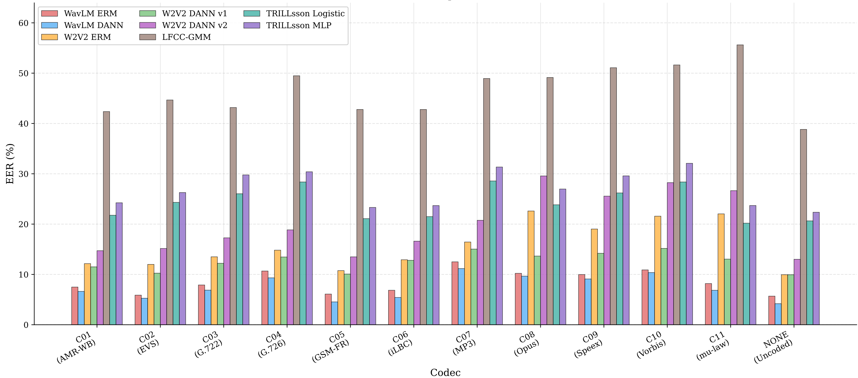
Per-Codec EER Comparison on Eval Set
