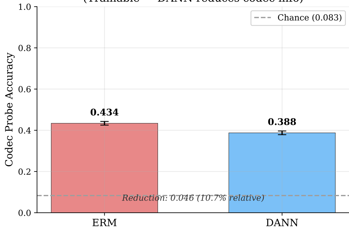
(b) Projection Layer Probes (WavLM & W2V2) (Trainable — DANN reduces codec info)
