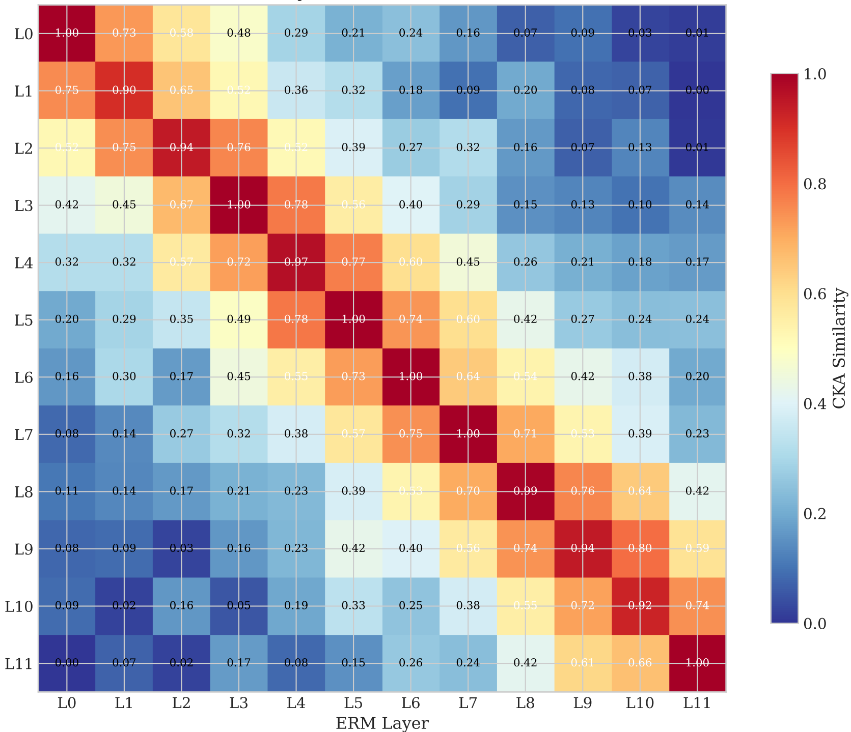
CKA Similarity: ERM vs DANN (Placeholder)
