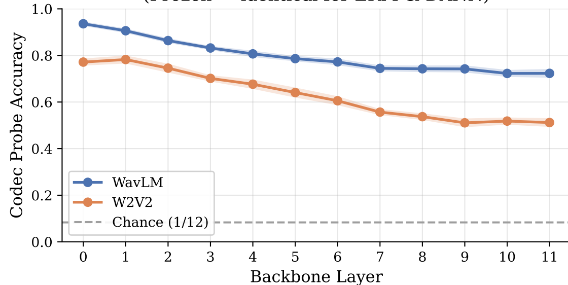
(a) Backbone Layer Probes (Frozen — identical for ERM & DANN)
