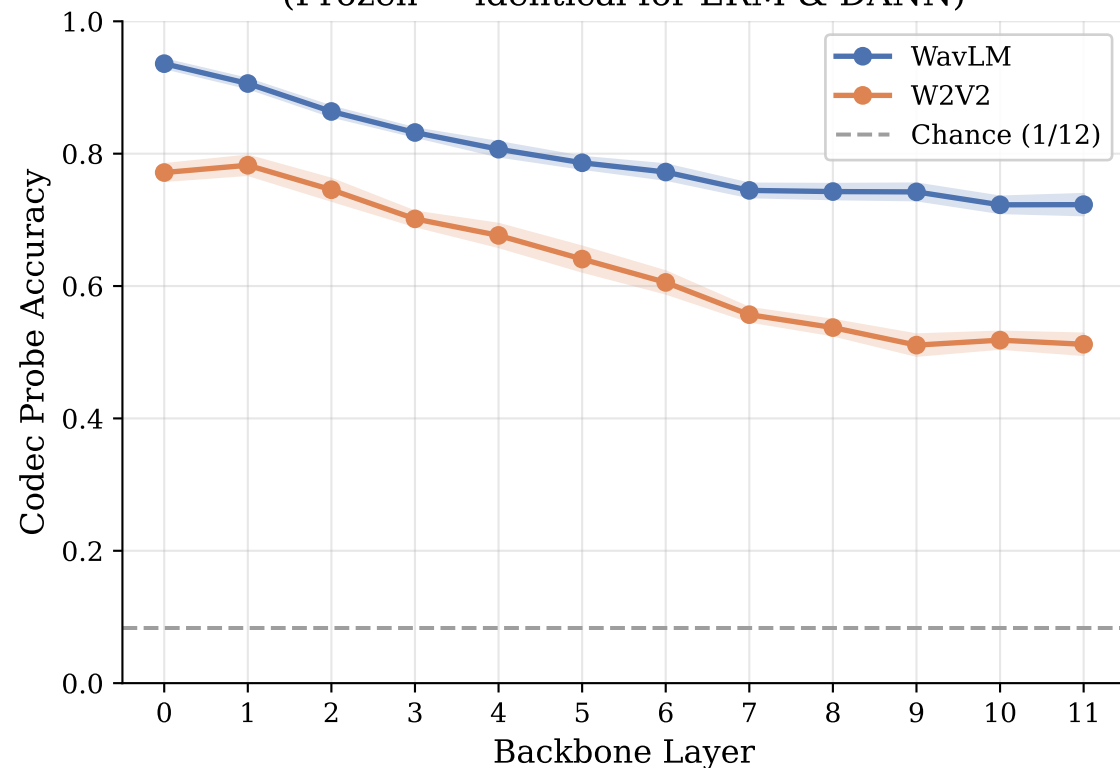
(a) Backbone Layer Probes (Frozen — identical for ERM & DANN)
