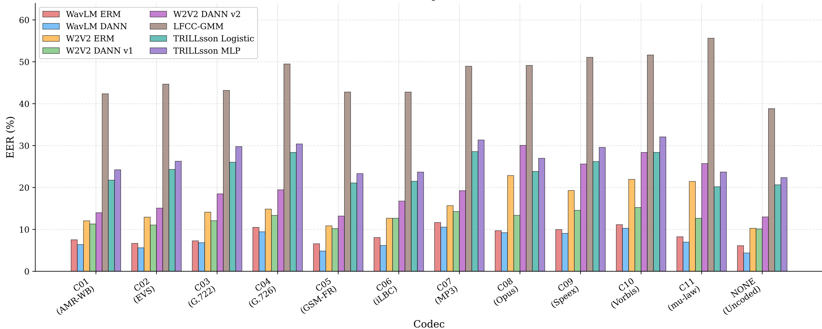
Per-Codec EER Comparison on Eval Set
