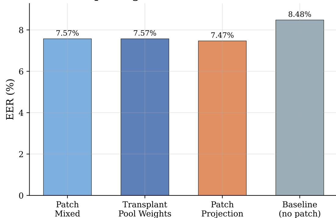
Spoofing Detection Performance
