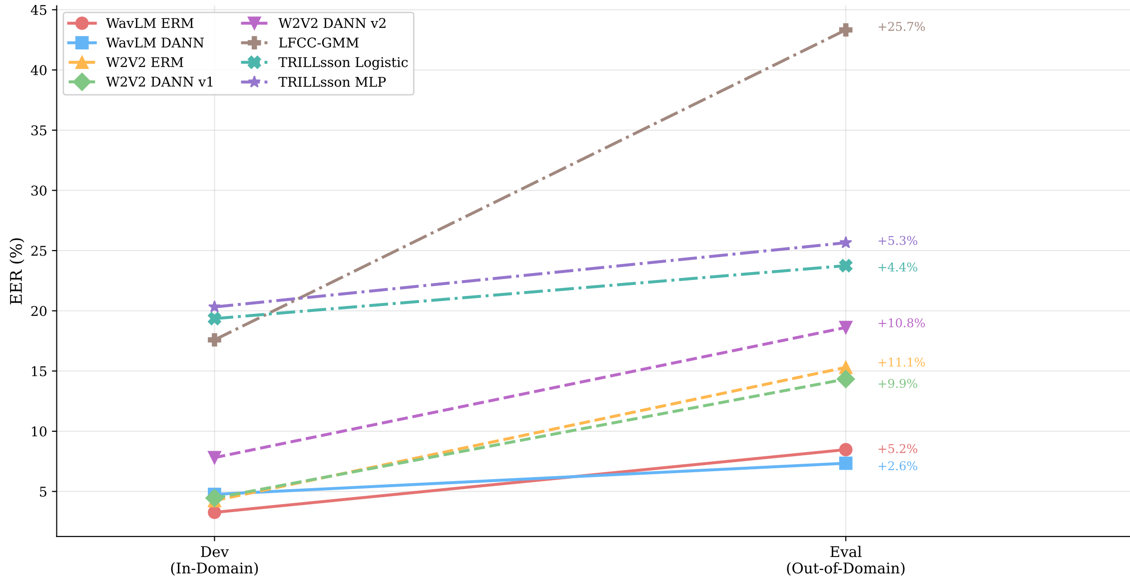
OOD Generalization: Dev \rightarrow Eval Transition
