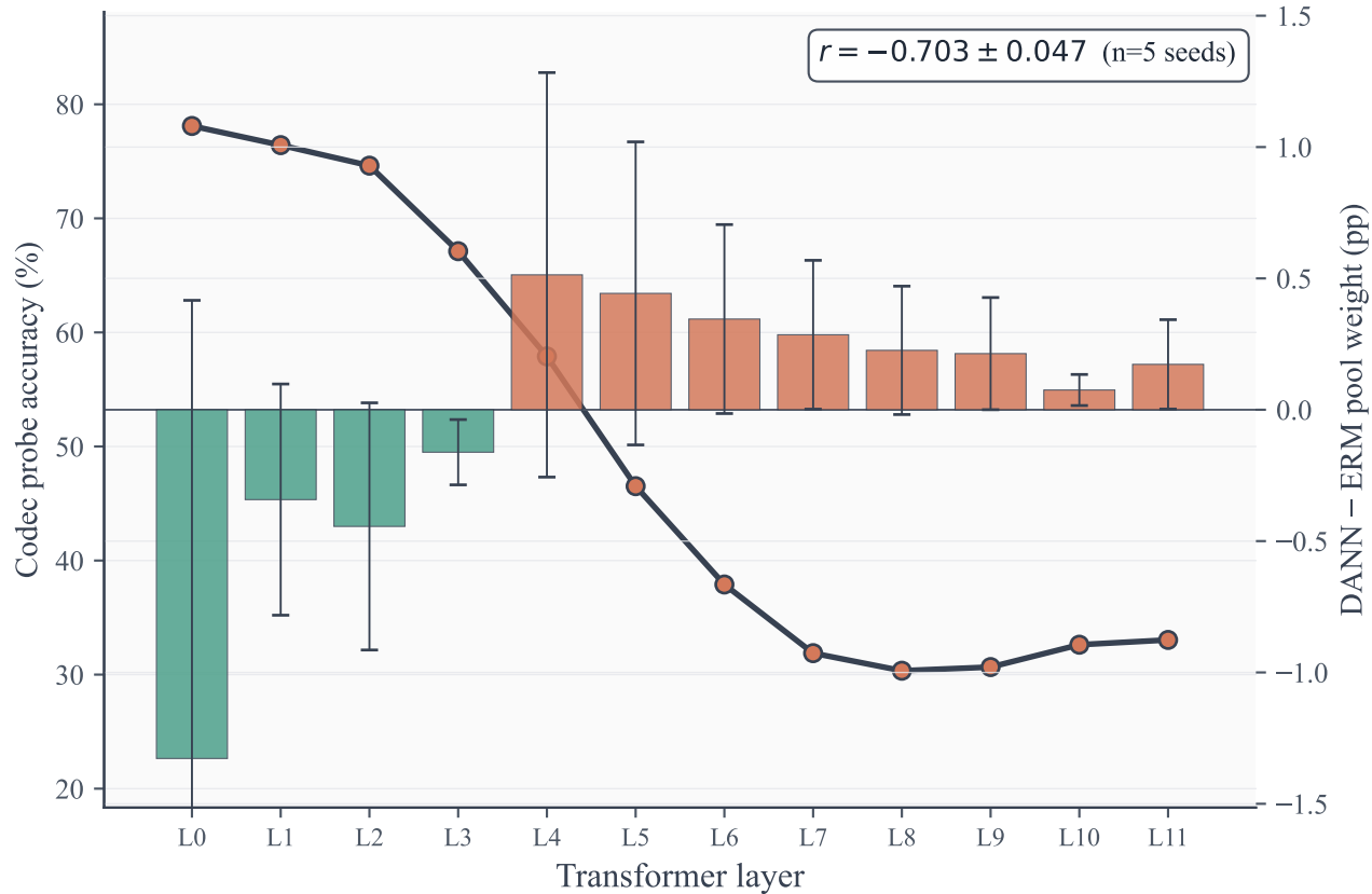
WavLM
