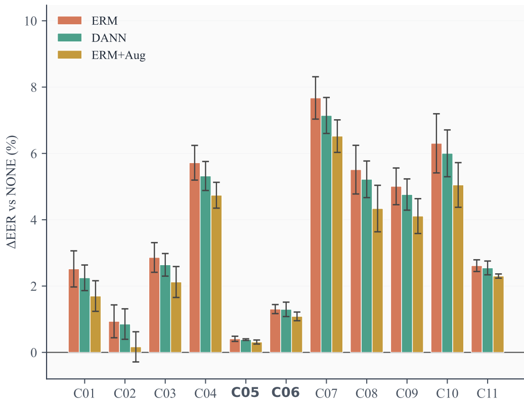
WavLM
