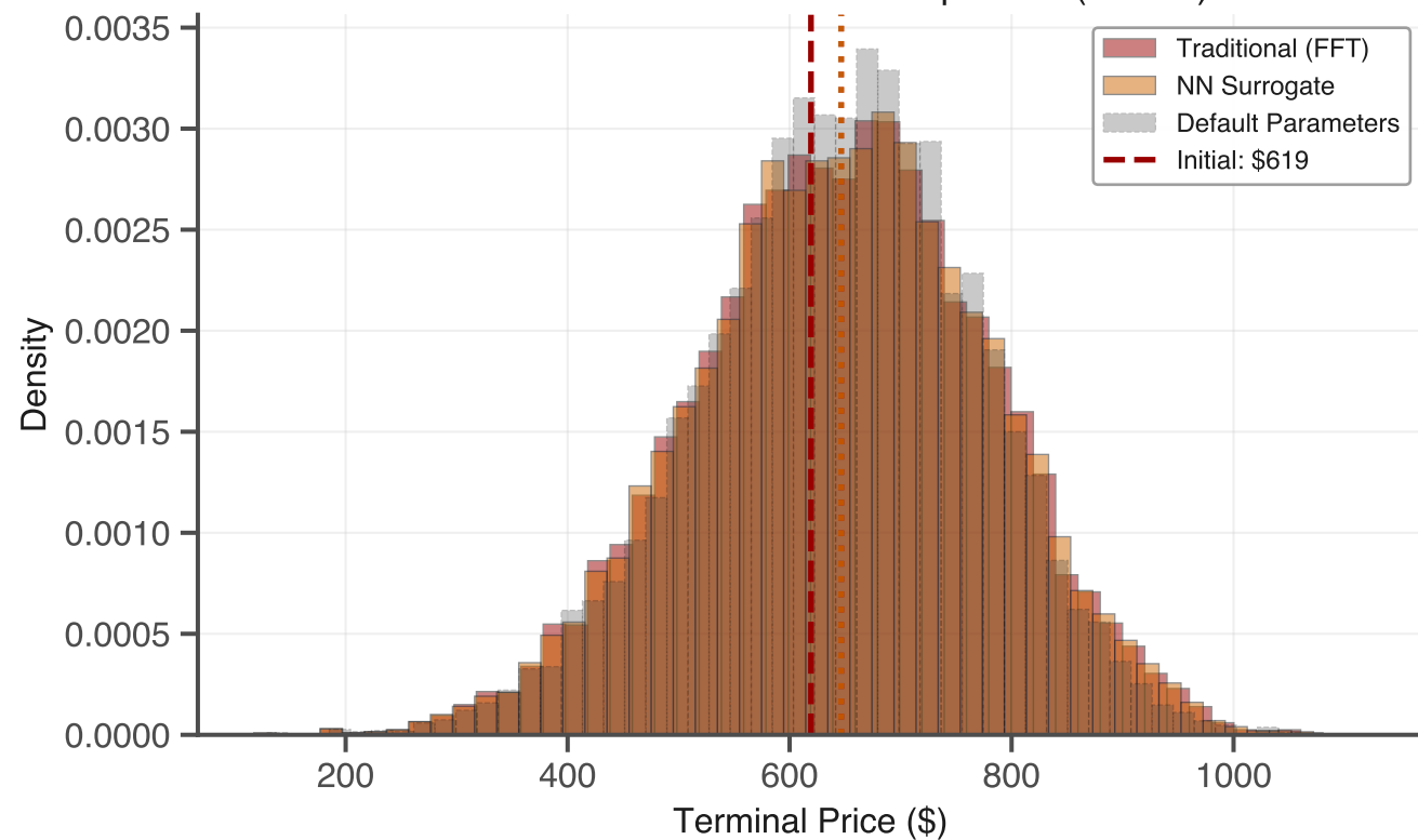
Terminal Price Distribution Comparison (1 Year)
